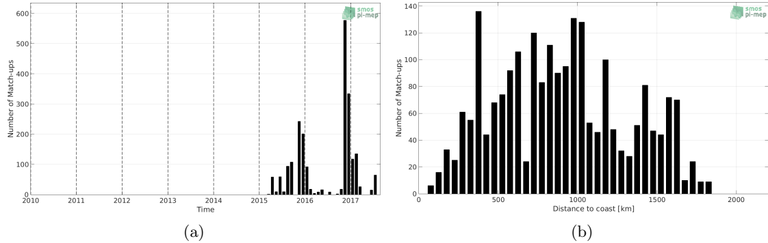
Figure 1: Number of match-ups between Sea mammals and SMAP-L3-RSS-V3-8DAY-RUNNING-70KM SSS as a function of time (a) and as function of the distance to coast (b) over the Roaring Forties and Furious Fifties Pi-MEP region and for the full satellite product period.
