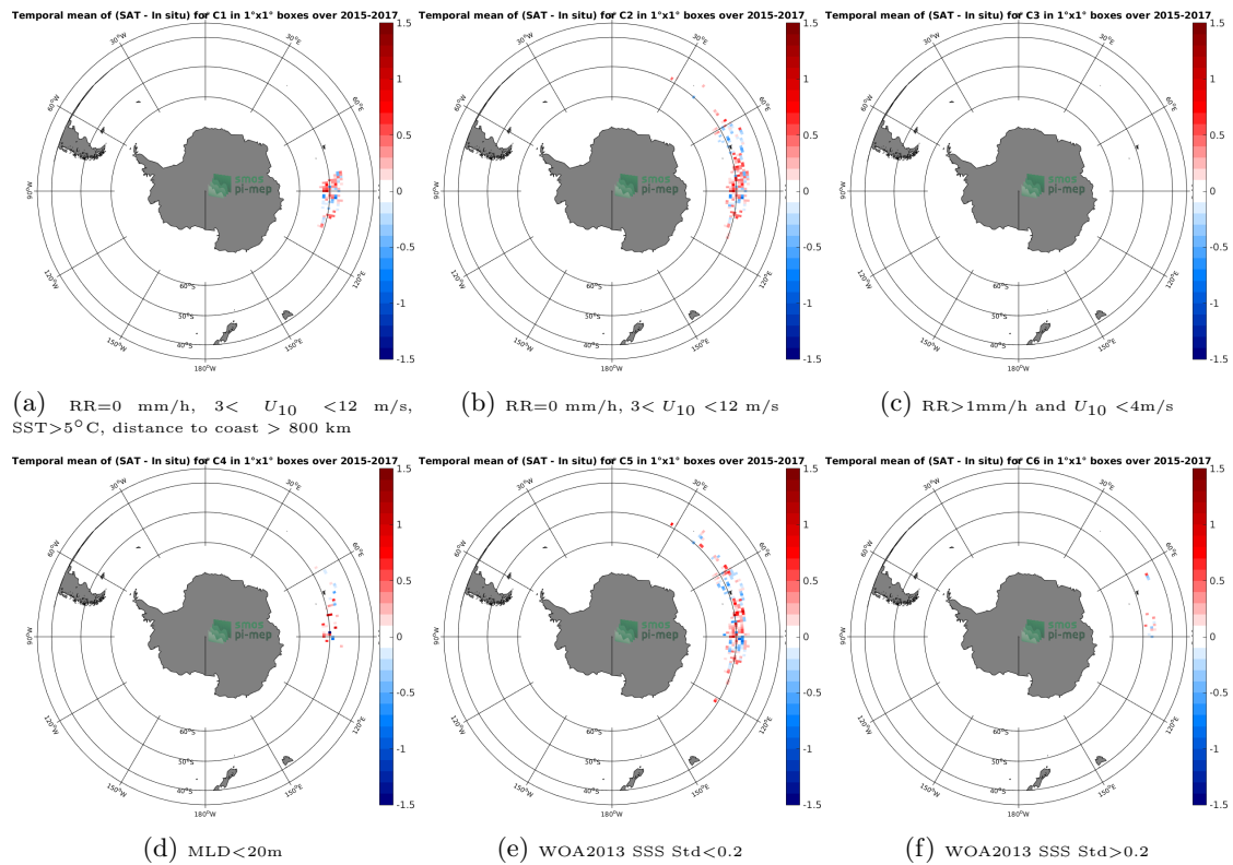
Figure 12: Temporal mean gridded over spatial boxes of size 1^\circ \times 1^\circ of \Delta SSS (SMAP-L3-RSS-V3-8DAY-RUNNING-70KM - Sea mammals) for 6 different subdatasets corresponding to:RR=0 mm/h, 3 < U_{10} < 12 m/s, SST > 5^\circ\text{C} , distance to coast > 800 km (a), RR=0 mm/h, 3 < U_{10} < 12 m/s (b), RR > 1 mm/h and U_{10} < 4 m/s (c),MLD < 20 m (d),WOA2013 SSS Std < 0.2 (e),WOA2013 SSS Std > 0.2 (f).
