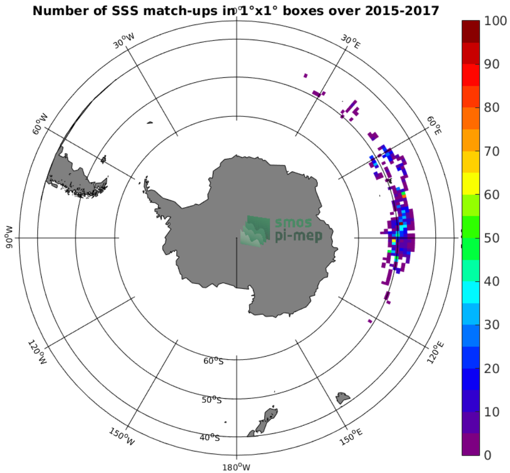
Figure 4: Number of SSS match-ups between Sea mammals SSS and the SMAP-L3-RSS-V3-8DAY-RUNNING-70KM SSS product for the Roaring Forties and Furious Fifties Pi-MEP region over 1°x1° boxes and for the full satellite product period.
