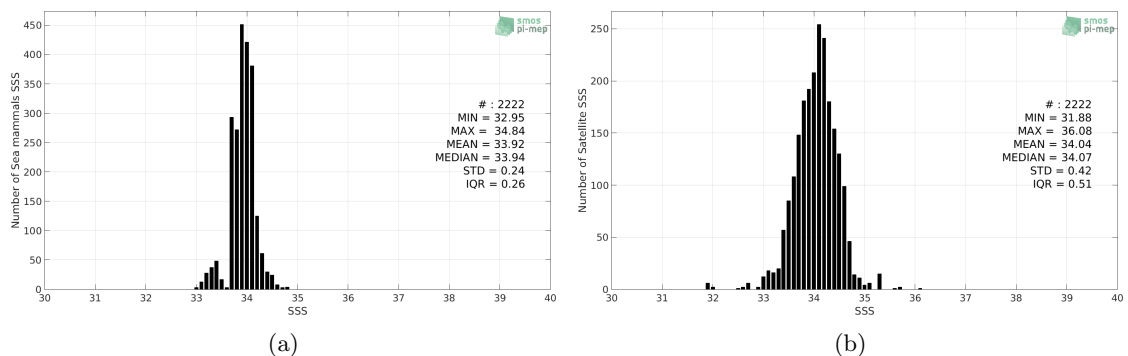
Figure 2: Histograms of SSS from Sea mammals (a) and SMAP-L3-RSS-V3-8DAY-RUNNING-70KM (b) considering all match-up pairs per bins of 0.1 over the Roaring Forties and Furious Fifties Pi-MEP region and for the full satellite product period.
