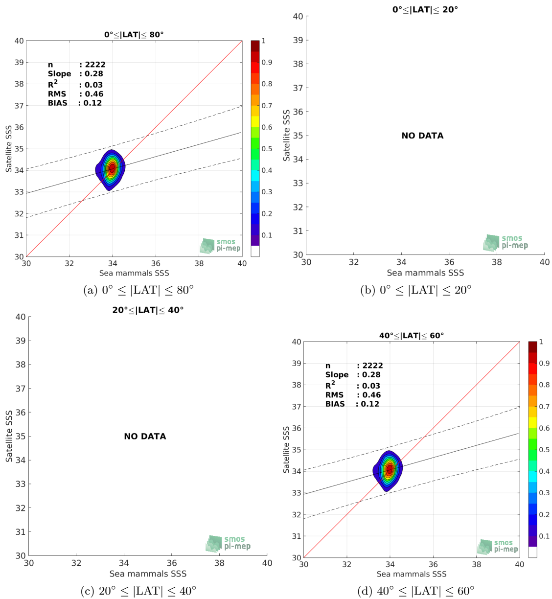
Figure 9: Contour maps of the concentration of SMAP-L3-RSS-V3-8DAY-RUNNING-70KM SSS (y-axis) versus Sea mammals SSS (x-axis) at match-up pairs for different latitude bands. For each plot, the red line shows x=y . The black thin and dashed lines indicate a linear fit through the data cloud and the \pm 95\% confidence levels, respectively. The number match-up pairs n , the slope and R^2 coefficient of the linear fit, the root mean square (RMS) and the mean bias between satellite and in situ data are indicated for each latitude band in each plots.
