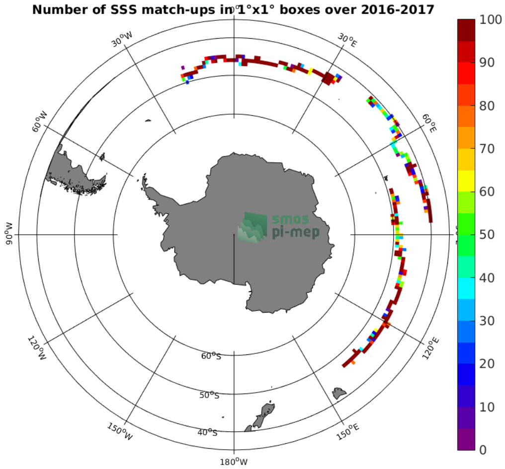
Figure 3: Number of SSS match-ups between Surface drifters SSS and the SMAP-L3-RSS-V3-8DAY-RUNNING-70KM SSS product for the Roaring Forties and Furious Fifties Pi-MEP region over 1°x1° boxes and for the full satellite product period.
