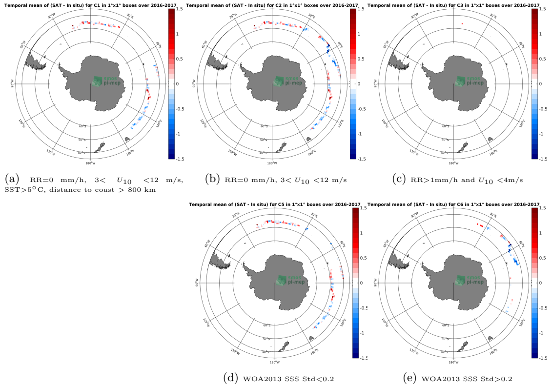
Figure 11: Temporal mean gridded over spatial boxes of size 1^\circ \times 1^\circ of \Delta SSS (SMAP-L3-RSS-V3-8DAY-RUNNING-70KM - Surface drifters) for 5 different subdatasets corresponding to:RR=0 mm/h, 3 < U_{10} < 12 m/s, SST >5^\circ C, distance to coast > 800 km (a), RR=0 mm/h, 3 < U_{10} < 12 m/s (b), RR >1 mm/h and U_{10} < 4 m/s (c), WOA2013 SSS Std <0.2 (d), WOA2013 SSS Std >0.2 (e).
