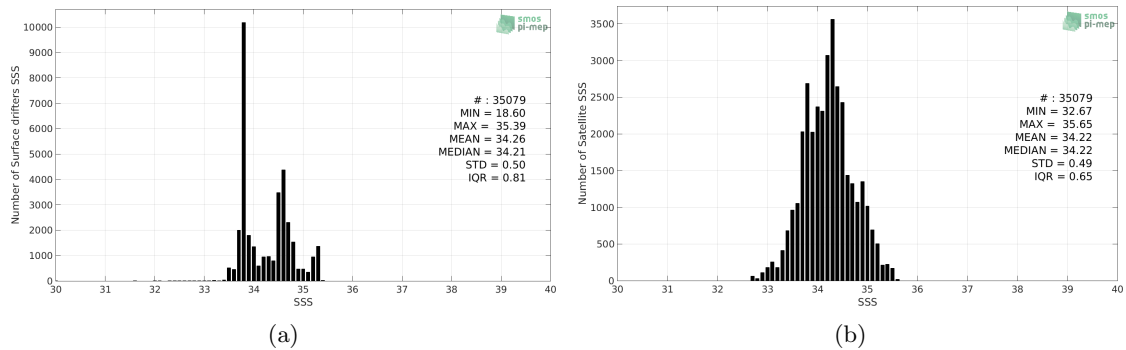
Figure 2: Histograms of SSS from Surface drifters (a) and SMAP-L3-RSS-V3-8DAY-RUNNING-70KM (b) considering all match-up pairs per bins of 0.1 over the Roaring Forties and Furious Fifties Pi-MEP region and for the full satellite product period.
