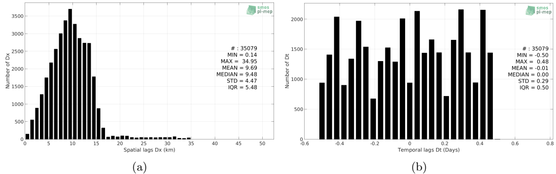
Figure 4: Histograms of the spatial (a) and temporal (b) lags between the time of the Surface drifters measurements and the date of the corresponding SMAP-L3-RSS-V3-8DAY-RUNNING-70KM SSS product.
