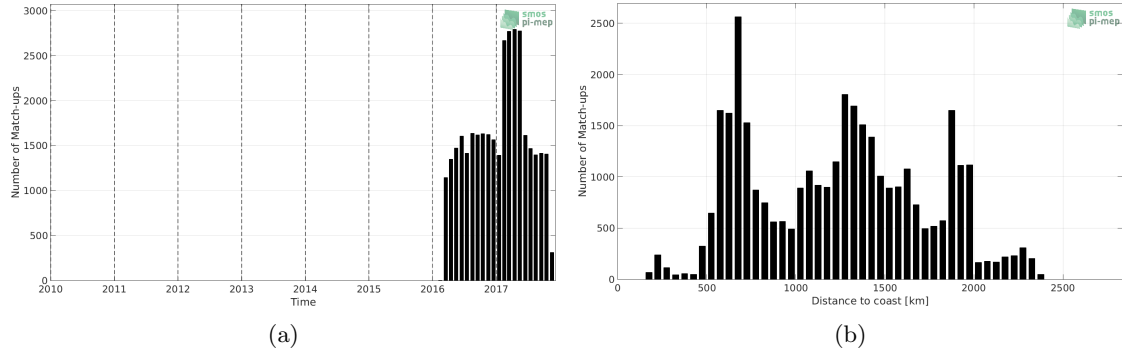
Figure 1: Number of match-ups between Surface drifters and SMAP-L3-RSS-V3-8DAY-RUNNING-70KM SSS as a function of time (a) and as function of the distance to coast (b) over the Roaring Forties and Furious Fifties Pi-MEP region and for the full satellite product period.
