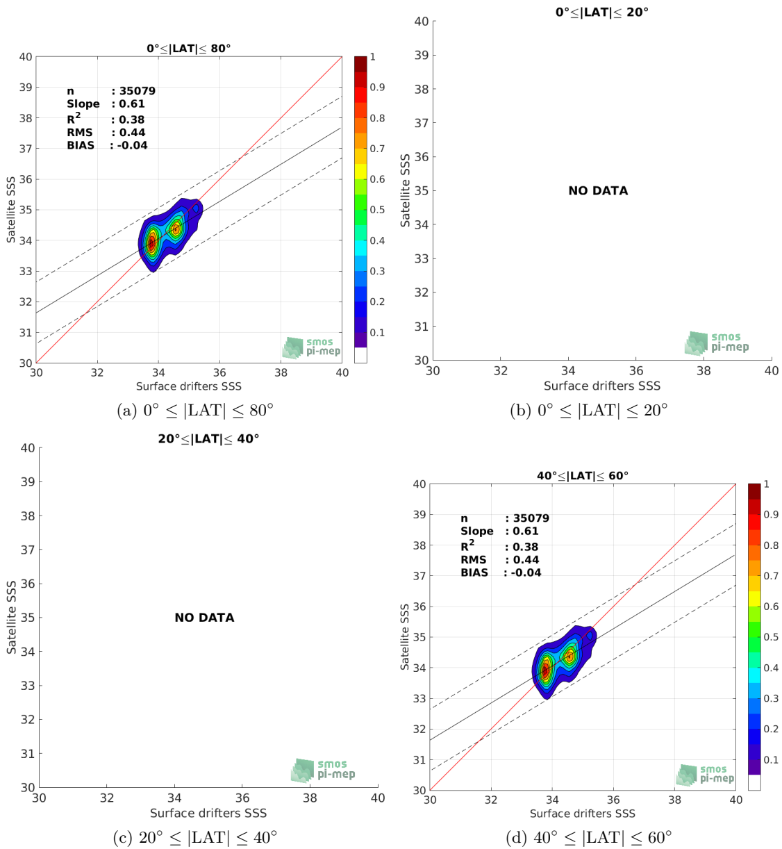
Figure 8: Contour maps of the concentration of SMAP-L3-RSS-V3-8DAY-RUNNING-70KM SSS (y-axis) versus Surface drifters SSS (x-axis) at match-up pairs for different latitude bands. For each plot, the red line shows x=y . The black thin and dashed lines indicate a linear fit through the data cloud and the \pm 95\% confidence levels, respectively. The number match-up pairs n , the slope and R^2 coefficient of the linear fit, the root mean square (RMS) and the mean bias between satellite and in situ data are indicated for each latitude band in each plots.
