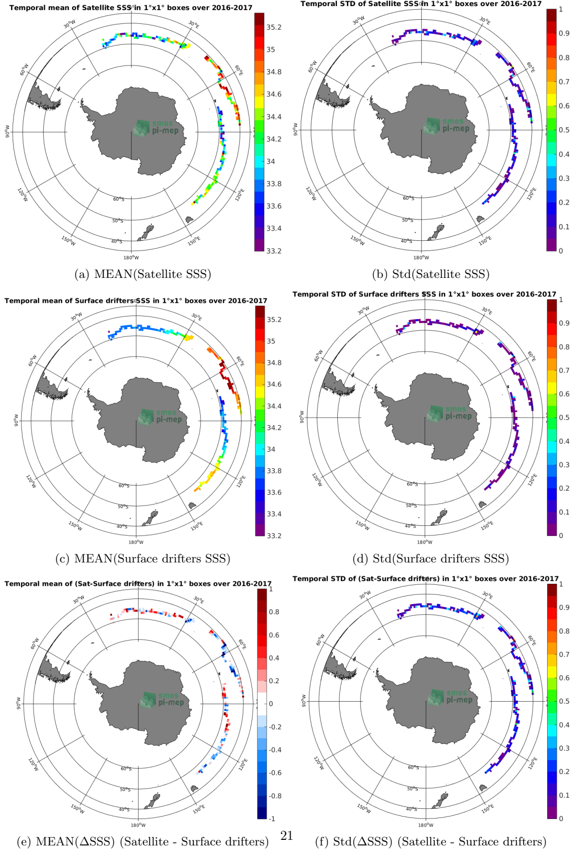
Figure 5: Temporal mean (left) and Std (right) of SSS from SMAP-L3-RSS-V3-8DAY-RUNNING-70KM (top), Surface drifters (middle), and of \Delta SSS (Satellite - Surface drifters). Only match-up pairs are used to generate these maps.
