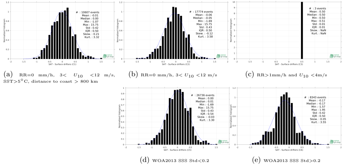
Figure 12: Normalized histogram of \Delta SSS (SMAP-L3-RSS-V3-8DAY-RUNNING-70KM - Surface drifters) for 5 different subdatasets corresponding to: RR=0 mm/h, 3 < U_{10} < 12 m/s, SST > 5°C, distance to coast > 800 km (a), RR=0 mm/h, 3 < U_{10} < 12 m/s (b), RR > 1mm/h and U_{10} < 4 m/s (c), WOA2013 SSS Std < 0.2 (d), WOA2013 SSS Std > 0.2 (e).
