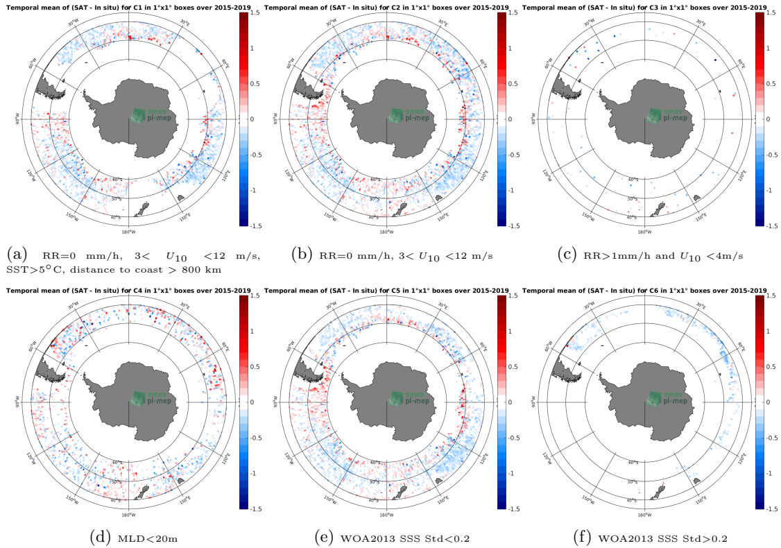
Figure 12: Temporal mean gridded over spatial boxes of size 1^\circ \times 1^\circ of \Delta SSS (SMAP-L3-RSS-V3-8DAY-RUNNING-70KM - Argo) for 6 different subdatasets corresponding to:RR=0 mm/h, 3 < U_{10} < 12 m/s, SST >5^\circ C, distance to coast > 800 km (a), RR=0 mm/h, 3 < U_{10} < 12 m/s (b), RR >1 mm/h and U_{10} < 4 m/s (c),MLD <20 m (d),WOA2013 SSS Std <0.2 (e),WOA2013 SSS Std >0.2 (f).
