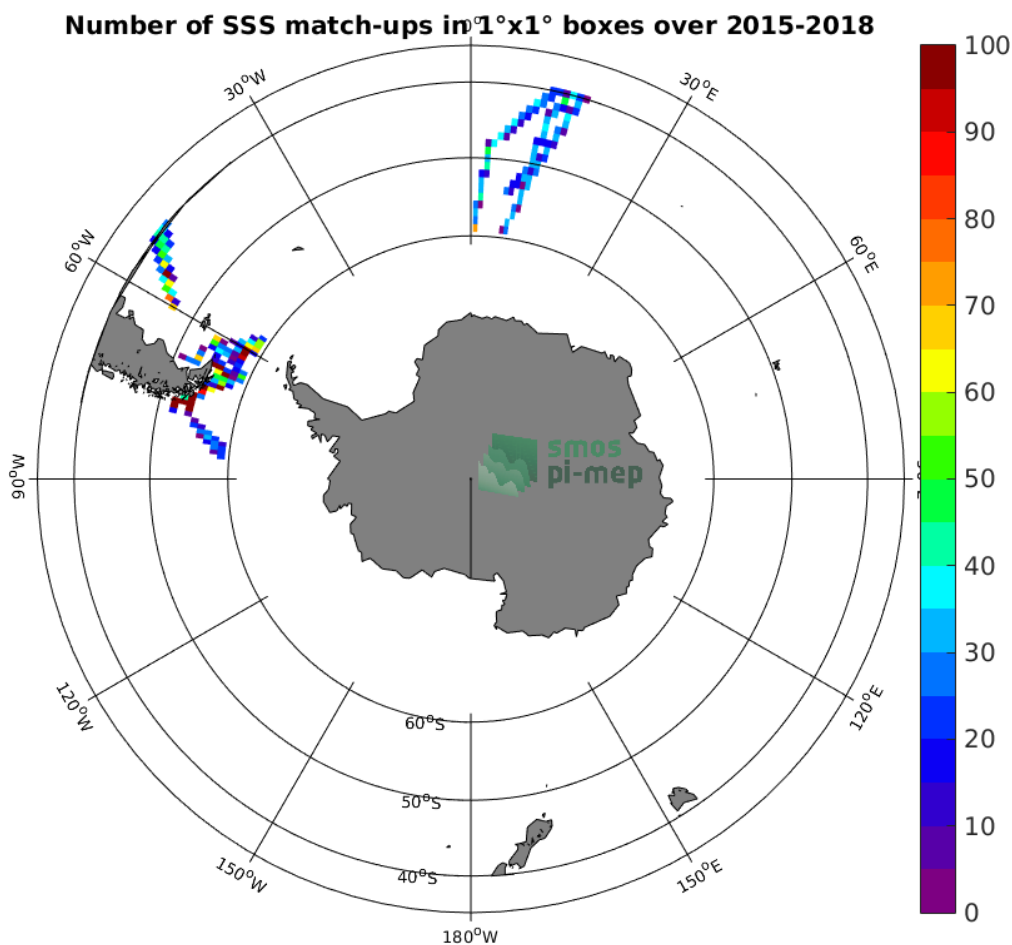
Figure 4: Number of SSS match-ups between TSG-POLARSTERN SSS and the SMAP-L3-RSS-V3-8DAY-RUNNING-40KM SSS product for the Roaring Forties and Furious Fifties Pi-MEP region over 1°x1° boxes and for the full satellite product period.
