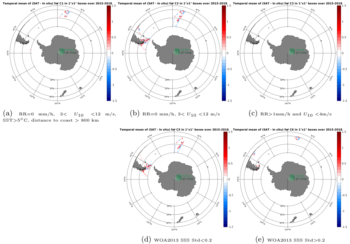
Figure 12: Temporal mean gridded over spatial boxes of size 1^\circ \times 1^\circ of \Delta SSS (SMAP-L3-RSS-V3-8DAY-RUNNING-40KM - TSG-POLARSTERN) for 5 different subdatasets corresponding to: RR=0 mm/h, 3 < U_{10} < 12 m/s, SST > 5^\circ\text{C} , distance to coast > 800 km (a), RR=0 mm/h, 3 < U_{10} < 12 m/s (b), RR > 1 mm/h and U_{10} < 4 m/s (c), WOA2013 SSS Std < 0.2 (d), WOA2013 SSS Std > 0.2 (e).
