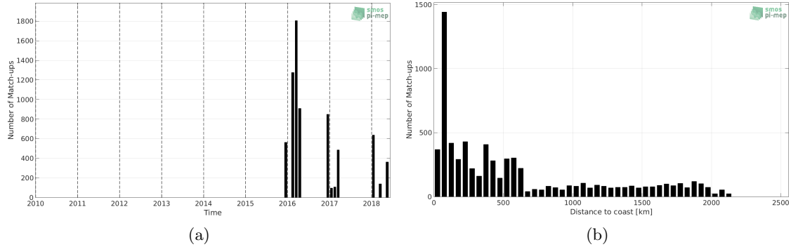
Figure 1: Number of match-ups between TSG-POLARSTERN and SMAP-L3-RSS-V3-8DAY-RUNNING-40KM SSS as a function of time (a) and as function of the distance to coast (b) over the Roaring Forties and Furious Fifties Pi-MEP region and for the full satellite product period.
