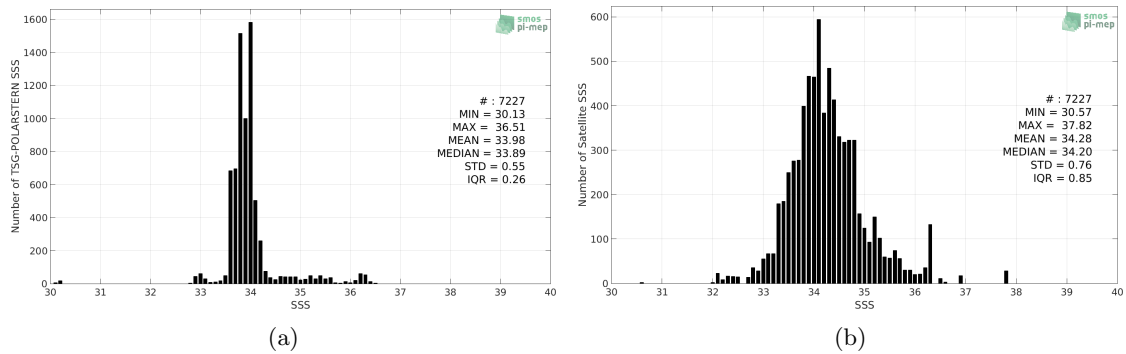
Figure 2: Histograms of SSS from TSG-POLARSTERN (a) and SMAP-L3-RSS-V3-8DAY-RUNNING-40KM (b) considering all match-up pairs per bins of 0.1 over the Roaring Forties and Furious Fifties Pi-MEP region and for the full satellite product period.
