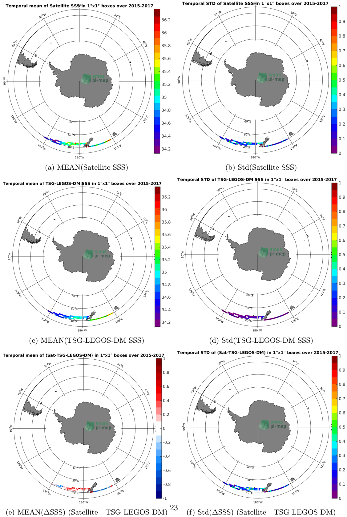
Figure 6: Temporal mean (left) and Std (right) of SSS from SMAP-L3-RSS-V3-8DAY-RUNNING-40KM (top), TSG-LEGOS-DM (middle), and of \Delta SSS (Satellite - TSG-LEGOS-DM). Only match-up pairs are used to generate these maps.
