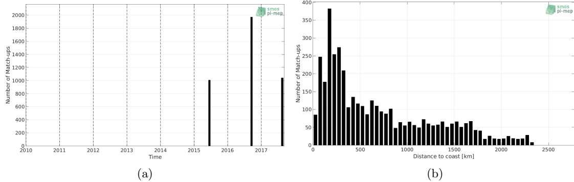
Figure 1: Number of match-ups between TSG-LEGOS-DM and SMAP-L3-RSS-V3-8DAY-RUNNING-40KM SSS as a function of time (a) and as function of the distance to coast (b) over the Roaring Forties and Furious Fifties Pi-MEP region and for the full satellite product period.
