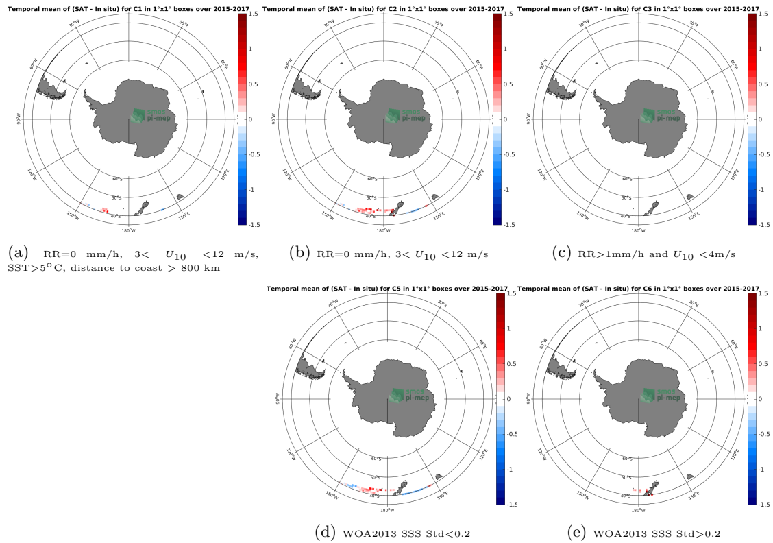
Figure 12: Temporal mean gridded over spatial boxes of size 1^\circ \times 1^\circ of \Delta SSS (SMAP-L3-RSS-V3-8DAY-RUNNING-40KM - TSG-LEGOS-DM) for 5 different subdatasets corresponding to:RR=0 mm/h, 3 < U_{10} < 12 m/s, SST > 5^\circ\text{C} , distance to coast > 800 km (a), RR=0 mm/h, 3 < U_{10} < 12 m/s (b), RR > 1 mm/h and U_{10} < 4 m/s (c), WOA2013 SSS Std < 0.2 (d), WOA2013 SSS Std > 0.2 (e).
