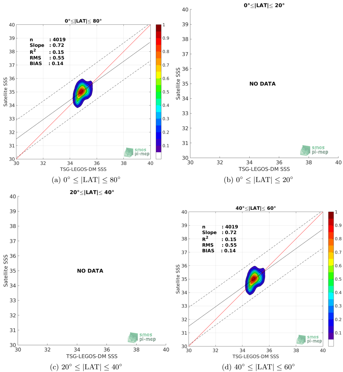
Figure 9: Contour maps of the concentration of SMAP-L3-RSS-V3-8DAY-RUNNING-40KM SSS (y-axis) versus TSG-LEGOS-DM SSS (x-axis) at match-up pairs for different latitude bands. For each plot, the red line shows x=y . The black thin and dashed lines indicate a linear fit through the data cloud and the \pm 95\% confidence levels, respectively. The number match-up pairs n , the slope and R^2 coefficient of the linear fit, the root mean square (RMS) and the mean bias between satellite and in situ data are indicated for each latitude band in each plots.
