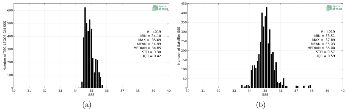
Figure 2: Histograms of SSS from TSG-LEGOS-DM (a) and SMAP-L3-RSS-V3-8DAY-RUNNING-40KM (b) considering all match-up pairs per bins of 0.1 over the Roaring Forties and Furious Fifties Pi-MEP region and for the full satellite product period.
