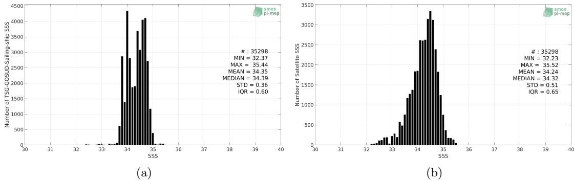
Figure 2: Histograms of SSS from TSG-GOSUD-Sailing-ship (a) and SMAP-L3-RSS-V3-8DAY-RUNNING-40KM (b) considering all match-up pairs per bins of 0.1 over the Roaring Forties and Furious Fifties Pi-MEP region and for the full satellite product period.
