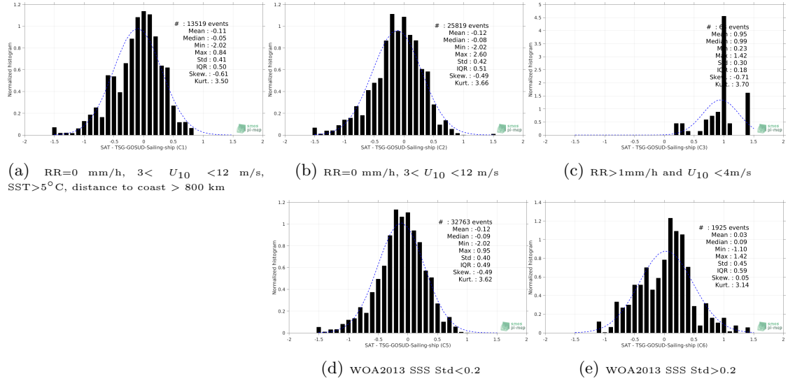
Figure 13: Normalized histogram of \Delta\text{SSS} (SMAP-L3-RSS-V3-8DAY-RUNNING-40KM - TSG-GOSUD-Sailing-ship) for 5 different subdatasets corresponding to: RR=0 mm/h, 3 < U_{10} < 12 m/s, SST >5^{\circ}\text{C} , distance to coast > 800 km (a), RR=0 mm/h, 3 < U_{10} < 12 m/s (b), RR >1 mm/h and U_{10} < 4 m/s (c), WOA2013 SSS Std <0.2 (d), WOA2013 SSS Std >0.2 (e).
