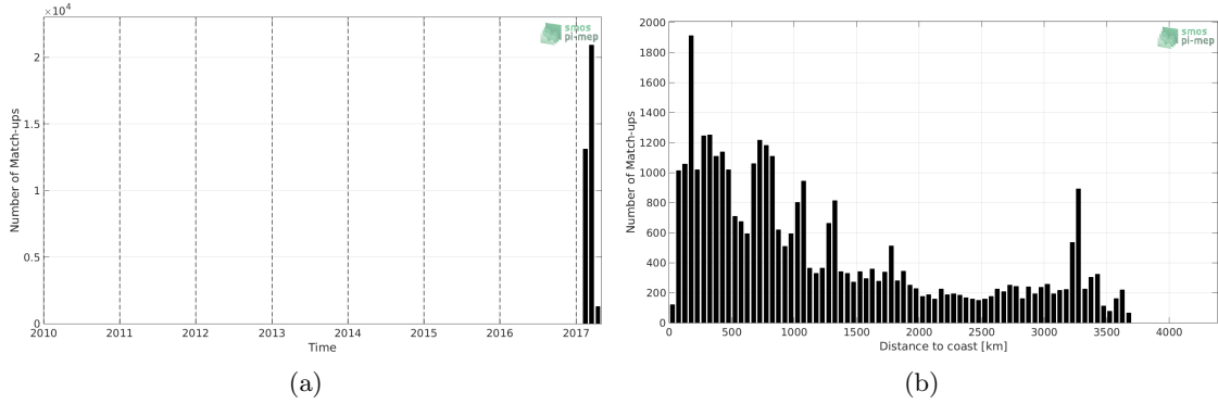
Figure 1: Number of match-ups between TSG-GOSUD-Sailing-ship and SMAP-L3-RSS-V3-8DAY-RUNNING-40KM SSS as a function of time (a) and as function of the distance to coast (b) over the Roaring Forties and Furious Fifties Pi-MEP region and for the full satellite product period.
