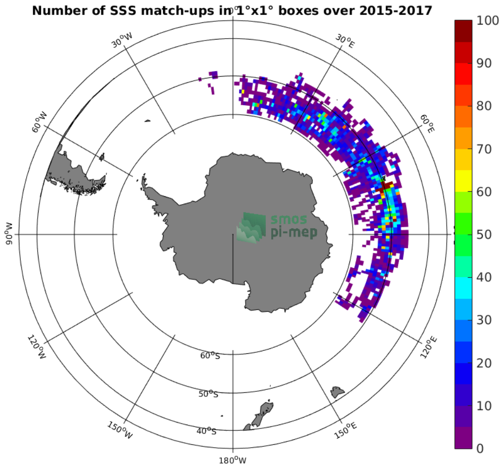
Figure 4: Number of SSS match-ups between Sea mammals SSS and the SMAP-L3-RSS-V3-8DAY-RUNNING-40KM SSS product for the Roaring Forties and Furious Fifties Pi-MEP region over 1°x1° boxes and for the full satellite product period.
