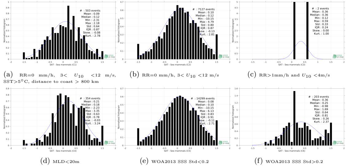
Figure 13: Normalized histogram of \Delta\text{SSS} (SMAP-L3-RSS-V3-8DAY-RUNNING-40KM - Sea mammals) for 6 different subdatasets corresponding to: RR=0 mm/h, 3 < U_{10} < 12 m/s, SST>5°C, distance to coast > 800 km (a), RR=0 mm/h, 3 < U_{10} < 12 m/s (b), RR>1mm/h and U_{10} < 4 m/s (c), MLD<20m (d), WOA2013 SSS Std<0.2 (e), WOA2013 SSS Std>0.2 (f).
