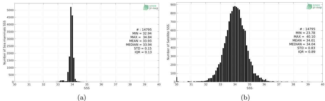
Figure 2: Histograms of SSS from Sea mammals (a) and SMAP-L3-RSS-V3-8DAY-RUNNING-40KM (b) considering all match-up pairs per bins of 0.1 over the Roaring Forties and Furious Fifties Pi-MEP region and for the full satellite product period.
