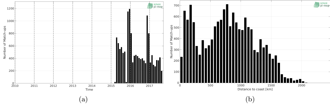
Figure 1: Number of match-ups between Sea mammals and SMAP-L3-RSS-V3-8DAY-RUNNING-40KM SSS as a function of time (a) and as function of the distance to coast (b) over the Roaring Forties and Furious Fifties Pi-MEP region and for the full satellite product period.
