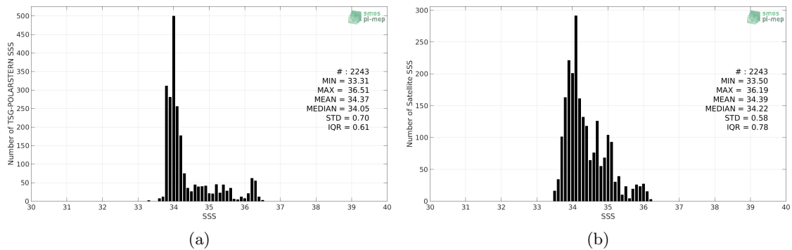
Figure 2: Histograms of SSS from TSG-POLARSTERN (a) and SMAP-L3-RSS-V3-MONTHLY-70KM (b) considering all match-up pairs per bins of 0.1 over the Roaring Forties and Furious Fifties Pi-MEP region and for the full satellite product period.
