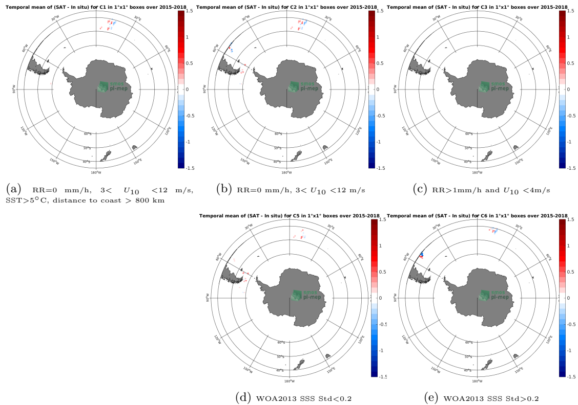
Figure 12: Temporal mean gridded over spatial boxes of size 1^\circ \times 1^\circ of \Delta SSS (SMAP-L3-RSS-V3-MONTHLY-70KM - TSG-POLARSTERN) for 5 different subdatasets corresponding to:RR=0 mm/h, 3 < U_{10} < 12 m/s, SST >5^\circ C, distance to coast > 800 km (a), RR=0 mm/h, 3 < U_{10} < 12 m/s (b), RR >1 mm/h and U_{10} < 4 m/s (c), WOA2013 SSS Std <0.2 (d), WOA2013 SSS Std >0.2 (e).
