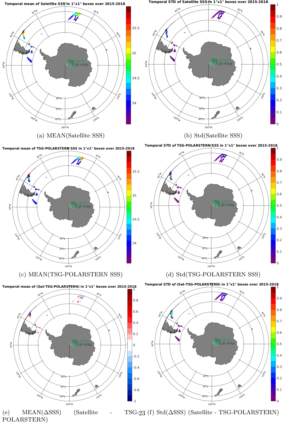
Figure 6: Temporal mean (left) and Std (right) of SSS from SMAP-L3-RSS-V3-MONTHLY-70KM (top), TSG-POLARSTERN (middle), and of \Delta SSS (Satellite - TSG-POLARSTERN). Only match-up pairs are used to generate these maps.
