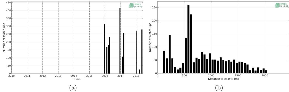
Figure 1: Number of match-ups between TSG-POLARSTERN and SMAP-L3-RSS-V3-MONTHLY-70KM SSS as a function of time (a) and as function of the distance to coast (b) over the Roaring Forties and Furious Fifties Pi-MEP region and for the full satellite product period.
