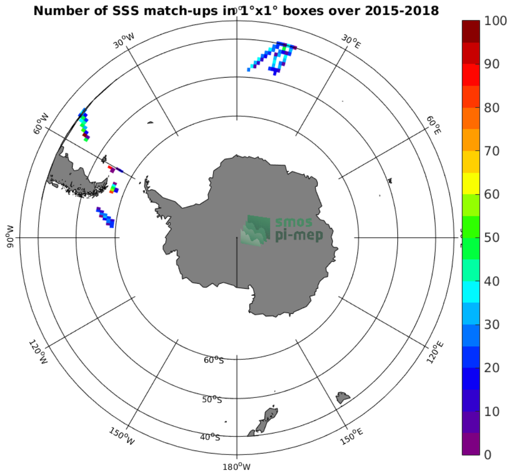
Figure 4: Number of SSS match-ups between TSG-POLARSTERN SSS and the SMAP-L3-RSS-V3-MONTHLY-70KM SSS product for the Roaring Forties and Furious Fifties Pi-MEP region over 1°x1° boxes and for the full satellite product period.
