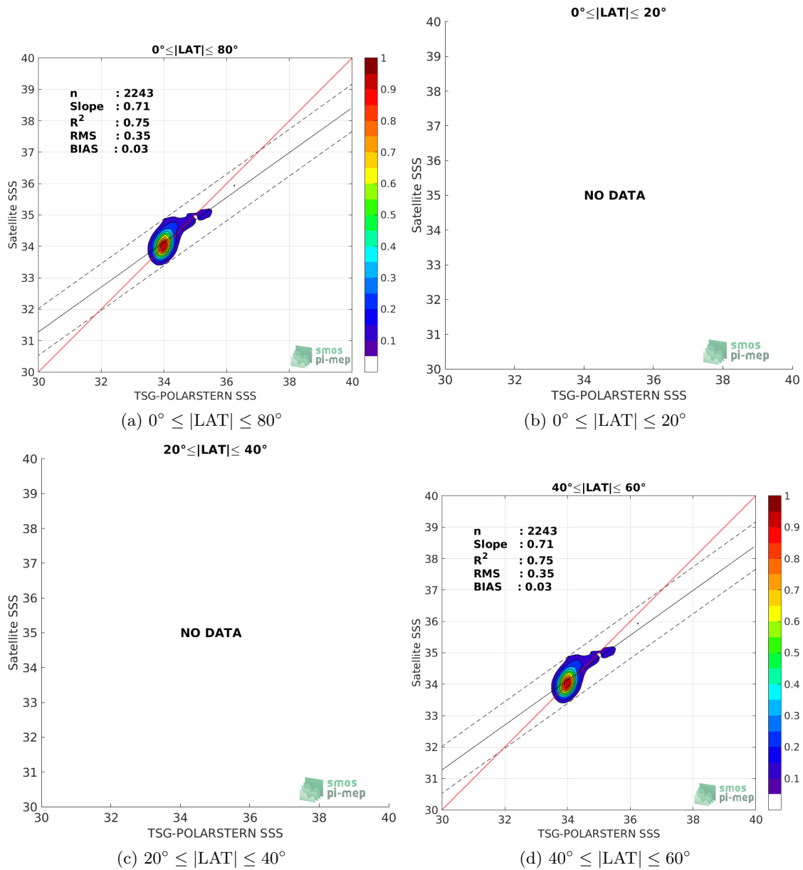
Figure 9: Contour maps of the concentration of SMAP-L3-RSS-V3-MONTHLY-70KM SSS (y-axis) versus TSG-POLARSTERN SSS (x-axis) at match-up pairs for different latitude bands. For each plot, the red line shows x=y . The black thin and dashed lines indicate a linear fit through the data cloud and the \pm 95\% confidence levels, respectively. The number match-up pairs n , the slope and R^2 coefficient of the linear fit, the root mean square (RMS) and the mean bias between satellite and in situ data are indicated for each latitude band in each plots.
