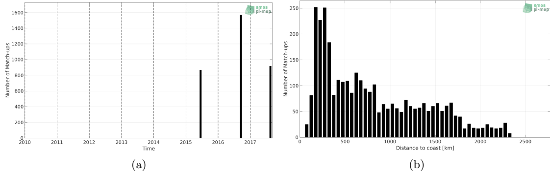
Figure 1: Number of match-ups between TSG-LEGOS-DM and SMAP-L3-RSS-V3-MONTHLY-70KM SSS as a function of time (a) and as function of the distance to coast (b) over the Roaring Forties and Furious Fifties Pi-MEP region and for the full satellite product period.
