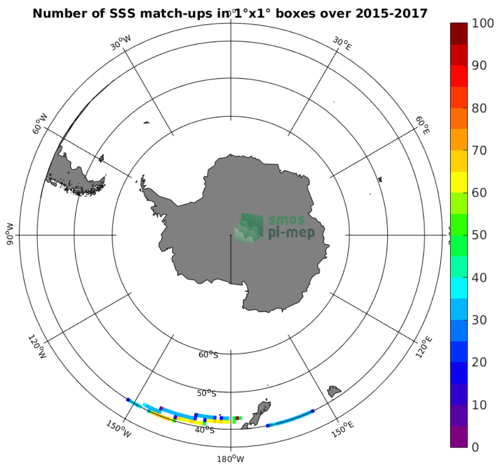
Figure 4: Number of SSS match-ups between TSG-LEGOS-DM SSS and the SMAP-L3-RSS-V3-MONTHLY-70KM SSS product for the Roaring Forties and Furious Fifties Pi-MEP region over 1^\circ \times 1^\circ boxes and for the full satellite product period.
