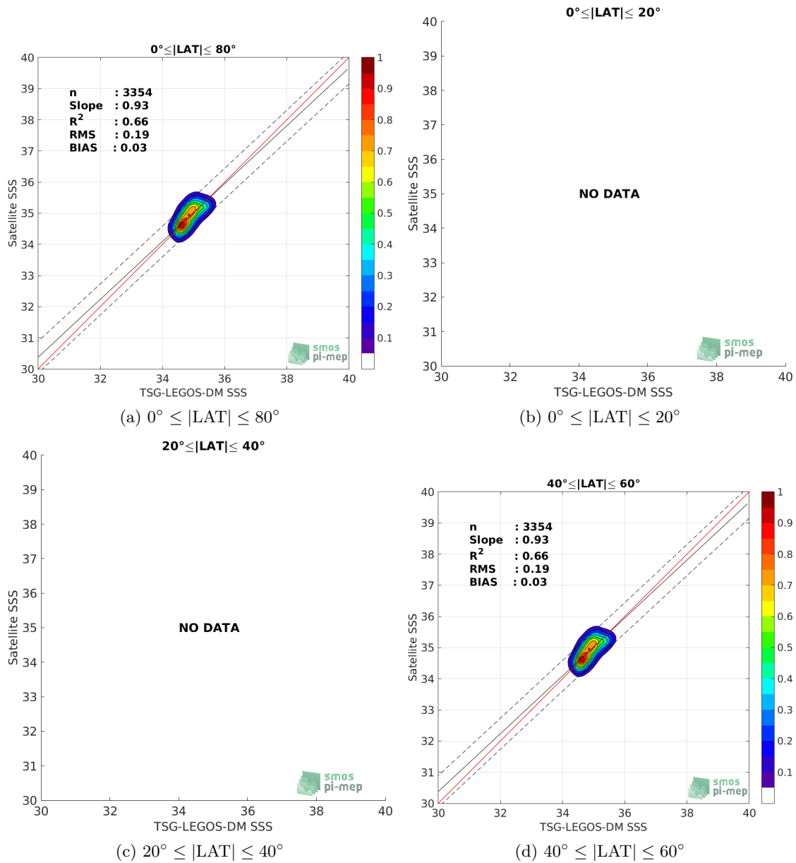
Figure 9: Contour maps of the concentration of SMAP-L3-RSS-V3-MONTHLY-70KM SSS (y-axis) versus TSG-LEGOS-DM SSS (x-axis) at match-up pairs for different latitude bands. For each plot, the red line shows x=y . The black thin and dashed lines indicate a linear fit through the data cloud and the \pm 95\% confidence levels, respectively. The number match-up pairs n , the slope and R^2 coefficient of the linear fit, the root mean square (RMS) and the mean bias between satellite and in situ data are indicated for each latitude band in each plots.
