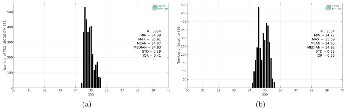
Figure 2: Histograms of SSS from TSG-LEGOS-DM (a) and SMAP-L3-RSS-V3-MONTHLY-70KM (b) considering all match-up pairs per bins of 0.1 over the Roaring Forties and Furious Fifties Pi-MEP region and for the full satellite product period.
