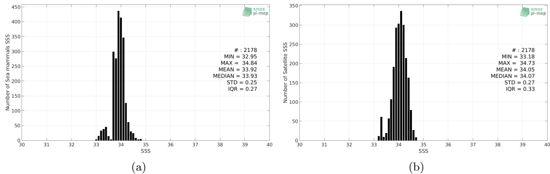
Figure 2: Histograms of SSS from Sea mammals (a) and SMAP-L3-RSS-V3-MONTHLY-70KM (b) considering all match-up pairs per bins of 0.1 over the Roaring Forties and Furious Fifties Pi-MEP region and for the full satellite product period.
