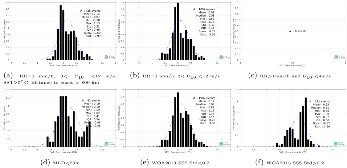
Figure 13: Normalized histogram of \Delta SSS (SMAP-L3-RSS-V3-MONTHLY-70KM - Sea mammals) for 6 different subdatasets corresponding to: RR=0 mm/h, 3 < U_{10} < 12 m/s, SST>5°C, distance to coast > 800 km (a), RR=0 mm/h, 3 < U_{10} < 12 m/s (b), RR>1mm/h and U_{10} < 4 m/s (c), MLD<20m (d), WOA2013 SSS Std<0.2 (e), WOA2013 SSS Std>0.2 (f).
