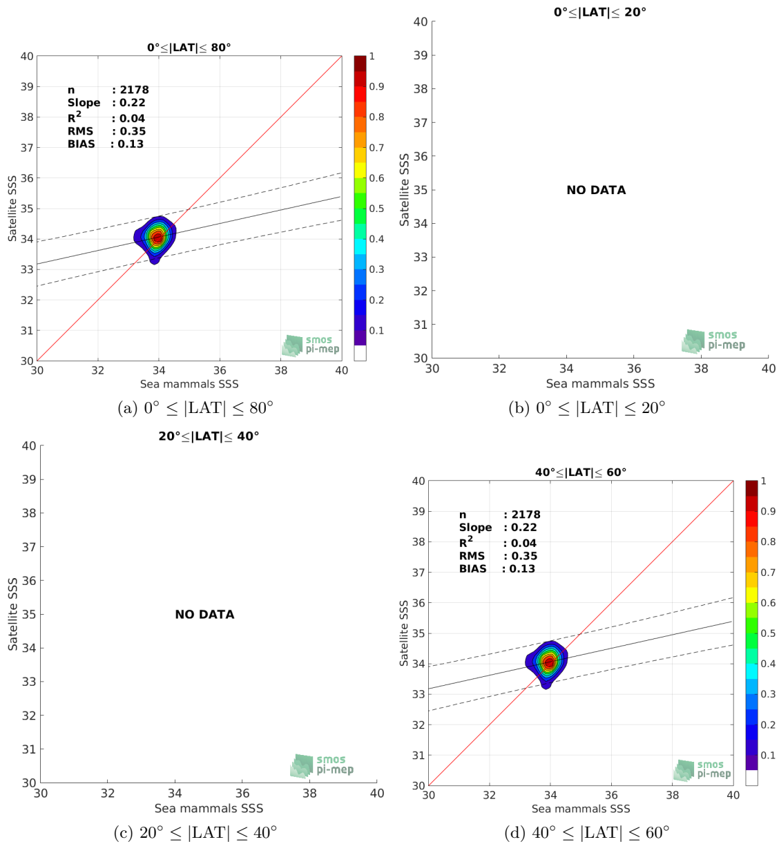
Figure 9: Contour maps of the concentration of SMAP-L3-RSS-V3-MONTHLY-70KM SSS (y-axis) versus Sea mammals SSS (x-axis) at match-up pairs for different latitude bands. For each plot, the red line shows x=y . The black thin and dashed lines indicate a linear fit through the data cloud and the \pm 95\% confidence levels, respectively. The number match-up pairs n , the slope and R^2 coefficient of the linear fit, the root mean square (RMS) and the mean bias between satellite and in situ data are indicated for each latitude band in each plots.
