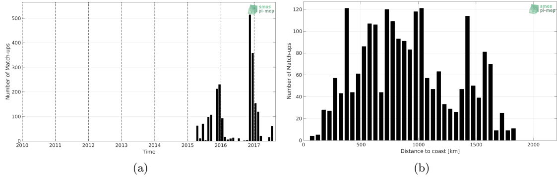
Figure 1: Number of match-ups between Sea mammals and SMAP-L3-RSS-V3-MONTHLY-70KM SSS as a function of time (a) and as function of the distance to coast (b) over the Roaring Forties and Furious Fifties Pi-MEP region and for the full satellite product period.
