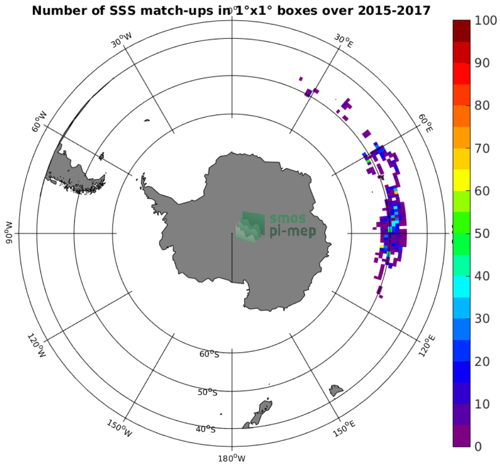
Figure 4: Number of SSS match-ups between Sea mammals SSS and the SMAP-L3-RSS-V3-MONTHLY-70KM SSS product for the Roaring Forties and Furious Fifties Pi-MEP region over 1°x1° boxes and for the full satellite product period.
