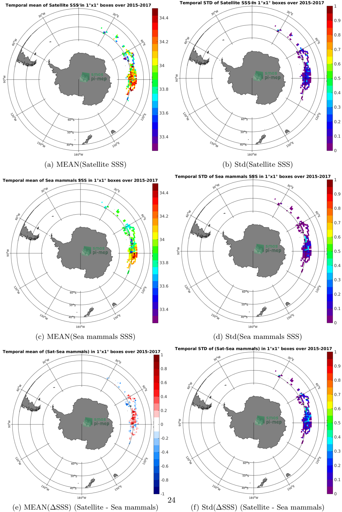
Figure 6: Temporal mean (left) and Std (right) of SSS from SMAP-L3-RSS-V3-MONTHLY-70KM (top), Sea mammals (middle), and of \Delta SSS (Satellite - Sea mammals). Only match-up pairs are used to generate these maps.
