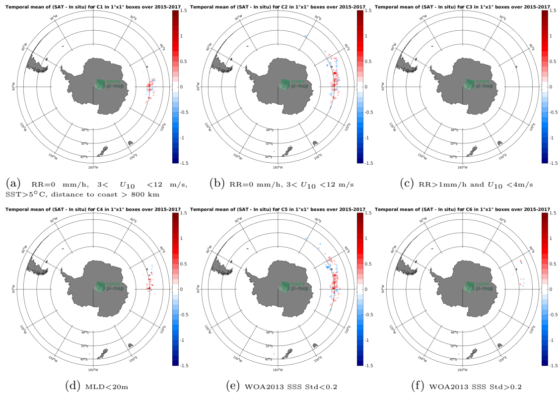
Figure 12: Temporal mean gridded over spatial boxes of size 1^\circ \times 1^\circ of \Delta SSS (SMAP-L3-RSS-V3-MONTHLY-70KM - Sea mammals) for 6 different subdatasets corresponding to:RR=0 mm/h, 3 < U_{10} < 12 m/s, SST > 5^\circ C, distance to coast > 800 km (a), RR=0 mm/h, 3 < U_{10} < 12 m/s (b), RR > 1 mm/h and U_{10} < 4 m/s (c),MLD < 20 m (d),WOA2013 SSS Std < 0.2 (e),WOA2013 SSS Std > 0.2 (f).
