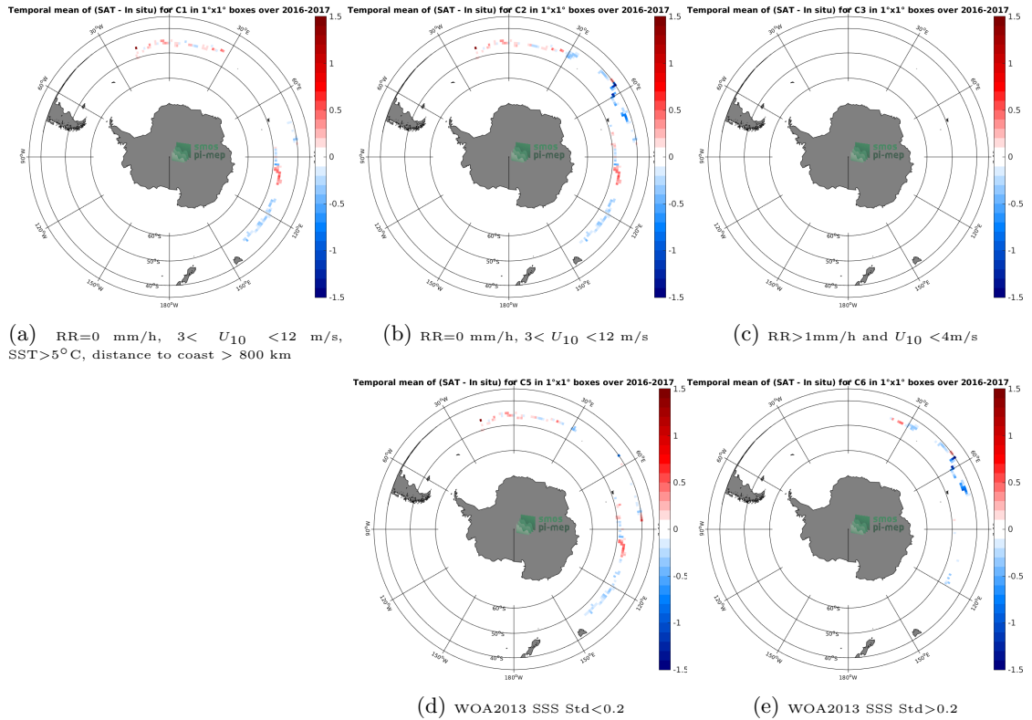
Figure 11: Temporal mean gridded over spatial boxes of size 1^\circ \times 1^\circ of \Delta SSS (SMAP-L3-RSS-V3-MONTHLY-70KM - Surface drifters) for 5 different subdatasets corresponding to:RR=0 mm/h, 3 < U_{10} < 12 m/s, SST > 5^\circ\text{C} , distance to coast > 800 km (a), RR=0 mm/h, 3 < U_{10} < 12 m/s (b), RR > 1 mm/h and U_{10} < 4 m/s (c), WOA2013 SSS Std < 0.2 (d), WOA2013 SSS Std > 0.2 (e).
