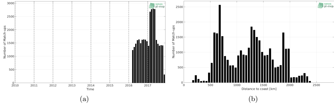
Figure 1: Number of match-ups between Surface drifters and SMAP-L3-RSS-V3-MONTHLY-70KM SSS as a function of time (a) and as function of the distance to coast (b) over the Roaring Forties and Furious Fifties Pi-MEP region and for the full satellite product period.
