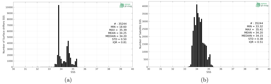
Figure 2: Histograms of SSS from Surface drifters (a) and SMAP-L3-RSS-V3-MONTHLY-70KM (b) considering all match-up pairs per bins of 0.1 over the Roaring Forties and Furious Fifties Pi-MEP region and for the full satellite product period.
