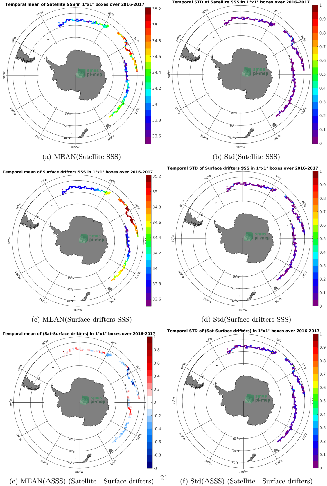
Figure 5: Temporal mean (left) and Std (right) of SSS from SMAP-L3-RSS-V3-MONTHLY-70KM (top), Surface drifters (middle), and of \Delta SSS (Satellite - Surface drifters). Only match-up pairs are used to generate these maps.
