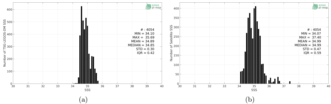
Figure 2: Histograms of SSS from TSG-LEGOS-DM (a) and SMAP-L3-RSS-V3-MONTHLY-0.25DEG-40KM (b) considering all match-up pairs per bins of 0.1 over the Roaring Forties and Furious Fifties Pi-MEP region and for the full satellite product period.
