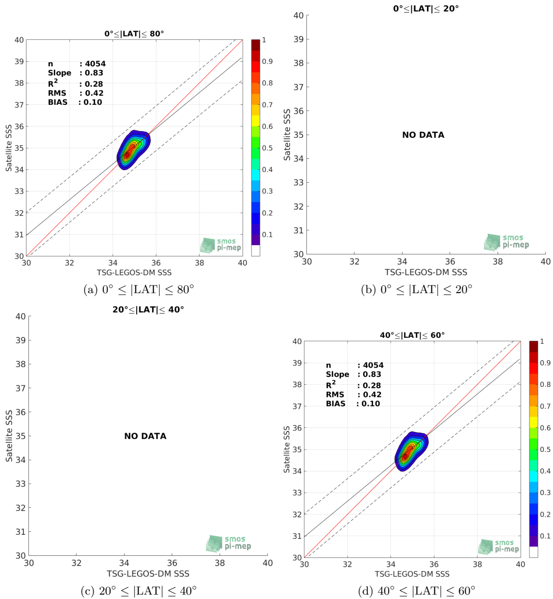
Figure 9: Contour maps of the concentration of SMAP-L3-RSS-V3-MONTHLY-0.25DEG-40KM SSS (y-axis) versus TSG-LEGOS-DM SSS (x-axis) at match-up pairs for different latitude bands. For each plot, the red line shows x=y . The black thin and dashed lines indicate a linear fit through the data cloud and the \pm 95\% confidence levels, respectively. The number match-up pairs n , the slope and R^2 coefficient of the linear fit, the root mean square (RMS) and the mean bias between satellite and in situ data are indicated for each latitude band in each plots.
