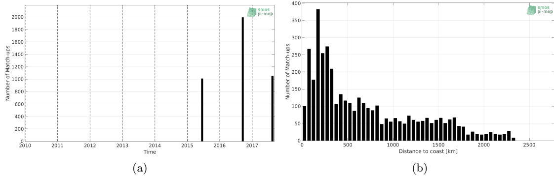
Figure 1: Number of match-ups between TSG-LEGOS-DM and SMAP-L3-RSS-V3-MONTHLY-0.25DEG-40KM SSS as a function of time (a) and as function of the distance to coast (b) over the Roaring Forties and Furious Fifties Pi-MEP region and for the full satellite product period.
