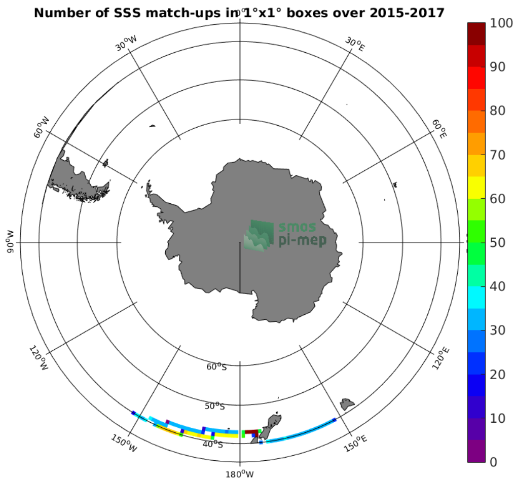
Figure 4: Number of SSS match-ups between TSG-LEGOS-DM SSS and the SMAP-L3-RSS-V3-MONTHLY-0.25DEG-40KM SSS product for the Roaring Forties and Furious Fifties Pi-MEP region over 1^\circ \times 1^\circ boxes and for the full satellite product period.
