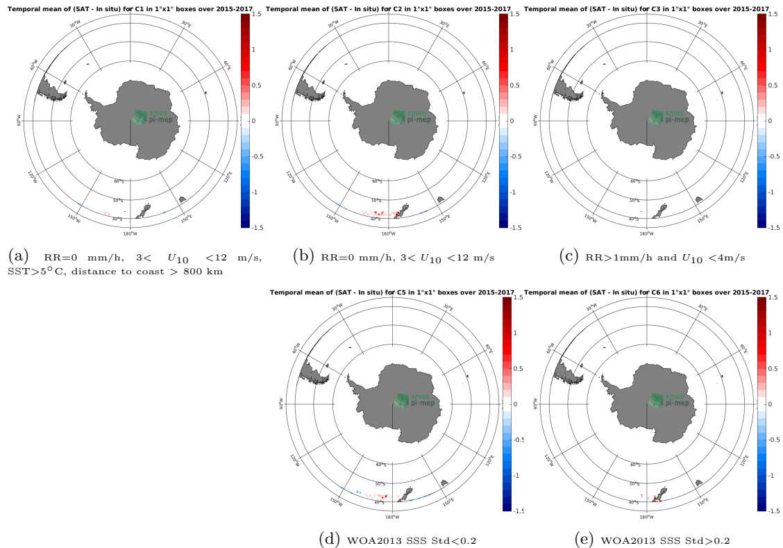
Figure 12: Temporal mean gridded over spatial boxes of size 1^\circ \times 1^\circ of \Delta SSS (SMAP-L3-RSS-V3-MONTHLY-0.25DEG-40KM - TSG-LEGOS-DM) for 5 different subdatasets corresponding to:RR=0 mm/h, 3 < U_{10} < 12 m/s, SST >5^\circ C, distance to coast > 800 km (a), RR=0 mm/h, 3 < U_{10} < 12 m/s (b), RR >1 mm/h and U_{10} < 4 m/s (c), WOA2013 SSS Std <0.2 (d), WOA2013 SSS Std >0.2 (e).
