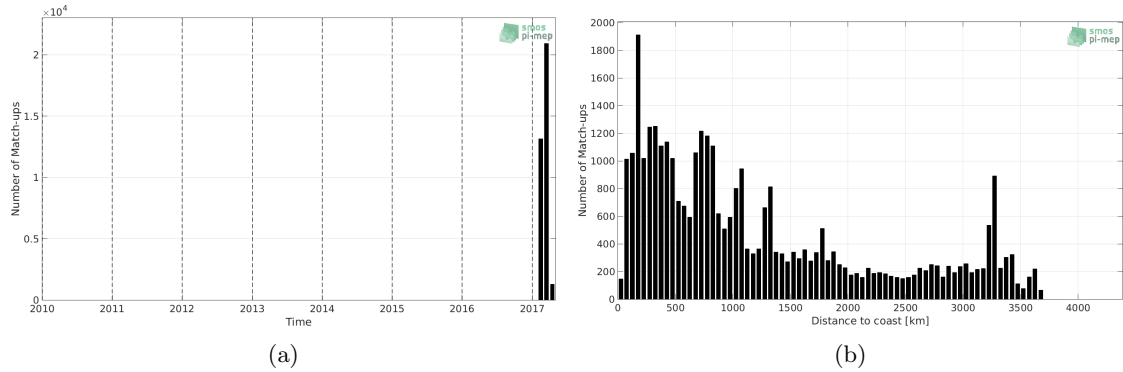
Figure 1: Number of match-ups between TSG-GOSUD-Sailing-ship and SMAP-L3-RSS-V3-MONTHLY-0.25DEG-40KM SSS as a function of time (a) and as function of the distance to coast (b) over the Roaring Forties and Furious Fifties Pi-MEP region and for the full satellite product period.
