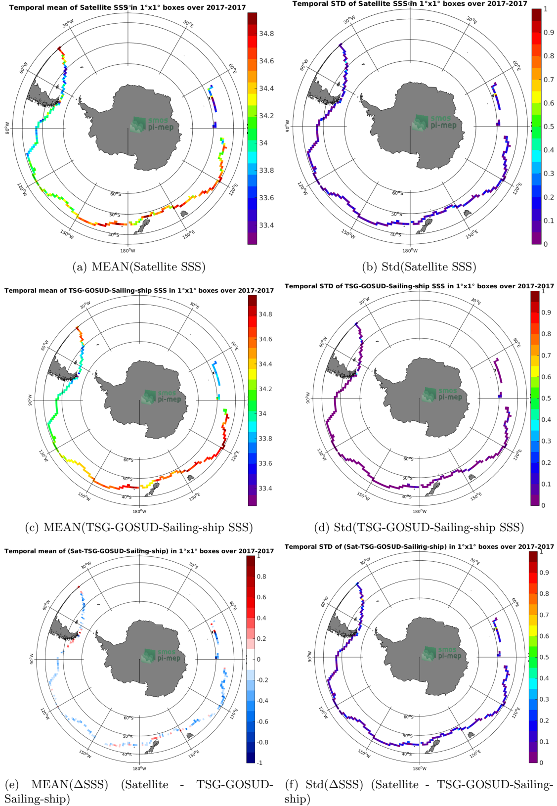
Figure 6: Temporal mean (left) and Std (right) of SSS from SMAP-L3-RSS-V3-MONTHLY-0.25DEG-40KM (top), TSG-GOSUD-Sailing-ship (middle), and of \Delta SSS (Satellite - TSG-GOSUD-Sailing-ship). Only match-up pairs are used to generate these maps.
