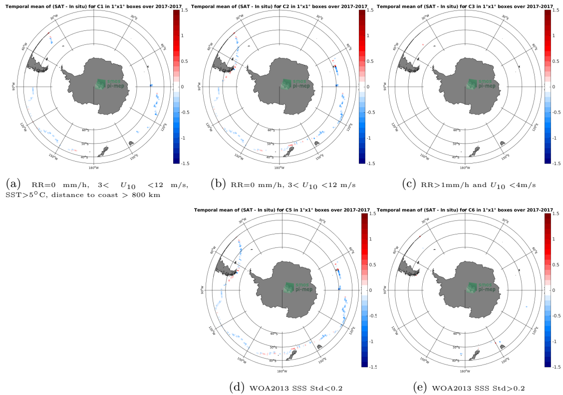
Figure 12: Temporal mean gridded over spatial boxes of size 1^\circ \times 1^\circ of \Delta SSS (SMAP-L3-RSS-V3-MONTHLY-0.25DEG-40KM - TSG-GOSUD-Sailing-ship) for 5 different subdatasets corresponding to:RR=0 mm/h, 3 < U_{10} < 12 m/s, SST >5^\circ C, distance to coast > 800 km (a), RR=0 mm/h, 3 < U_{10} < 12 m/s (b), RR >1 mm/h and U_{10} < 4 m/s (c), WOA2013 SSS Std <0.2 (d), WOA2013 SSS Std >0.2 (e).
