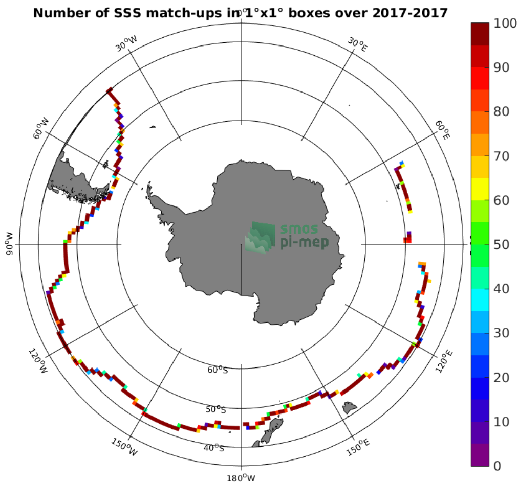
Figure 4: Number of SSS match-ups between TSG-GOSUD-Sailing-ship SSS and the SMAP-L3-RSS-V3-MONTHLY-0.25DEG-40KM SSS product for the Roaring Forties and Furious Fifties Pi-MEP region over 1°x1° boxes and for the full satellite product period.
