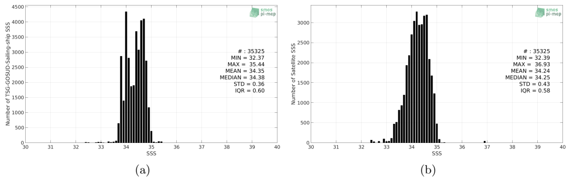
Figure 2: Histograms of SSS from TSG-GOSUD-Sailing-ship (a) and SMAP-L3-RSS-V3-MONTHLY-0.25DEG-40KM (b) considering all match-up pairs per bins of 0.1 over the Roaring Forties and Furious Fifties Pi-MEP region and for the full satellite product period.
