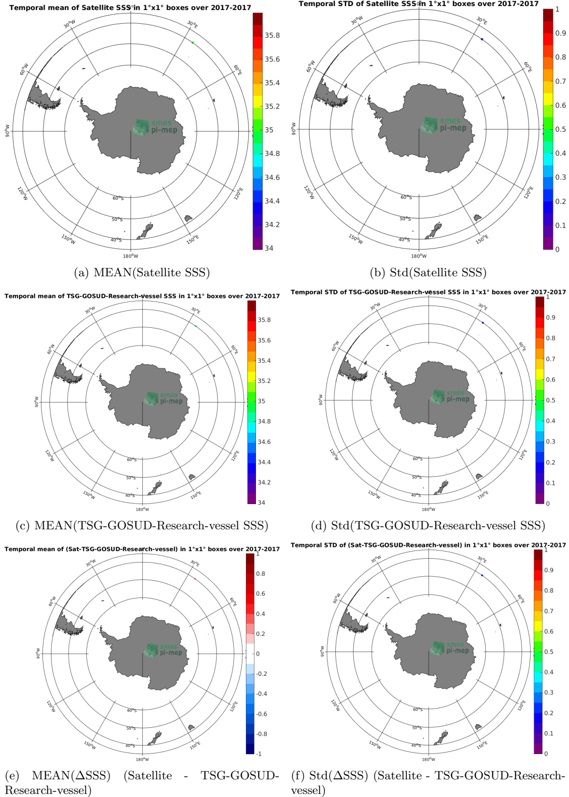
Figure 6: Temporal mean (left) and Std (right) of SSS from SMAP-L3-RSS-V3-MONTHLY-0.25DEG-40KM (top), TSG-GOSUD-Research-vessel (middle), and of \Delta SSS (Satellite - TSG-GOSUD-Research-vessel). Only match-up pairs are used to generate these maps.
