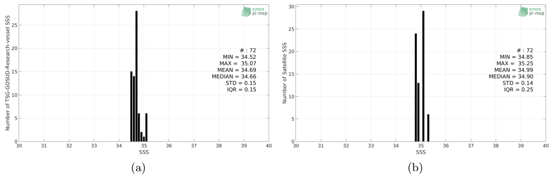
Figure 2: Histograms of SSS from TSG-GOSUD-Research-vessel (a) and SMAP-L3-RSS-V3-MONTHLY-0.25DEG-40KM (b) considering all match-up pairs per bins of 0.1 over the Roaring Forties and Furious Fifties Pi-MEP region and for the full satellite product period.
