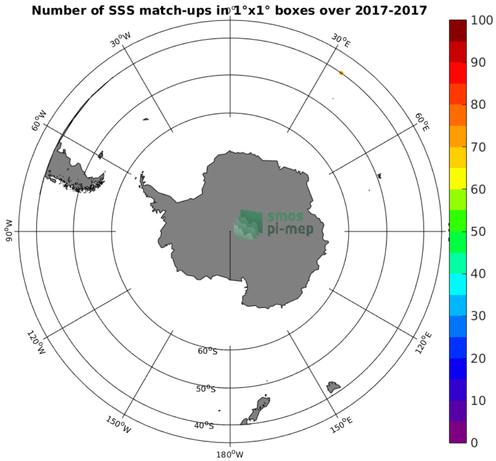
Figure 4: Number of SSS match-ups between TSG-GOSUD-Research-vessel SSS and the SMAP-L3-RSS-V3-MONTHLY-0.25DEG-40KM SSS product for the Roaring Forties and Furious Fifties Pi-MEP region over 1°x1° boxes and for the full satellite product period.
