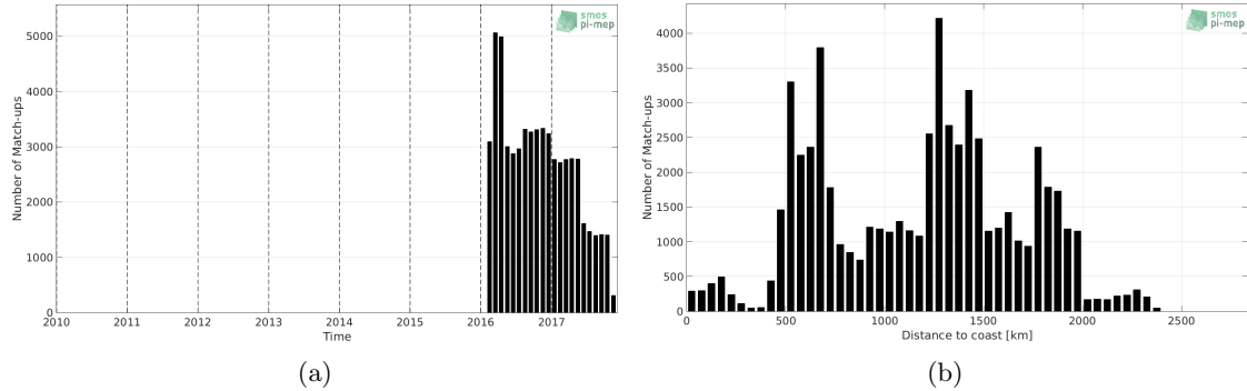
Figure 1: Number of match-ups between Surface drifters and SMAP-L3-RSS-V3-MONTHLY-0.25DEG-40KM SSS as a function of time (a) and as function of the distance to coast (b) over the Roaring Forties and Furious Fifties Pi-MEP region and for the full satellite product period.
