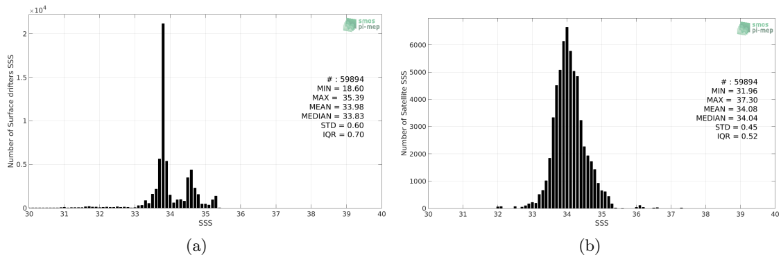
Figure 2: Histograms of SSS from Surface drifters (a) and SMAP-L3-RSS-V3-MONTHLY-0.25DEG-40KM (b) considering all match-up pairs per bins of 0.1 over the Roaring Forties and Furious Fifties Pi-MEP region and for the full satellite product period.
