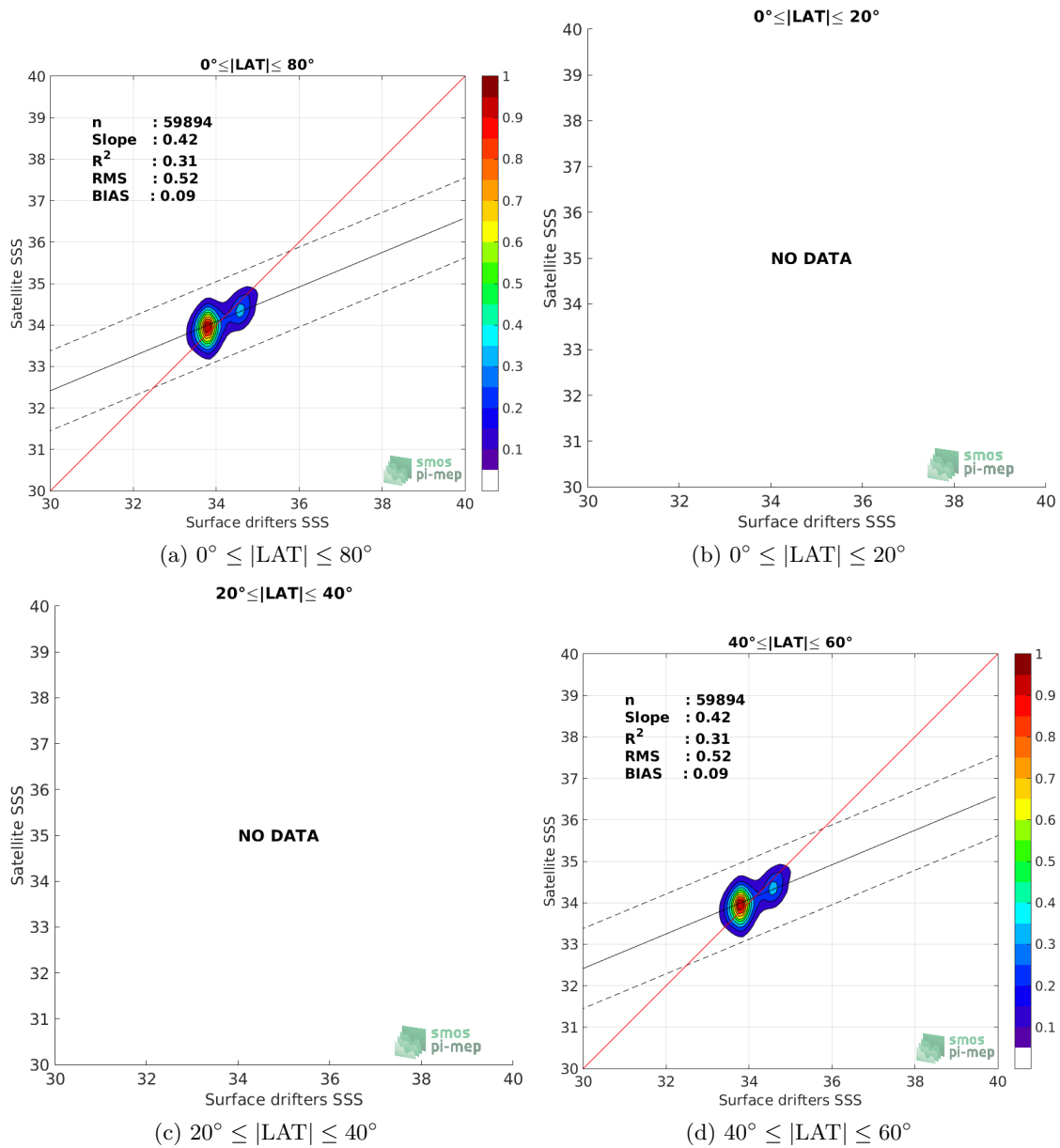
Figure 8: Contour maps of the concentration of SMAP-L3-RSS-V3-MONTHLY-0.25DEG-40KM SSS (y-axis) versus Surface drifters SSS (x-axis) at match-up pairs for different latitude bands. For each plot, the red line shows x=y . The black thin and dashed lines indicate a linear fit through the data cloud and the \pm 95\% confidence levels, respectively. The number match-up pairs n , the slope and R^2 coefficient of the linear fit, the root mean square (RMS) and the mean bias between satellite and in situ data are indicated for each latitude band in each plots.
