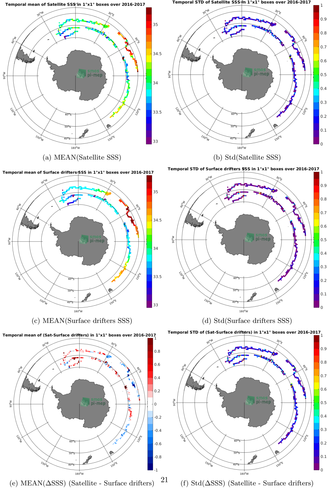
Figure 5: Temporal mean (left) and Std (right) of SSS from SMAP-L3-RSS-V3-MONTHLY-0.25DEG-40KM (top), Surface drifters (middle), and of \Delta SSS (Satellite - Surface drifters). Only match-up pairs are used to generate these maps.
