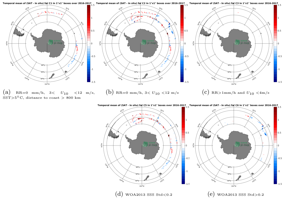
Figure 11: Temporal mean gridded over spatial boxes of size 1^\circ \times 1^\circ of \Delta SSS (SMAP-L3-RSS-V3-MONTHLY-0.25DEG-40KM - Surface drifters) for 5 different subdatasets corresponding to:RR=0 mm/h, 3 < U_{10} < 12 m/s, SST >5^\circ C, distance to coast > 800 km (a), RR=0 mm/h, 3 < U_{10} < 12 m/s (b), RR >1 mm/h and U_{10} < 4 m/s (c), WOA2013 SSS Std <0.2 (d), WOA2013 SSS Std >0.2 (e).
