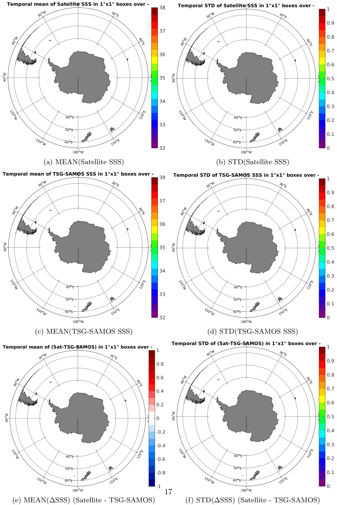
Figure 6: Temporal mean (left) and STD (right) of SSS from SMAP-L3-RSS-V2-8DAY-RUNNING-70KM (top), TSG-SAMOS (middle), and of \Delta SSS (Satellite - TSG-SAMOS). Only match-up pairs are used to generate these maps.
