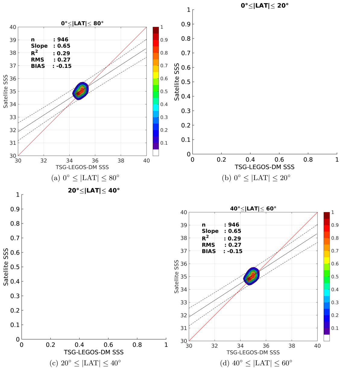
Figure 9: Contour maps of the concentration of SMAP-L3-RSS-V2-8DAY-RUNNING-70KM SSS (y-axis) versus TSG-LEGOS-DM SSS (x-axis) at match-up pairs for different latitude bands. For each plot, the red line shows x=y . The black thin and dashed lines indicate a linear fit through the data cloud and the \pm 95\% confidence levels, respectively. The number match-up pairs n , the slope and R^2 coefficient of the linear fit, the root mean square (RMS) and the mean bias between satellite and in situ data are indicated for each latitude band in each plots.
