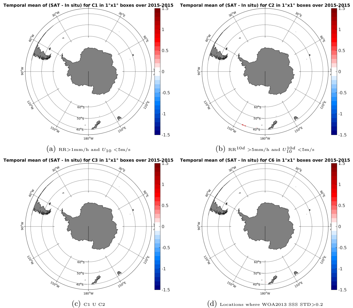
Figure 12: Temporal mean gridded over spatial boxes of size 1^\circ \times 1^\circ of \Delta SSS (SMAP-L3-RSS-V2-8DAY-RUNNING-70KM - TSG-LEGOS-DM) for 4 different subdatasets corresponding to: RR > 1\text{mm/h} and U_{10} < 5\text{m/s} (a), RR^{10d} > 5\text{mm/h} and U_{10}^{10d} < 5\text{m/s} (b), C1 U C2 (c), Locations where WOA2013 SSS STD > 0.2 (d).
