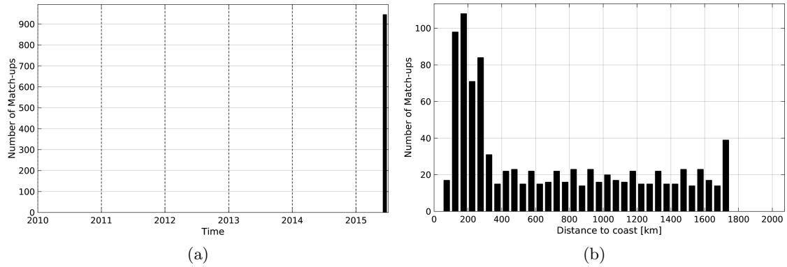
Figure 1: Number of match-ups between TSG-LEGOS-DM and SMAP-L3-RSS-V2-8DAY-RUNNING-70KM SSS as a function of time (a) and as function of the distance to coast (b) over the Roaring Forties and Furious Fifties Pi-MEP region and for the full satellite product period.
