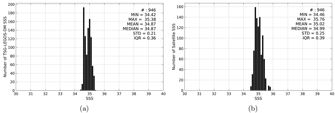
Figure 2: Histograms of SSS from TSG-LEGOS-DM (a) and SMAP-L3-RSS-V2-8DAY-RUNNING-70KM (b) considering all match-up pairs per bins of 0.1 over the Roaring Forties and Furious Fifties Pi-MEP region and for the full satellite product period.
