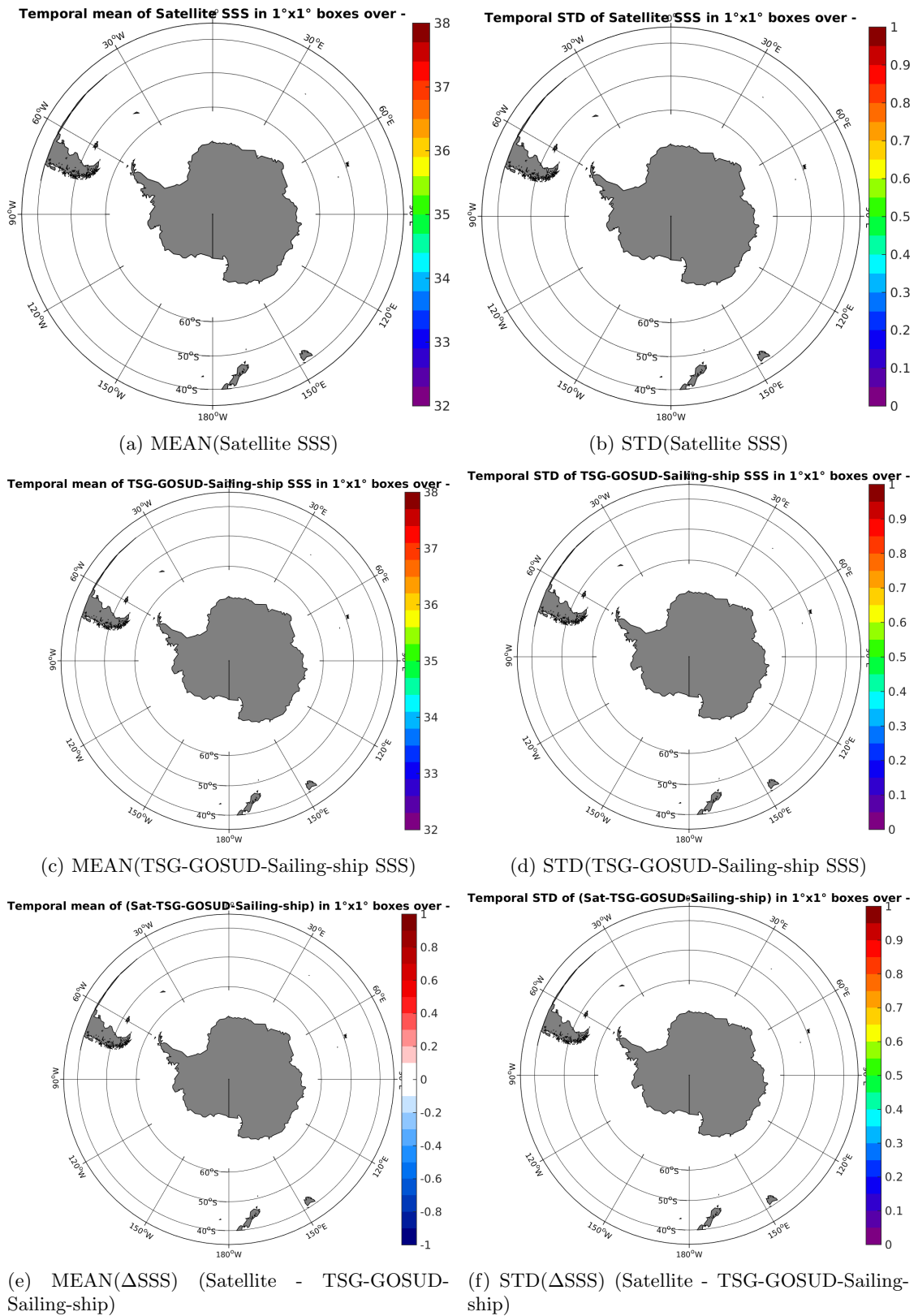
Figure 6: Temporal mean (left) and STD (right) of SSS from SMAP-L3-RSS-V2-8DAY-RUNNING-70KM (top), TSG-GOSUD-Sailing-ship (middle), and of \Delta SSS (Satellite - TSG-GOSUD-Sailing-ship). Only match-up pairs are used to generate these maps.
