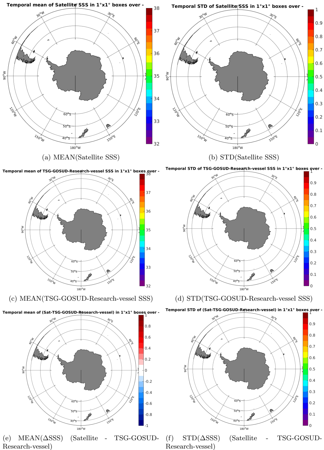
Figure 6: Temporal mean (left) and STD (right) of SSS from SMAP-L3-RSS-V2-8DAY-RUNNING-70KM (top), TSG-GOSUD-Research-vessel (middle), and of \Delta SSS (Satellite - TSG-GOSUD-Research-vessel). Only match-up pairs are used to generate these maps.
