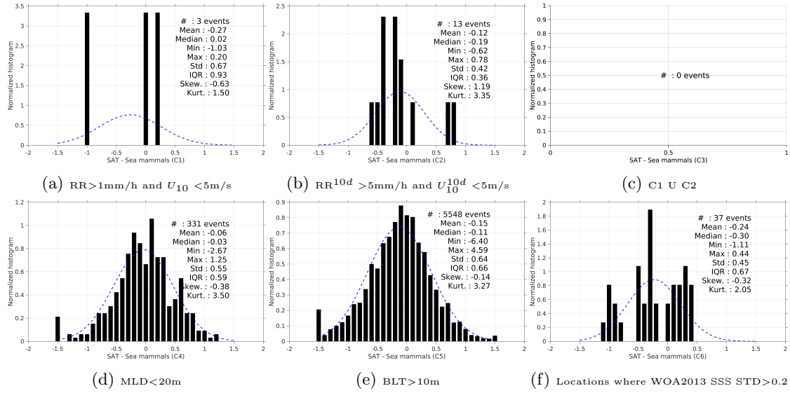
Figure 13: Normalized histogram of \Delta SSS (SMAP-L3-RSS-V2-8DAY-RUNNING-70KM - Sea mammals) for 6 different subdatasets corresponding to: RR>1mm/h and U_{10} < 5\text{m/s} (a), RR^{10d} > 5\text{mm/h} and U_{10}^{10d} < 5\text{m/s} (b), C1 U C2 (c), MLD<20m (d), BLT>10m (e), Locations where WOA2013 SSS STD>0.2 (f).
