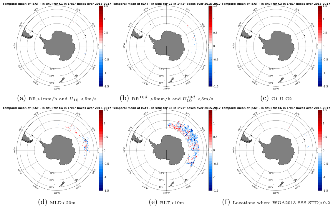
Figure 12: Temporal mean gridded over spatial boxes of size 1^\circ \times 1^\circ of \Delta SSS (SMAP-L3-RSS-V2-8DAY-RUNNING-70KM - Sea mammals) for 6 different subdatasets corresponding to: RR > 1\text{mm/h} and U_{10} < 5\text{m/s} (a), RR^{10d} > 5\text{mm/h} and U_{10}^{10d} < 5\text{m/s} (b), C1 U C2 (c), MLD < 20\text{m} (d), BLT > 10\text{m} (e), Locations where WOA2013 SSS STD > 0.2 (f).
