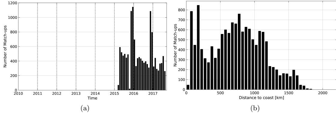
Figure 1: Number of match-ups between Sea mammals and SMAP-L3-RSS-V2-8DAY-RUNNING-70KM SSS as a function of time (a) and as function of the distance to coast (b) over the Roaring Forties and Furious Fifties Pi-MEP region and for the full satellite product period.
