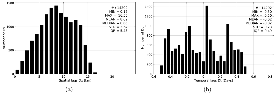
Figure 5: Histograms of the spatial (a) and temporal (b) lags between the time of the Sea mammals measurements and the date of the corresponding SMAP-L3-RSS-V2-8DAY-RUNNING-70KM SSS product.
