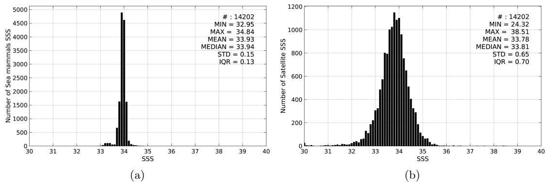
Figure 2: Histograms of SSS from Sea mammals (a) and SMAP-L3-RSS-V2-8DAY-RUNNING-70KM (b) considering all match-up pairs per bins of 0.1 over the Roaring Forties and Furious Fifties Pi-MEP region and for the full satellite product period.
