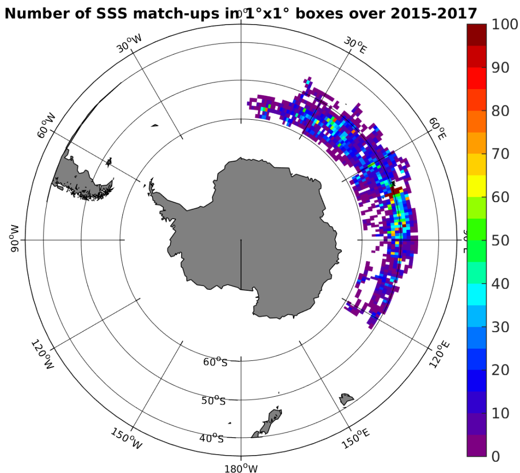
Figure 4: Number of SSS match-ups between Sea mammals SSS and the SMAP-L3-RSS-V2-8DAY-RUNNING-70KM SSS product for the Roaring Forties and Furious Fifties Pi-MEP region over 1^\circ \times 1^\circ boxes and for the full satellite product period.
