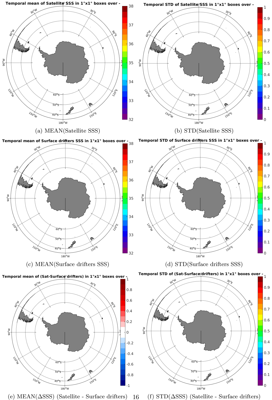
Figure 5: Temporal mean (left) and STD (right) of SSS from SMAP-L3-RSS-V2-8DAY-RUNNING-70KM (top), Surface drifters (middle), and of \Delta SSS (Satellite - Surface drifters). Only match-up pairs are used to generate these maps.
