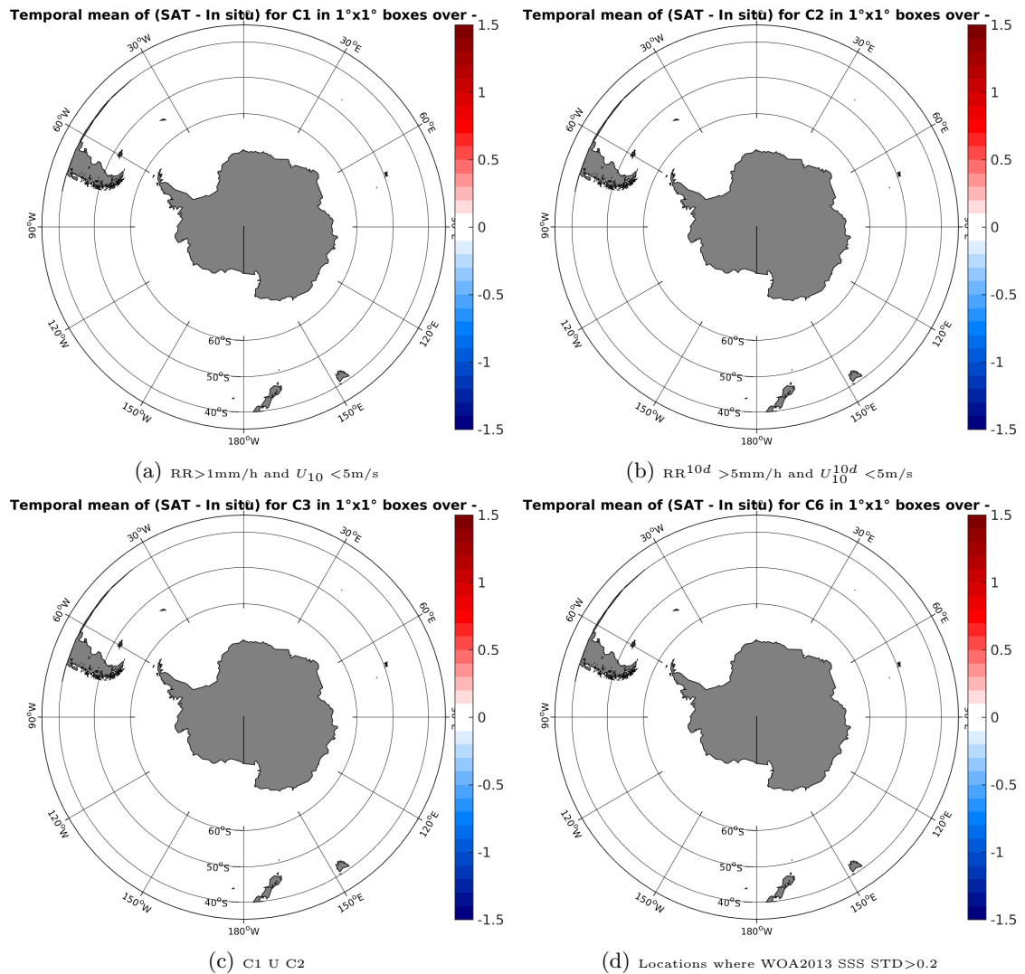
Figure 11: Temporal mean gridded over spatial boxes of size 1^\circ \times 1^\circ of \Delta SSS (SMAP-L3-RSS-V2-8DAY-RUNNING-70KM - Surface drifters) for 4 different subdatasets corresponding to:RR > 1 mm/h and U_{10} < 5 m/s (a), RR 10d > 5 mm/h and U_{10}^{10d} < 5 m/s (b), C1 U C2 (c),Locations where WOA2013 SSS STD > 0.2 (d).
