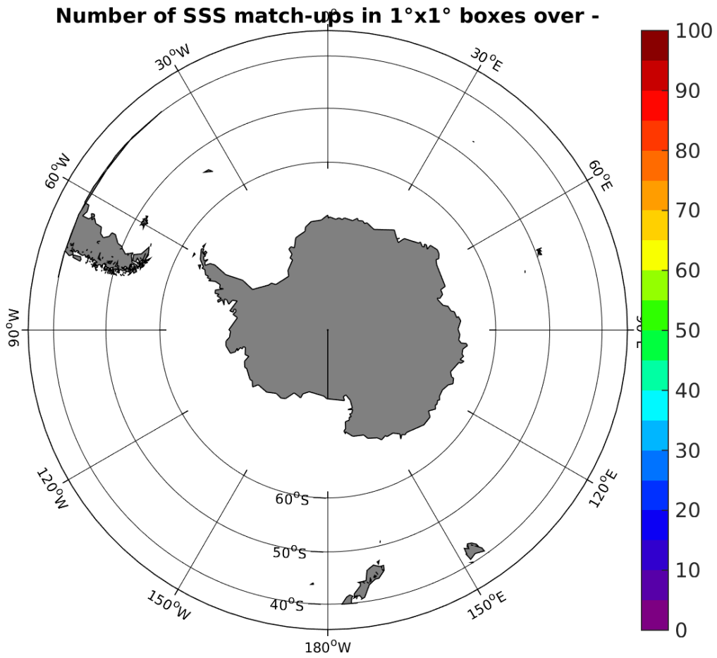
Figure 3: Number of SSS match-ups between Surface drifters SSS and the SMAP-L3-RSS-V2-8DAY-RUNNING-70KM SSS product for the Roaring Forties and Furious Fifties Pi-MEP region over 1°x1° boxes and for the full satellite product period.
