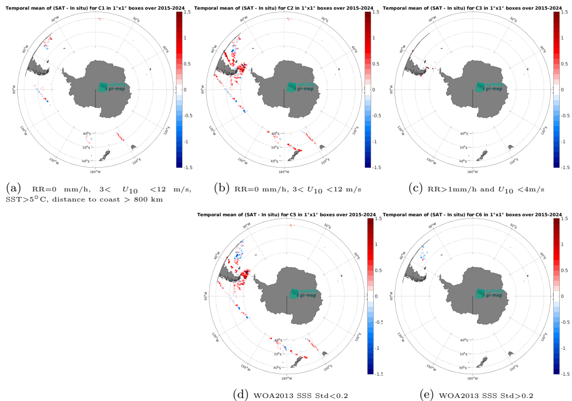
Figure 14: Temporal mean gridded over spatial boxes of size 1^\circ \times 1^\circ of \Delta\text{SSS} (SMAP SSS L3 v5.0 - 8-Day running (JPL) - TSG (SAMOS)) for 5 different subdatasets corresponding to: RR=0 mm/h, 3 < U_{10} < 12 m/s, SST > 5^\circ\text{C} , distance to coast > 800 km (a), RR=0 mm/h, 3 < U_{10} < 12 m/s (b), RR > 1mm/h and U_{10} < 4 m/s (c), WOA2013 SSS Std < 0.2 (d), WOA2013 SSS Std > 0.2 (e).
