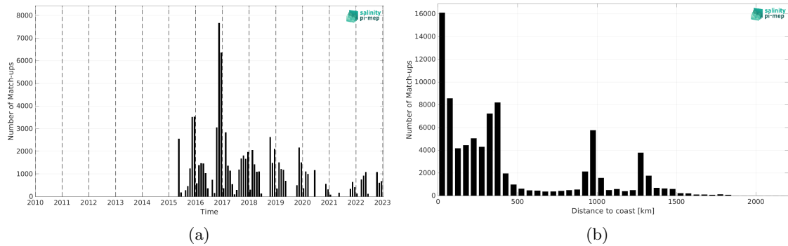
Figure 2: Number of match-ups between TSG (SAMOS) and SMAP SSS L3 v5.0 - 8-Day running (JPL) SSS as a function of time (a) and as function of the distance to coast (b) over the Roaring Forties and Furious Fifties Pi-MEP region and for the full satellite product period.
