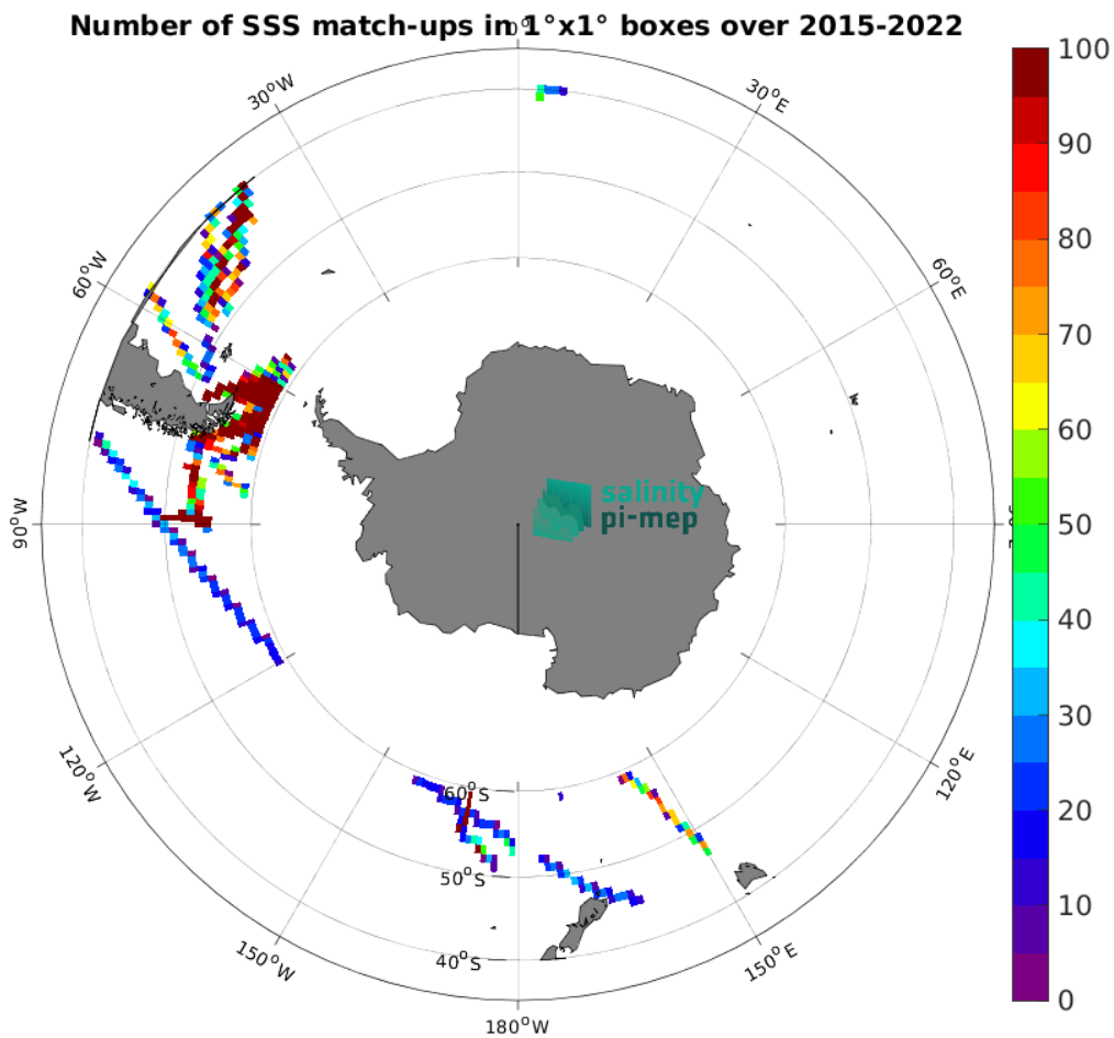
Figure 5: Number of SSS match-ups between TSG (SAMOS) SSS and the SMAP SSS L3 v5.0 - 8-Day running (JPL) SSS product for the Roaring Forties and Furious Fifties Pi-MEP region over 1^\circ \times 1^\circ boxes and for the full satellite product period.
