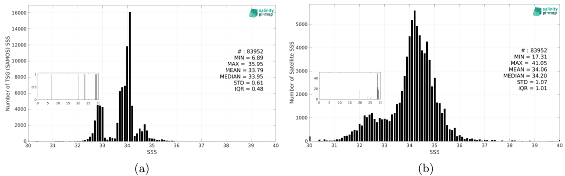
Figure 3: Histograms of SSS from TSG (SAMOS) (a) and SMAP SSS L3 v5.0 - 8-Day running (JPL) (b) considering all match-up pairs per bins of 0.1 over the Roaring Forties and Furious Fifties Pi-MEP region and for the full satellite product period.
