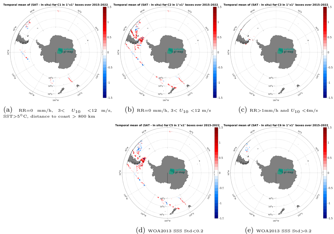
Figure 14: Temporal mean gridded over spatial boxes of size 1^\circ \times 1^\circ of \Delta SSS (SMAP SSS L3 v5.0 - 8-Day running (JPL) - TSG (SAMOS)) for 5 different subdatasets corresponding to:RR=0 mm/h, 3 < U_{10} < 12 m/s, SST > 5^\circ\text{C} , distance to coast > 800 km (a), RR=0 mm/h, 3 < U_{10} < 12 m/s (b), RR > 1 mm/h and U_{10} < 4 m/s (c), WOA2013 SSS Std < 0.2 (d), WOA2013 SSS Std > 0.2 (e).
