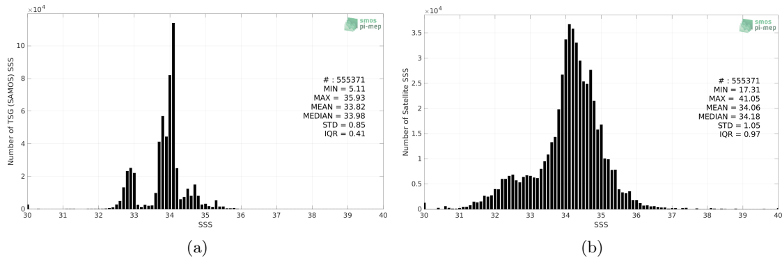
Figure 2: Histograms of SSS from TSG (SAMOS) (a) and SMAP SSS L3 v5.0 - 8-Day running (JPL) (b) considering all match-up pairs per bins of 0.1 over the Roaring Forties and Furious Fifties Pi-MEP region and for the full satellite product period.
