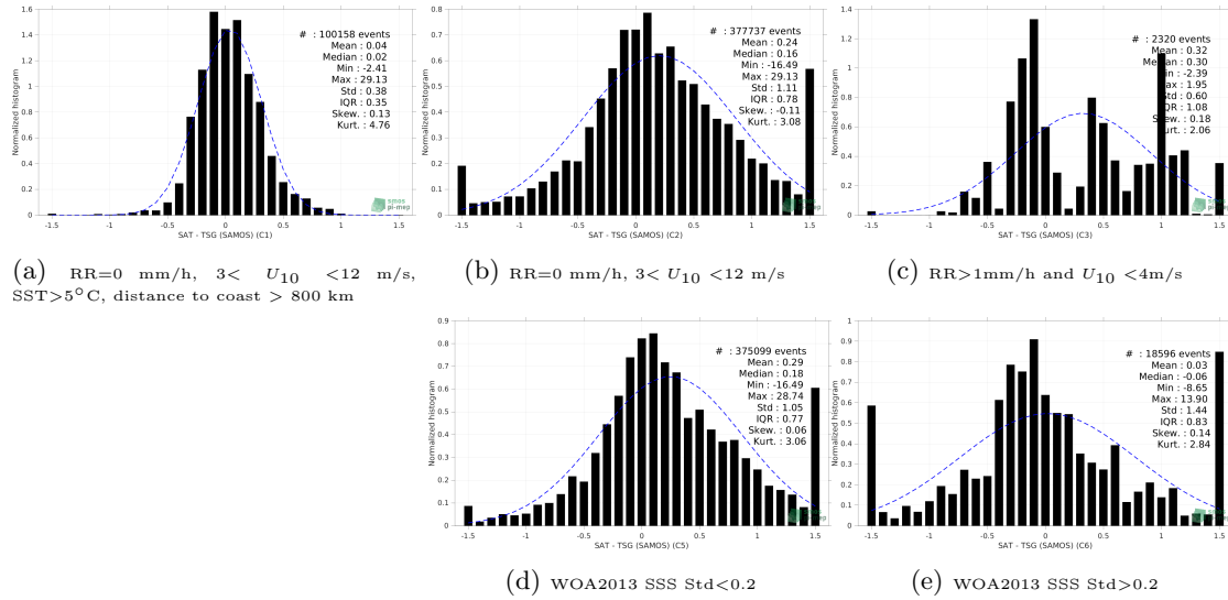
Figure 13: Normalized histogram of \Delta SSS (SMAP SSS L3 v5.0 - 8-Day running (JPL) - TSG (SAMOS)) for 5 different subdatasets corresponding to: RR=0 mm/h, 3 < U_{10} < 12 m/s, SST >5^{\circ}\text{C} , distance to coast > 800 km (a), RR=0 mm/h, 3 < U_{10} < 12 m/s (b), RR >1 mm/h and U_{10} < 4 m/s (c), WOA2013 SSS Std <0.2 (d), WOA2013 SSS Std >0.2 (e).
