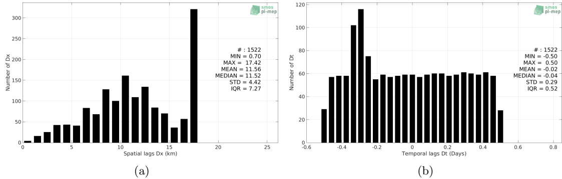
Figure 5: Histograms of the spatial (a) and temporal (b) lags between the time of the TSG (SAMOS) measurements and the date of the corresponding SMAP SSS L3 v5.0 - 8-Day running (JPL) SSS product.
