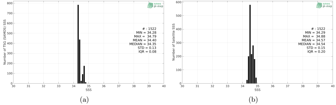
Figure 2: Histograms of SSS from TSG (SAMOS) (a) and SMAP SSS L3 v5.0 - 8-Day running (JPL) (b) considering all match-up pairs per bins of 0.1 over the Roaring Forties and Furious Fifties Pi-MEP region and for the full satellite product period.
