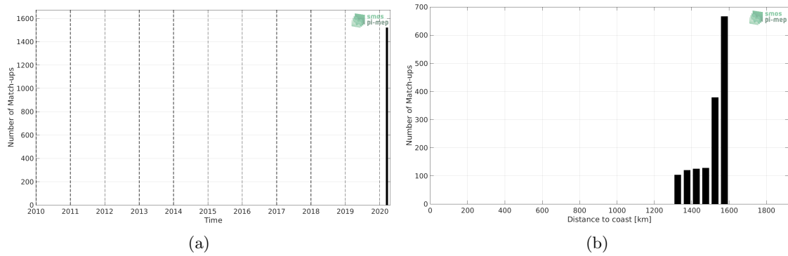
Figure 1: Number of match-ups between TSG (SAMOS) and SMAP SSS L3 v5.0 - 8-Day running (JPL) SSS as a function of time (a) and as function of the distance to coast (b) over the Roaring Forties and Furious Fifties Pi-MEP region and for the full satellite product period.
