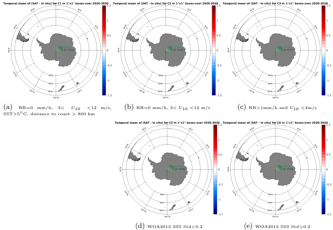
Figure 12: Temporal mean gridded over spatial boxes of size 1^{\circ}\times 1^{\circ} of \Delta\text{SSS} (SMAP SSS L3 v5.0 - 8-Day running (JPL) - TSG (SAMOS)) for 5 different subdatasets corresponding to:RR=0 mm/h, 3 < U_{10} < 12 m/s, SST >5^{\circ}\text{C} , distance to coast > 800 km (a), RR=0 mm/h, 3 < U_{10} < 12 m/s (b), RR >1 mm/h and U_{10} < 4 m/s (c), WOA2013 SSS Std <0.2 (d), WOA2013 SSS Std >0.2 (e).
