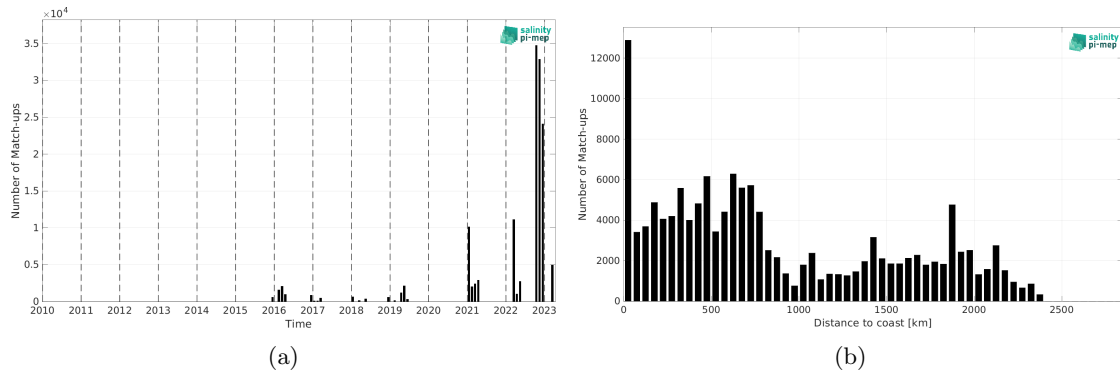
Figure 2: Number of match-ups between TSG (Polarstern) and SMAP SSS L3 v5.0 - 8-Day running (JPL) SSS as a function of time (a) and as function of the distance to coast (b) over the Roaring Forties and Furious Fifties Pi-MEP region and for the full satellite product period.
