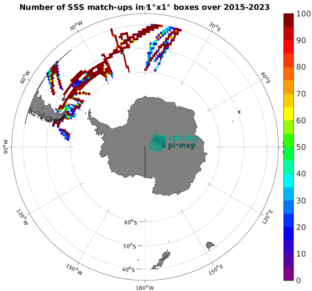
Figure 5: Number of SSS match-ups between TSG (Polarstern) SSS and the SMAP SSS L3 v5.0 - 8-Day running (JPL) SSS product for the Roaring Forties and Furious Fifties Pi-MEP region over 1^\circ \times 1^\circ boxes and for the full satellite product period.
