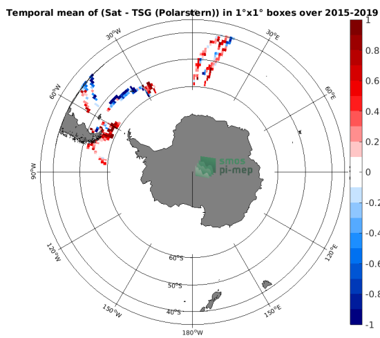
(e) MEAN( \Delta SSS) (Satellite - TSG (Polarstern))
