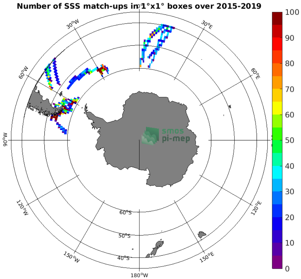
Figure 4: Number of SSS match-ups between TSG (Polarstern) SSS and the SMAP SSS L3 v5.0 - 8-Day running (JPL) SSS product for the Roaring Forties and Furious Fifties Pi-MEP region over 1°x1° boxes and for the full satellite product period.
