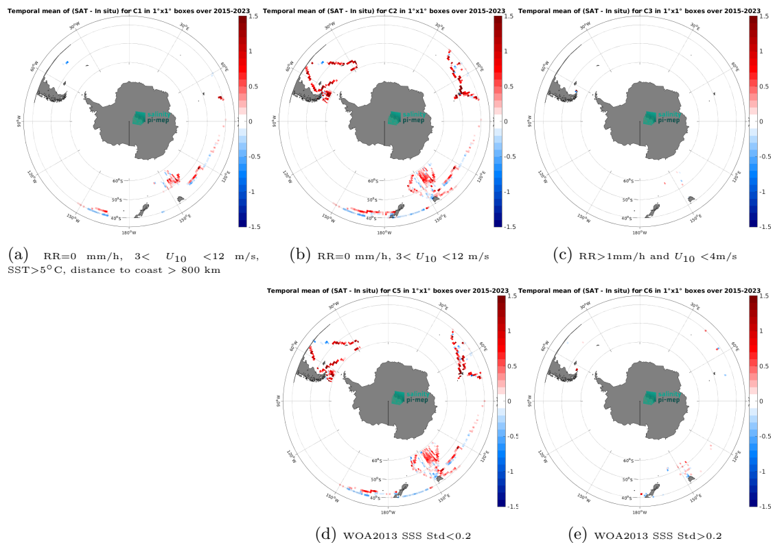
Figure 14: Temporal mean gridded over spatial boxes of size 1^\circ \times 1^\circ of \Delta SSS (SMAP SSS L3 v5.0 - 8-Day running (JPL) - TSG (LEGOS-DM)) for 5 different subdatasets corresponding to:RR=0 mm/h, 3 < U_{10} < 12 m/s, SST>5°C, distance to coast > 800 km (a), RR=0 mm/h, 3 < U_{10} < 12 m/s (b), RR>1mm/h and U_{10} < 4 m/s (c), WOA2013 SSS Std<0.2 (d), WOA2013 SSS Std>0.2 (e).
