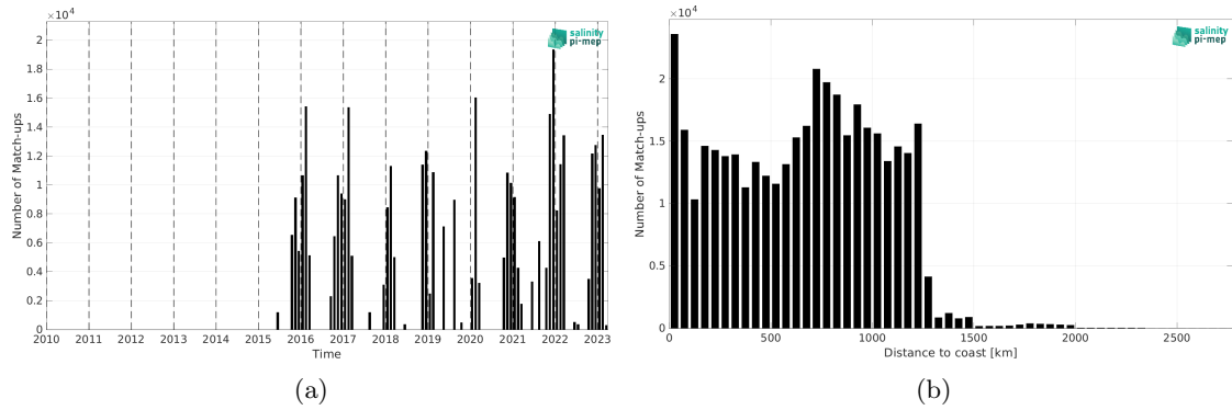
Figure 2: Number of match-ups between TSG (LEGOS-DM) and SMAP SSS L3 v5.0 - 8-Day running (JPL) SSS as a function of time (a) and as function of the distance to coast (b) over the Roaring Forties and Furious Fifties Pi-MEP region and for the full satellite product period.
