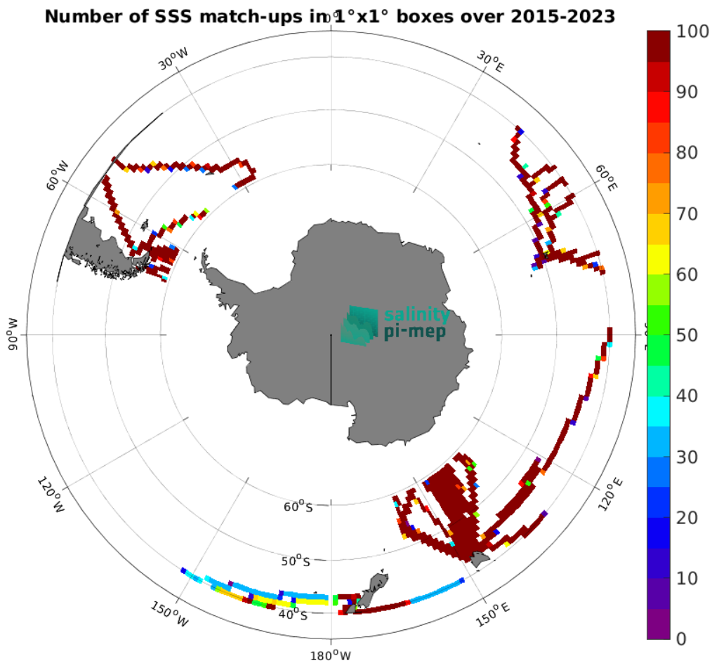
Figure 5: Number of SSS match-ups between TSG (LEGOS-DM) SSS and the SMAP SSS L3 v5.0 - 8-Day running (JPL) SSS product for the Roaring Forties and Furious Fifties Pi-MEP region over 1^\circ \times 1^\circ boxes and for the full satellite product period.
