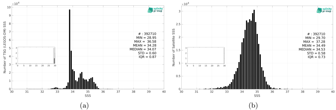
Figure 3: Histograms of SSS from TSG (LEGOS-DM) (a) and SMAP SSS L3 v5.0 - 8-Day running (JPL) (b) considering all match-up pairs per bins of 0.1 over the Roaring Forties and Furious Fifties Pi-MEP region and for the full satellite product period.
