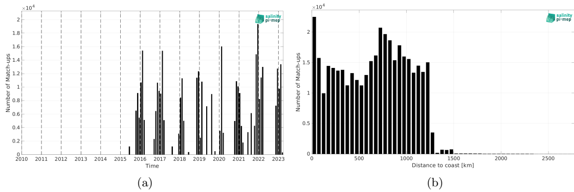
Figure 1: Number of match-ups between TSG (LEGOS-DM) and SMAP SSS L3 v5.0 - 8-Day running (JPL) SSS as a function of time (a) and as function of the distance to coast (b) over the Roaring Forties and Furious Fifties Pi-MEP region and for the full satellite product period.
