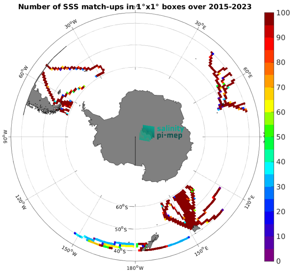
Figure 4: Number of SSS match-ups between TSG (LEGOS-DM) SSS and the SMAP SSS L3 v5.0 - 8-Day running (JPL) SSS product for the Roaring Forties and Furious Fifties Pi-MEP region over 1^{\circ} \times 1^{\circ} boxes and for the full satellite product period.
