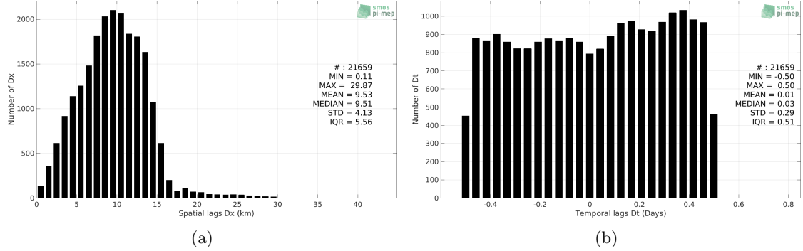
Figure 5: Histograms of the spatial (a) and temporal (b) lags between the time of the TSG (LEGOS-DM) measurements and the date of the corresponding SMAP SSS L3 v5.0 - 8-Day running (JPL) SSS product.
