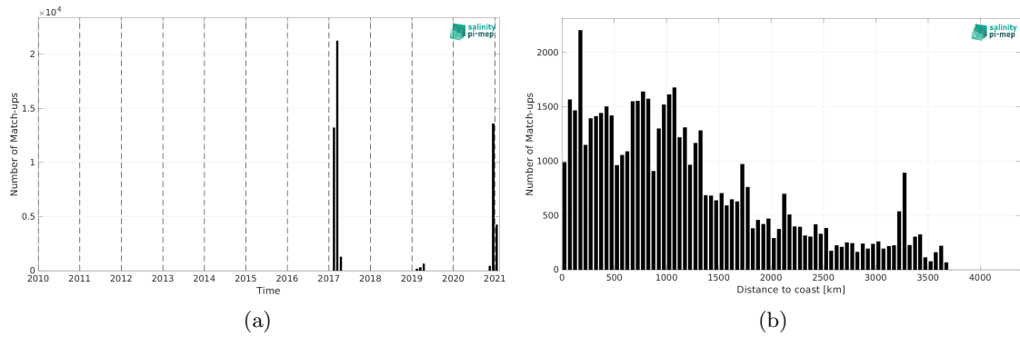
Figure 2: Number of match-ups between TSG (GOSUD-Sailing-ship) and SMAP SSS L3 v5.0 - 8-Day running (JPL) SSS as a function of time (a) and as function of the distance to coast (b) over the Roaring Forties and Furious Fifties Pi-MEP region and for the full satellite product period.
