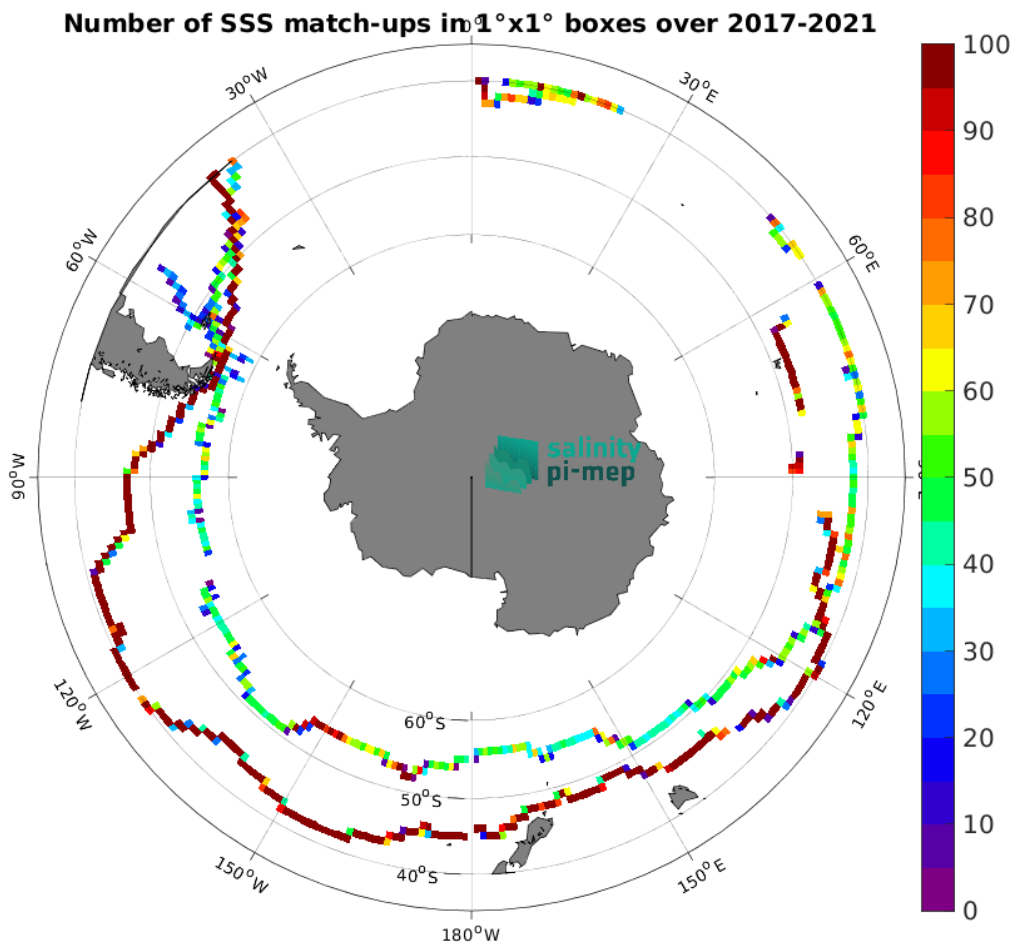
Figure 5: Number of SSS match-ups between TSG (GOSUD-Sailing-ship) SSS and the SMAP SSS L3 v5.0 - 8-Day running (JPL) SSS product for the Roaring Forties and Furious Fifties Pi-MEP region over 1^\circ \times 1^\circ boxes and for the full satellite product period.
