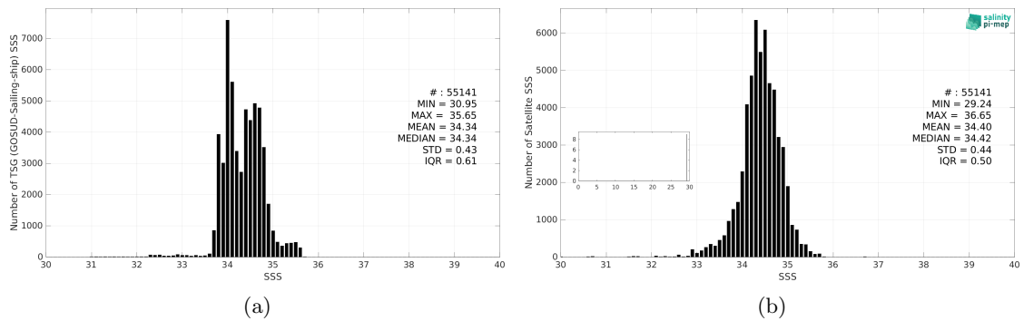
Figure 3: Histograms of SSS from TSG (GOSUD-Sailing-ship) (a) and SMAP SSS L3 v5.0 - 8-Day running (JPL) (b) considering all match-up pairs per bins of 0.1 over the Roaring Forties and Furious Fifties Pi-MEP region and for the full satellite product period.
