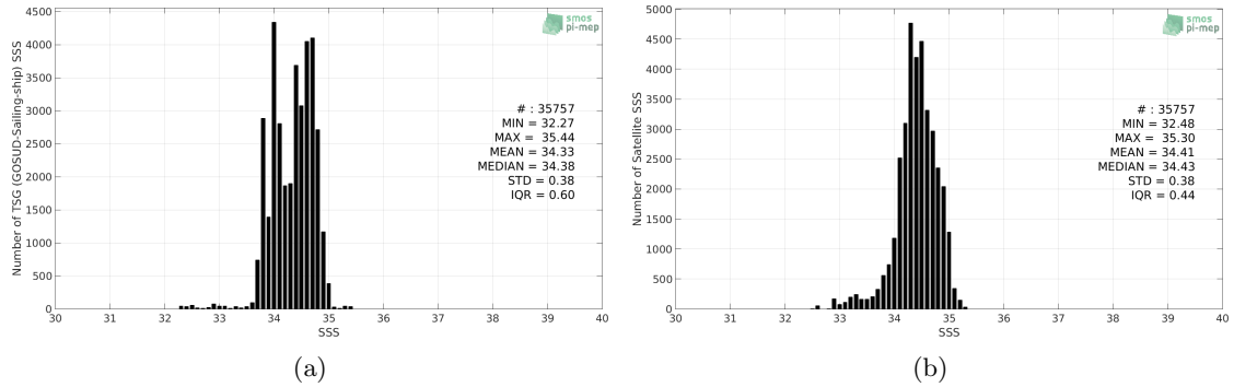
Figure 2: Histograms of SSS from TSG (GOSUD-Sailing-ship) (a) and SMAP SSS L3 v5.0 - 8-Day running (JPL) (b) considering all match-up pairs per bins of 0.1 over the Roaring Forties and Furious Fifties Pi-MEP region and for the full satellite product period.
