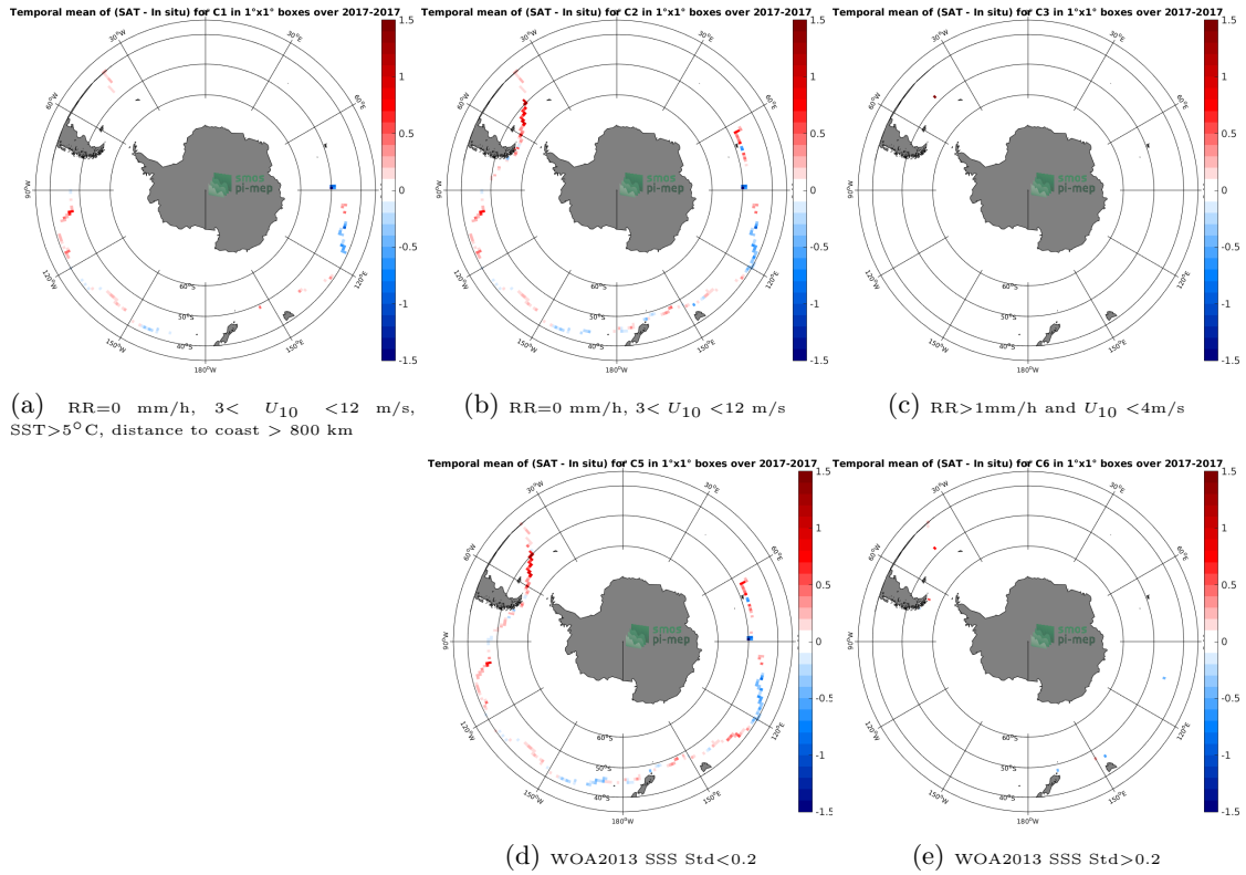
Figure 12: Temporal mean gridded over spatial boxes of size 1^\circ \times 1^\circ of \Delta SSS (SMAP SSS L3 v5.0 - 8-Day running (JPL) - TSG (GOSUD-Sailing-ship)) for 5 different subdatasets corresponding to: RR=0 mm/h, 3 < U_{10} < 12 m/s, SST>5°C, distance to coast > 800 km (a), RR=0 mm/h, 3 < U_{10} < 12 m/s (b), RR>1mm/h and U_{10} < 4 m/s (c), WOA2013 SSS Std<0.2 (d), WOA2013 SSS Std>0.2 (e).
