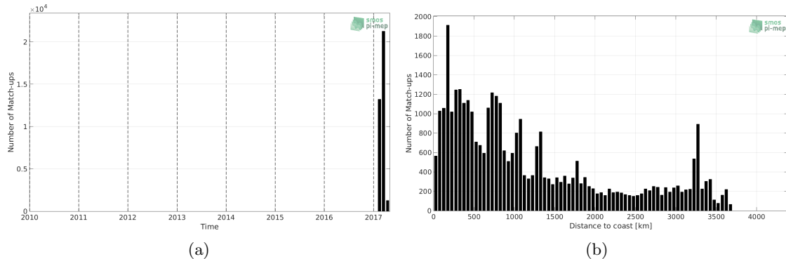
Figure 1: Number of match-ups between TSG (GOSUD-Sailing-ship) and SMAP SSS L3 v5.0 - 8-Day running (JPL) SSS as a function of time (a) and as function of the distance to coast (b) over the Roaring Forties and Furious Fifties Pi-MEP region and for the full satellite product period.
