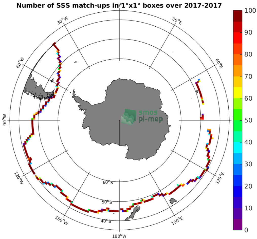
Figure 4: Number of SSS match-ups between TSG (GOSUD-Sailing-ship) SSS and the SMAP SSS L3 v5.0 - 8-Day running (JPL) SSS product for the Roaring Forties and Furious Fifties Pi-MEP region over 1^\circ \times 1^\circ boxes and for the full satellite product period.
