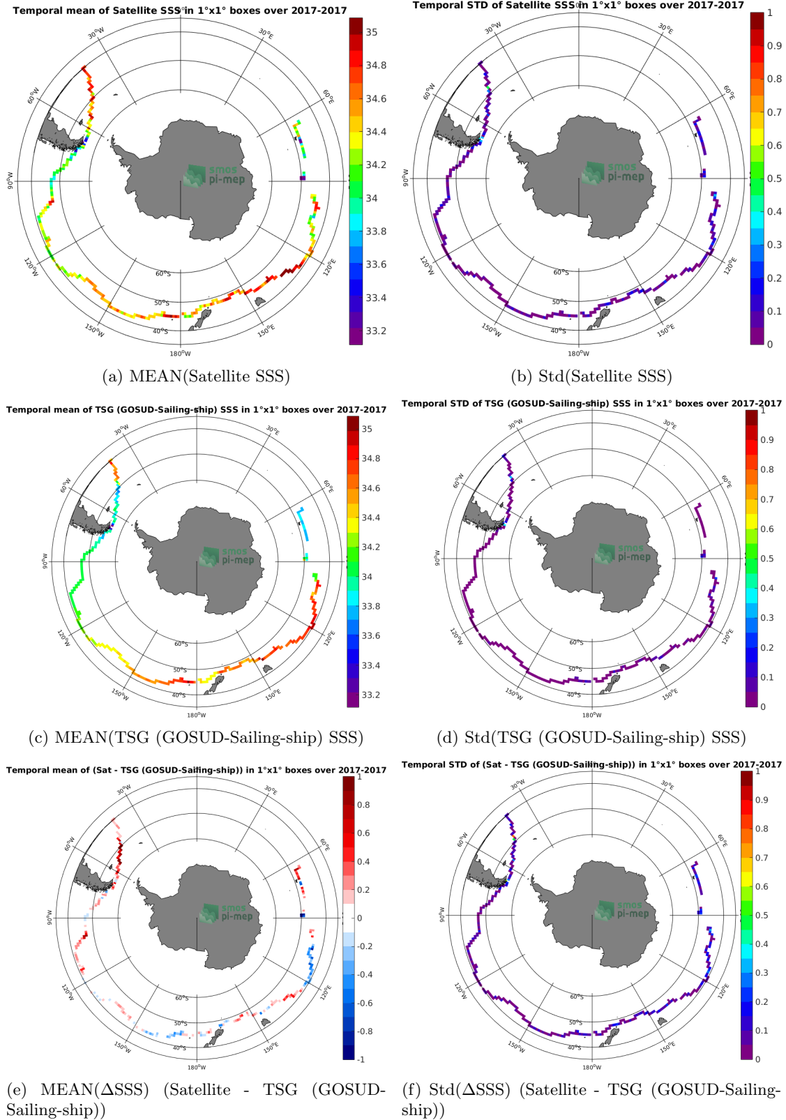
Figure 6: Temporal mean (left) and Std (right), of SSS from SMAP SSS L3 v5.0 - 8-Day running (JPL) (top), TSG (GOSUD-Sailing-ship) (middle), and of \Delta SSS (Satellite - TSG (GOSUD-Sailing-ship)). Only match-up pairs are used to generate these maps.
