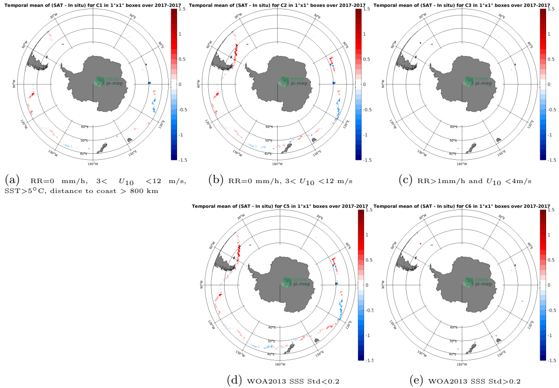
Figure 12: Temporal mean gridded over spatial boxes of size 1°x1° of \Delta SSS (SMAP SSS L3 v5.0 - 8-Day running (JPL) - TSG (GOSUD-Sailing-ship)) for 5 different subdatasets corresponding to:RR=0 mm/h, 3 < U_{10} < 12 m/s, SST>5°C, distance to coast > 800 km (a), RR=0 mm/h, 3 < U_{10} < 12 m/s (b), RR>1mm/h and U_{10} < 4 m/s (c), WOA2013 SSS Std<0.2 (d), WOA2013 SSS Std>0.2 (e).
