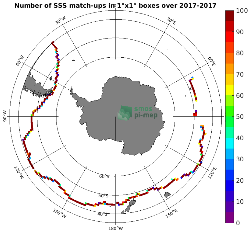
Figure 4: Number of SSS match-ups between TSG (GOSUD-Sailing-ship) SSS and the SMAP SSS L3 v5.0 - 8-Day running (JPL) SSS product for the Roaring Forties and Furious Fifties Pi-MEP region over 1^\circ \times 1^\circ boxes and for the full satellite product period.
