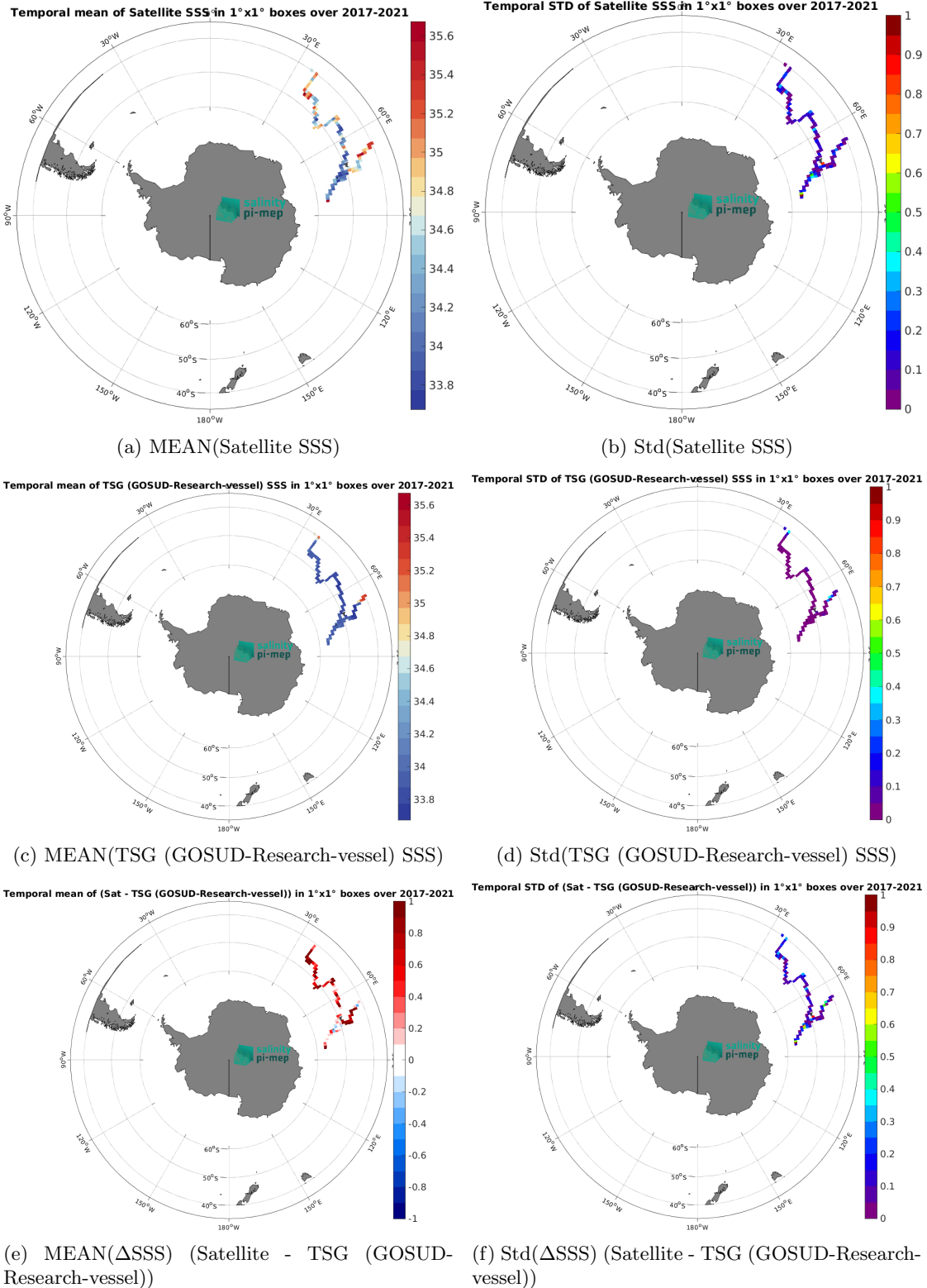
Figure 7: Temporal mean (left) and Std (right) of SSS from SMAP SSS L3 v5.0 - 8-Day running (JPL) (top), TSG (GOSUD-Research-vessel) (middle), and of \Delta SSS (Satellite - TSG (GOSUD-Research-vessel)). Only match-up pairs are used to generate these maps.
