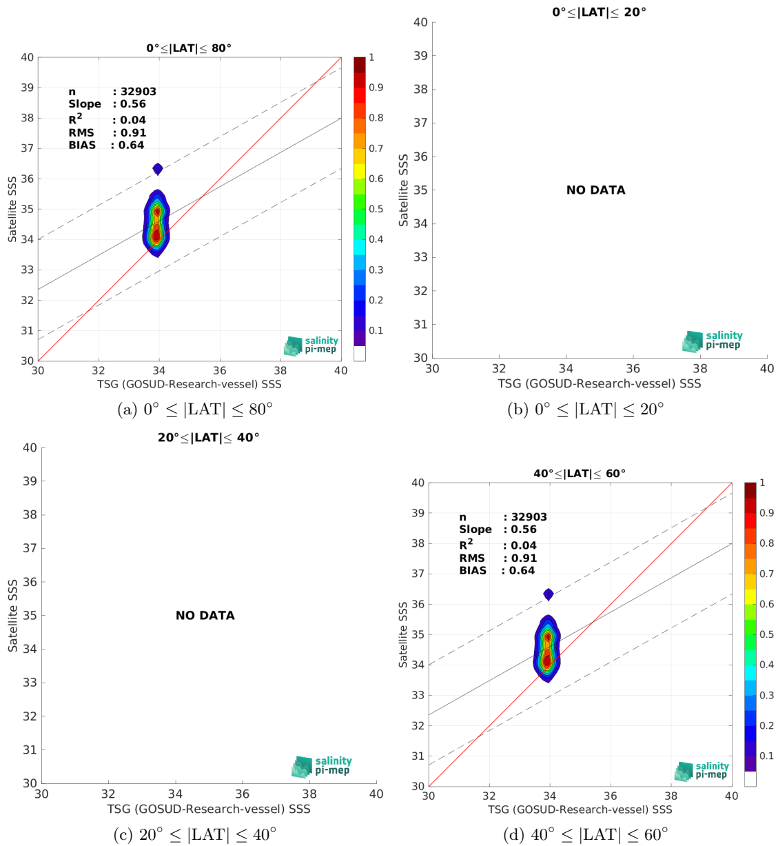
Figure 10: Contour maps of the concentration of SMAP SSS L3 v5.0 - 8-Day running (JPL) SSS (y-axis) versus TSG (GOSUD-Research-vessel) SSS (x-axis) at match-up pairs for different latitude bands. For each plot, the red line shows x=y . The black thin and dashed lines indicate a linear fit through the data cloud and the \pm 95\% confidence levels, respectively. The number match-up pairs n , the slope and R^2 coefficient of the linear fit, the root mean square (RMS) and the mean bias between satellite and in situ data are indicated for each latitude band in each plots.
