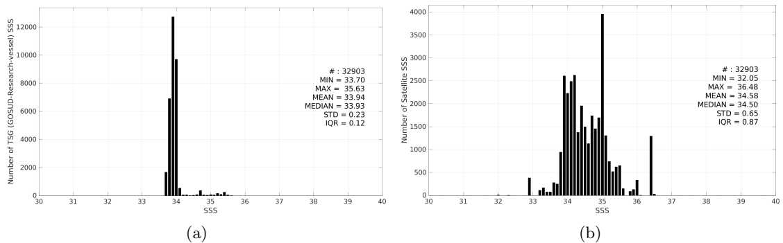
Figure 3: Histograms of SSS from TSG (GOSUD-Research-vessel) (a) and SMAP SSS L3 v5.0 - 8-Day running (JPL) (b) considering all match-up pairs per bins of 0.1 over the Roaring Forties and Furious Fifties Pi-MEP region and for the full satellite product period.
