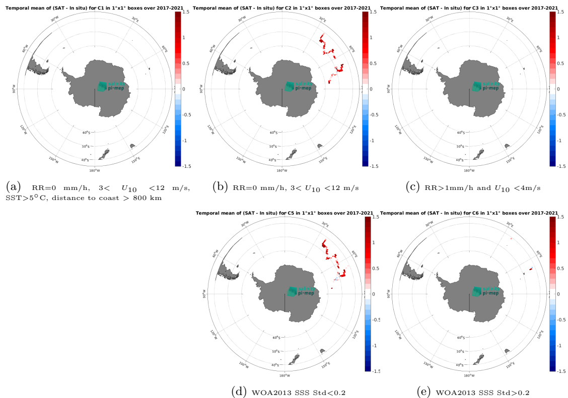
Figure 14: Temporal mean gridded over spatial boxes of size 1^\circ \times 1^\circ of \Delta SSS (SMAP SSS L3 v5.0 - 8-Day running (JPL) - TSG (GOSUD-Research-vessel)) for 5 different subdatasets corresponding to:RR=0 mm/h, 3 < U_{10} < 12 m/s, SST>5°C, distance to coast > 800 km (a), RR=0 mm/h, 3 < U_{10} < 12 m/s (b), RR>1mm/h and U_{10} < 4 m/s (c), WOA2013 SSS Std<0.2 (d), WOA2013 SSS Std>0.2 (e).
