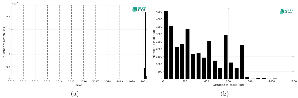
Figure 2: Number of match-ups between TSG (GOSUD-Research-vessel) and SMAP SSS L3 v5.0 - 8-Day running (JPL) SSS as a function of time (a) and as function of the distance to coast (b) over the Roaring Forties and Furious Fifties Pi-MEP region and for the full satellite product period.
