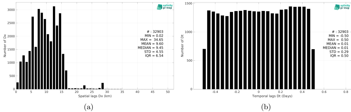
Figure 6: Histograms of the spatial (a) and temporal (b) lags between the location/time of the TSG (GOSUD-Research-vessel) measurement and the date of the corresponding SMAP SSS L3 v5.0 - 8-Day running (JPL) SSS pixel.
