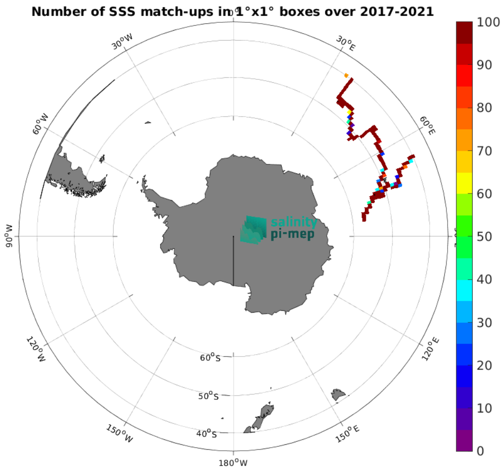
Figure 5: Number of SSS match-ups between TSG (GOSUD-Research-vessel) SSS and the SMAP SSS L3 v5.0 - 8-Day running (JPL) SSS product for the Roaring Forties and Furious Fifties Pi-MEP region over 1^\circ \times 1^\circ boxes and for the full satellite product period.
