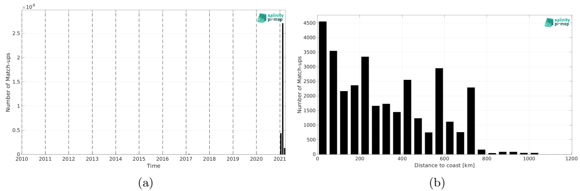
Figure 1: Number of match-ups between TSG (GOSUD-Research-vessel) and SMAP SSS L3 v5.0 - 8-Day running (JPL) SSS as a function of time (a) and as function of the distance to coast (b) over the Roaring Forties and Furious Fifties Pi-MEP region and for the full satellite product period.
