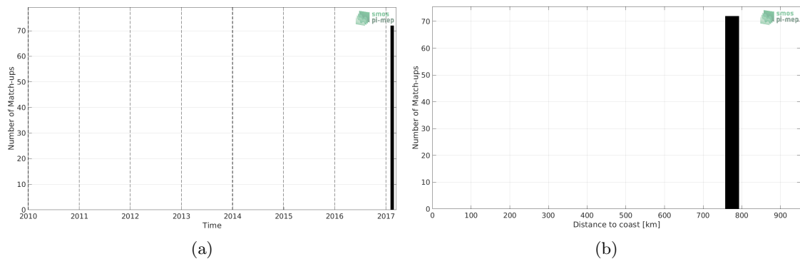
Figure 1: Number of match-ups between TSG (GOSUD-Research-vessel) and SMAP SSS L3 v5.0 - 8-Day running (JPL) SSS as a function of time (a) and as function of the distance to coast (b) over the Roaring Forties and Furious Fifties Pi-MEP region and for the full satellite product period.
