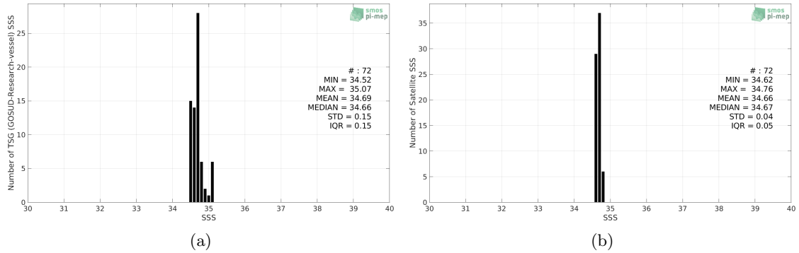
Figure 2: Histograms of SSS from TSG (GOSUD-Research-vessel) (a) and SMAP SSS L3 v5.0 - 8-Day running (JPL) (b) considering all match-up pairs per bins of 0.1 over the Roaring Forties and Furious Fifties Pi-MEP region and for the full satellite product period.
