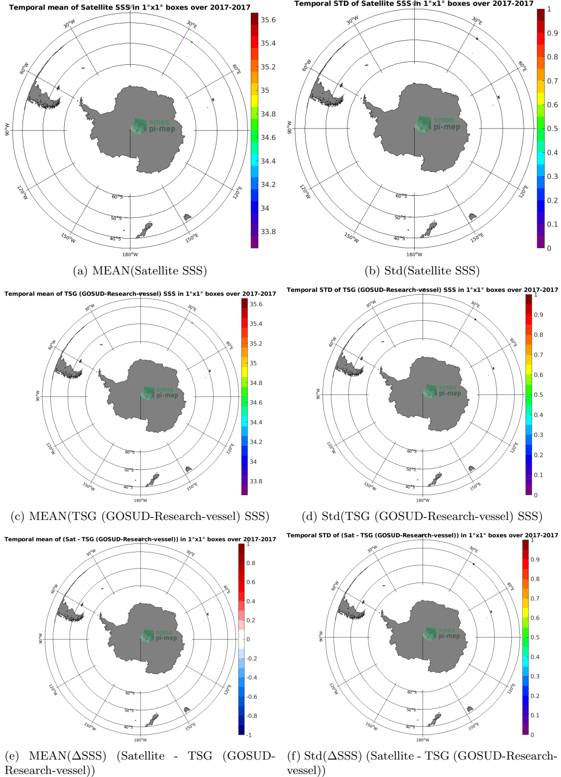
Figure 6: Temporal mean (left) and Std (right) of SSS from SMAP SSS L3 v5.0 - 8-Day running (JPL) (top), TSG (GOSUD-Research-vessel) (middle), and of \Delta SSS (Satellite - TSG (GOSUD-Research-vessel)). Only match-up pairs are used to generate these maps.
