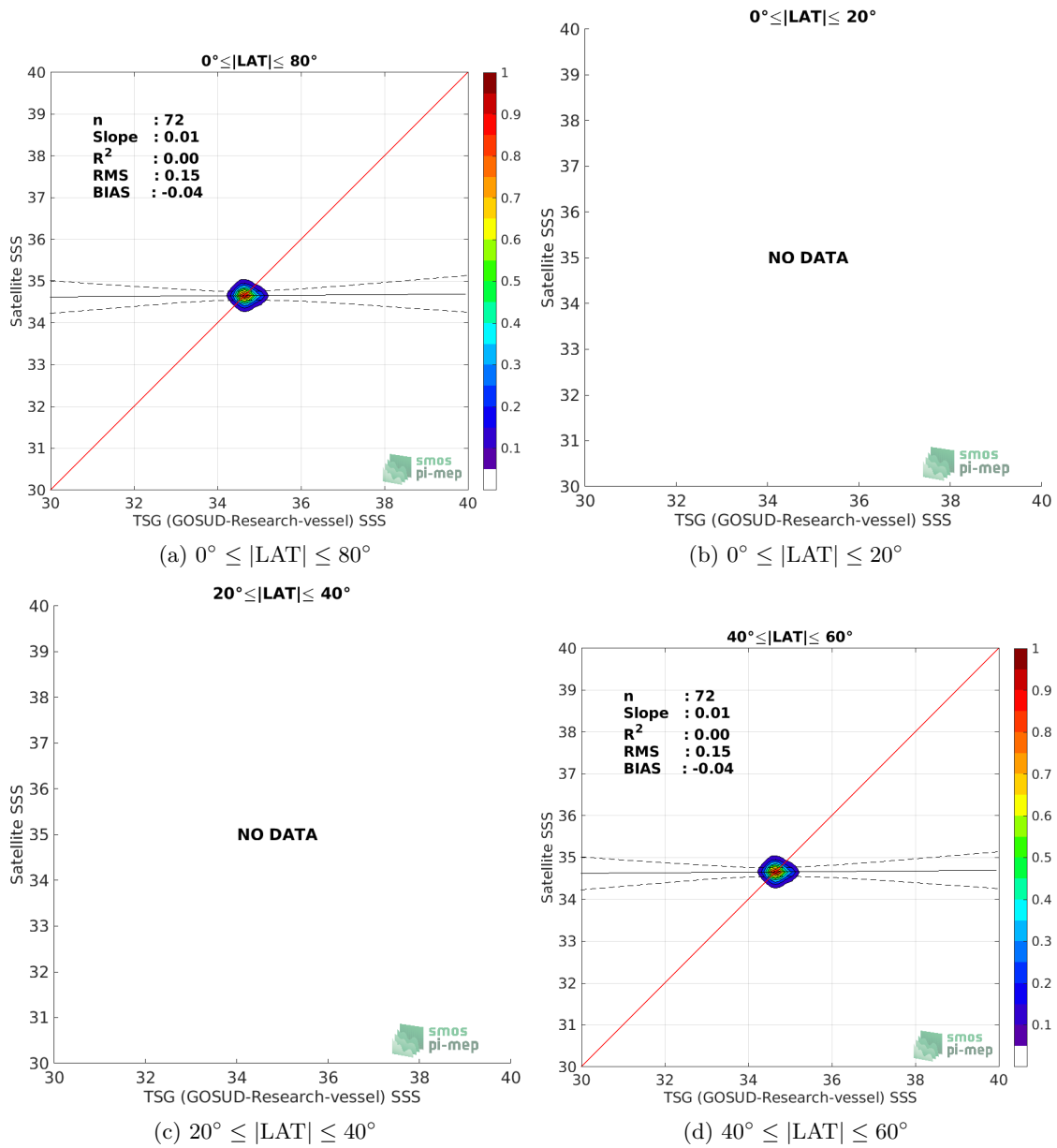
Figure 9: Contour maps of the concentration of SMAP SSS L3 v5.0 - 8-Day running (JPL) SSS (y-axis) versus TSG (GOSUD-Research-vessel) SSS (x-axis) at match-up pairs for different latitude bands. For each plot, the red line shows x=y . The black thin and dashed lines indicate a linear fit through the data cloud and the \pm 95\% confidence levels, respectively. The number match-up pairs n , the slope and R^2 coefficient of the linear fit, the root mean square (RMS) and the mean bias between satellite and in situ data are indicated for each latitude band in each plots.
