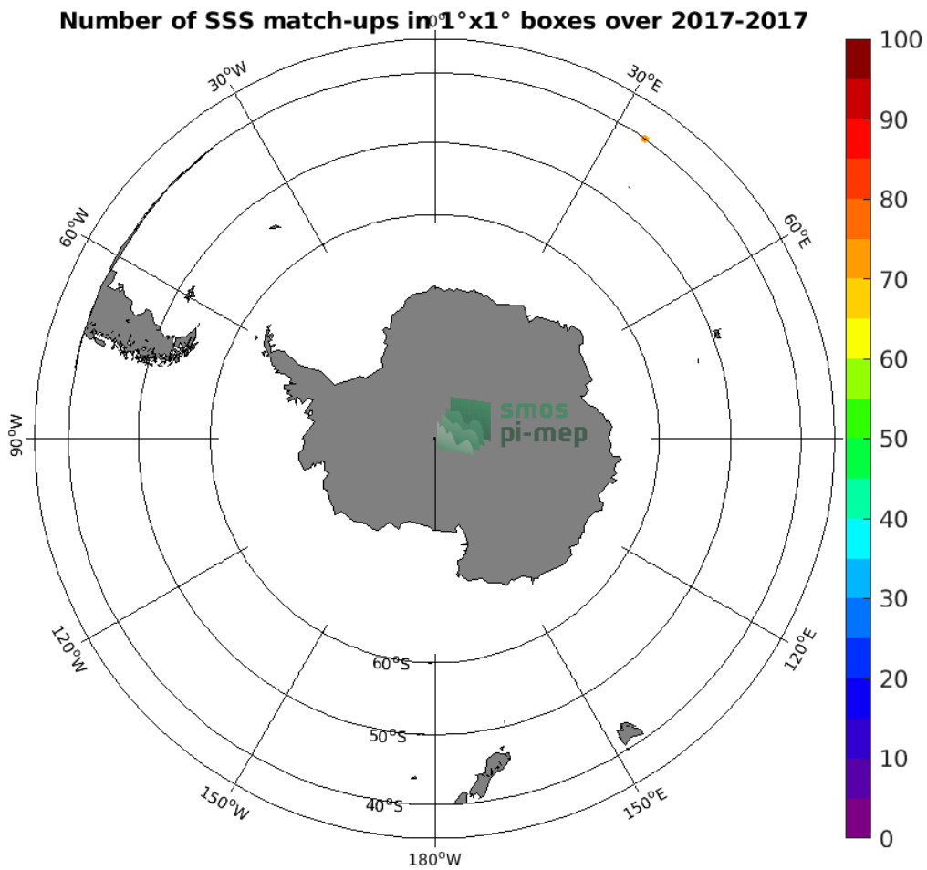
Figure 4: Number of SSS match-ups between TSG (GOSUD-Research-vessel) SSS and the SMAP SSS L3 v5.0 - 8-Day running (JPL) SSS product for the Roaring Forties and Furious Fifties Pi-MEP region over 1^\circ \times 1^\circ boxes and for the full satellite product period.
