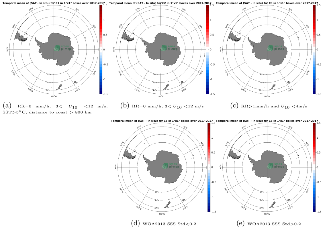
Figure 12: Temporal mean gridded over spatial boxes of size 1°x1° of \Delta SSS (SMAP SSS L3 v5.0 - 8-Day running (JPL) - TSG (GOSUD-Research-vessel)) for 5 different subdatasets corresponding to:RR=0 mm/h, 3 < U_{10} < 12 m/s, SST>5°C, distance to coast > 800 km (a), RR=0 mm/h, 3 < U_{10} < 12 m/s (b), RR>1mm/h and U_{10} < 4 m/s (c), WOA2013 SSS Std<0.2 (d), WOA2013 SSS Std>0.2 (e).
