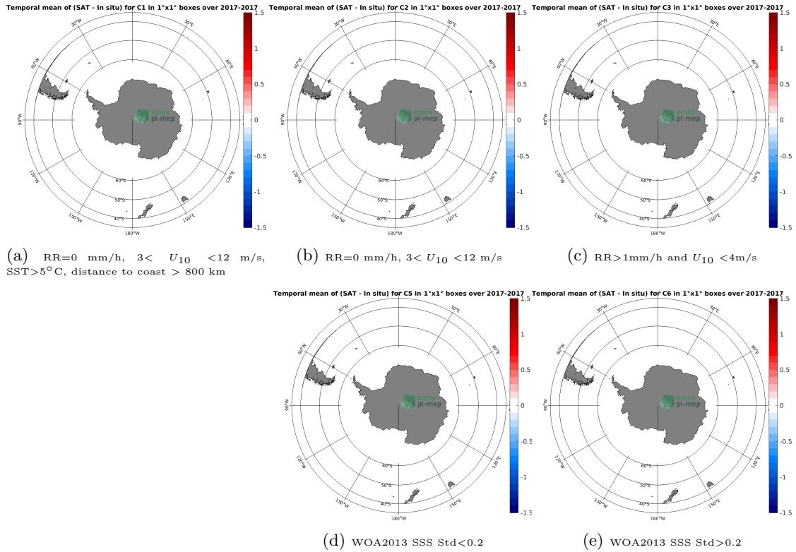
Figure 12: Temporal mean gridded over spatial boxes of size 1°x1° of \Delta SSS (SMAP SSS L3 v5.0 - 8-Day running (JPL) - TSG (GOSUD-Research-vessel)) for 5 different subdatasets corresponding to: RR=0 mm/h, 3 < U_{10} < 12 m/s, SST > 5°C, distance to coast > 800 km (a), RR=0 mm/h, 3 < U_{10} < 12 m/s (b), RR > 1mm/h and U_{10} < 4 m/s (c), WOA2013 SSS Std < 0.2 (d), WOA2013 SSS Std > 0.2 (e).
