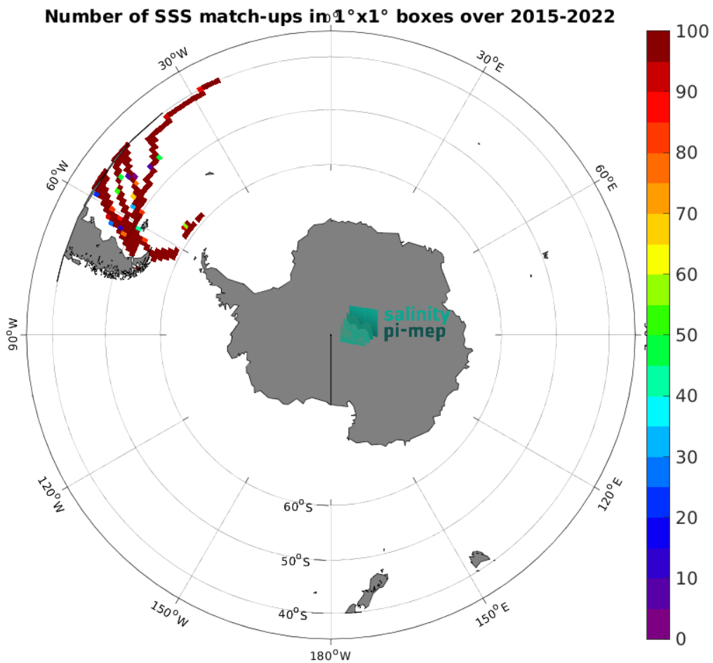
Figure 5: Number of SSS match-ups between TSG (CSIC-UTM) SSS and the SMAP SSS L3 v5.0 - 8-Day running (JPL) SSS product for the Roaring Forties and Furious Fifties Pi-MEP region over 1^\circ \times 1^\circ boxes and for the full satellite product period.
