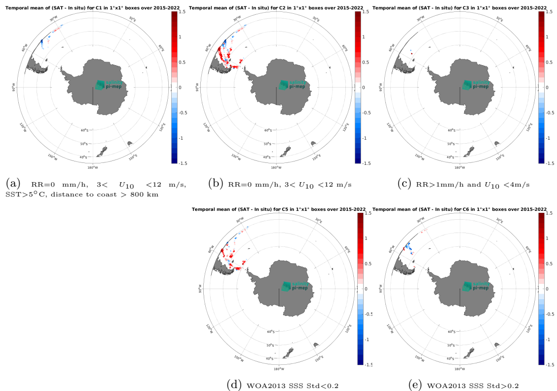
Figure 14: Temporal mean gridded over spatial boxes of size 1^\circ \times 1^\circ of \Delta SSS (SMAP SSS L3 v5.0 - 8-Day running (JPL) - TSG (CSIC-UTM)) for 5 different subdatasets corresponding to:RR=0 mm/h, 3 < U_{10} < 12 m/s, SST > 5^\circ\text{C} , distance to coast > 800 km (a), RR=0 mm/h, 3 < U_{10} < 12 m/s (b), RR > 1 mm/h and U_{10} < 4 m/s (c), WOA2013 SSS Std < 0.2 (d), WOA2013 SSS Std > 0.2 (e).
