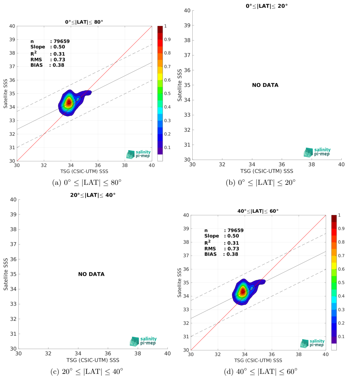
Figure 10: Contour maps of the concentration of SMAP SSS L3 v5.0 - 8-Day running (JPL) SSS (y-axis) versus TSG (CSIC-UTM) SSS (x-axis) at match-up pairs for different latitude bands. For each plot, the red line shows x=y . The black thin and dashed lines indicate a linear fit through the data cloud and the \pm 95\% confidence levels, respectively. The number match-up pairs n , the slope and R^2 coefficient of the linear fit, the root mean square (RMS) and the mean bias between satellite and in situ data are indicated for each latitude band in each plots.
