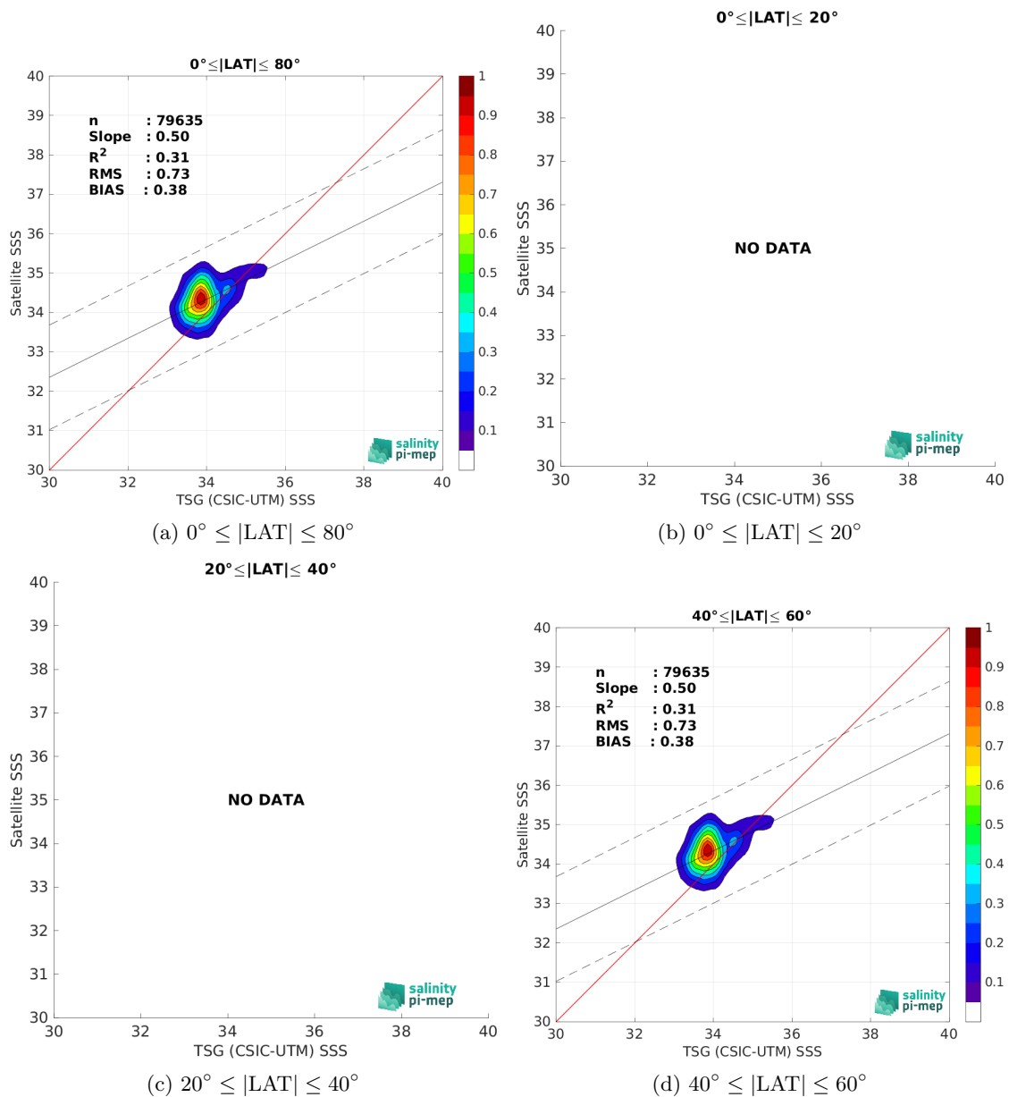
Figure 9: Contour maps of the concentration of SMAP SSS L3 v5.0 - 8-Day running (JPL) SSS (y-axis) versus TSG (CSIC-UTM) SSS (x-axis) at match-up pairs for different latitude bands. For each plot, the red line shows x=y . The black thin and dashed lines indicate a linear fit through the data cloud and the \pm 95\% confidence levels, respectively. The number match-up pairs n , the slope and R^2 coefficient of the linear fit, the root mean square (RMS) and the mean bias between satellite and in situ data are indicated for each latitude band in each plots.
