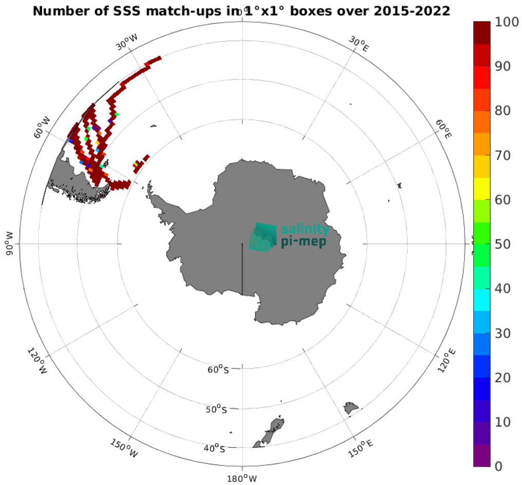
Figure 4: Number of SSS match-ups between TSG (CSIC-UTM) SSS and the SMAP SSS L3 v5.0 - 8-Day running (JPL) SSS product for the Roaring Forties and Furious Fifties Pi-MEP region over 1^\circ \times 1^\circ boxes and for the full satellite product period.
