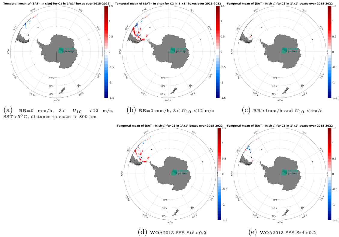
Figure 12: Temporal mean gridded over spatial boxes of size 1^{\circ}\times 1^{\circ} of \Delta\text{SSS} (SMAP SSS L3 v5.0 - 8-Day running (JPL) - TSG (CSIC-UTM)) for 5 different subdatasets corresponding to:RR=0 mm/h, 3 < U_{10} < 12 m/s, SST >5^{\circ}\text{C} , distance to coast > 800 km (a), RR=0 mm/h, 3 < U_{10} < 12 m/s (b), RR >1 mm/h and U_{10} < 4 m/s (c), WOA2013 SSS Std <0.2 (d), WOA2013 SSS Std >0.2 (e).
