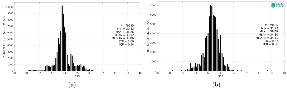
Figure 2: Histograms of SSS from TSG (CSIC-UTM) (a) and SMAP SSS L3 v5.0 - 8-Day running (JPL) (b) considering all match-up pairs per bins of 0.1 over the Roaring Forties and Furious Fifties Pi-MEP region and for the full satellite product period.
