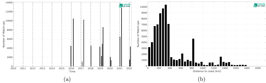
Figure 1: Number of match-ups between TSG (CSIC-UTM) and SMAP SSS L3 v5.0 - 8-Day running (JPL) SSS as a function of time (a) and as function of the distance to coast (b) over the Roaring Forties and Furious Fifties Pi-MEP region and for the full satellite product period.
