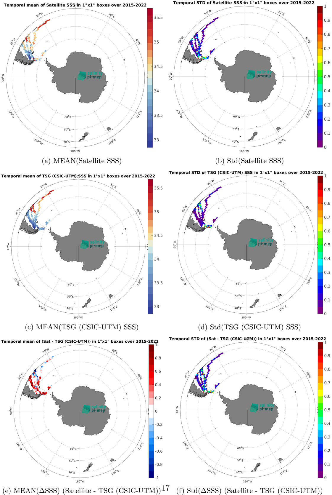
Figure 6: Temporal mean (left) and Std (right) of SSS from SMAP SSS L3 v5.0 - 8-Day running (JPL) (top), TSG (CSIC-UTM) (middle), and of \Delta SSS (Satellite - TSG (CSIC-UTM)). Only match-up pairs are used to generate these maps.
