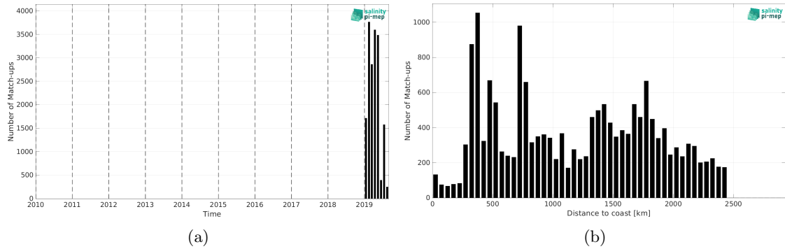
Figure 2: Number of match-ups between Saildrone and SMAP SSS L3 v5.0 - 8-Day running (JPL) SSS as a function of time (a) and as function of the distance to coast (b) over the Roaring Forties and Furious Fifties Pi-MEP region and for the full satellite product period.
