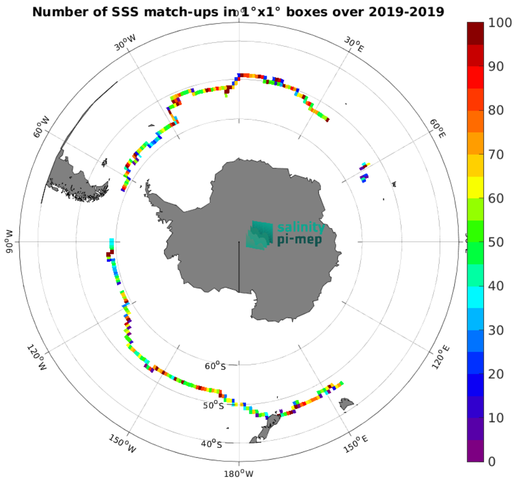
Figure 5: Number of SSS match-ups between Saildrone SSS and the SMAP SSS L3 v5.0 - 8-Day running (JPL) SSS product for the Roaring Forties and Furious Fifties Pi-MEP region over 1^\circ \times 1^\circ boxes and for the full satellite product period.
