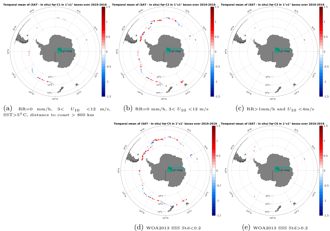
Figure 14: Temporal mean gridded over spatial boxes of size 1^\circ \times 1^\circ of \Delta SSS (SMAP SSS L3 v5.0 - 8-Day running (JPL) - Saicdrone) for 5 different subdatasets corresponding to:RR=0 mm/h, 3 < U_{10} < 12 m/s, SST > 5°C, distance to coast > 800 km (a), RR=0 mm/h, 3 < U_{10} < 12 m/s (b), RR > 1mm/h and U_{10} < 4 m/s (c), WOA2013 SSS Std < 0.2 (d), WOA2013 SSS Std > 0.2 (e).
