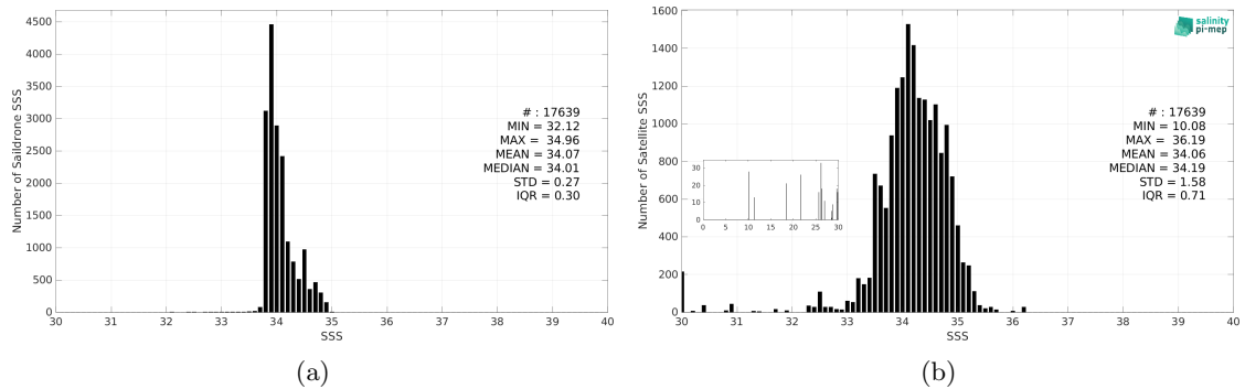
Figure 3: Histograms of SSS from Saildrone (a) and SMAP SSS L3 v5.0 - 8-Day running (JPL) (b) considering all match-up pairs per bins of 0.1 over the Roaring Forties and Furious Fifties Pi-MEP region and for the full satellite product period.
