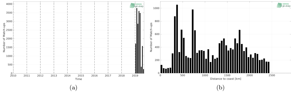
Figure 1: Number of match-ups between Sairdron and SMAP SSS L3 v5.0 - 8-Day running (JPL) SSS as a function of time (a) and as function of the distance to coast (b) over the Roaring Forties and Furious Fifties Pi-MEP region and for the full satellite product period.
