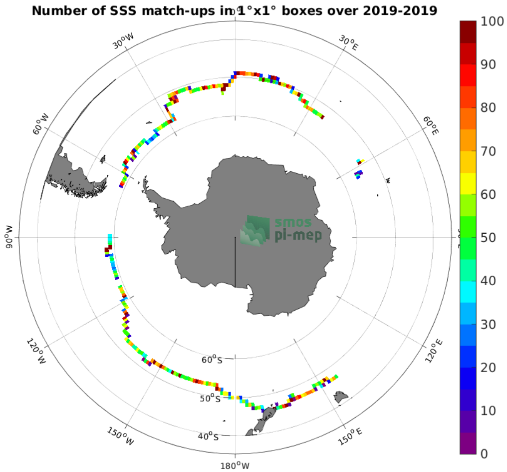
Figure 4: Number of SSS match-ups between Sailldrone SSS and the SMAP SSS L3 v5.0 - 8-Day running (JPL) SSS product for the Roaring Forties and Furious Fifties Pi-MEP region over 1^\circ \times 1^\circ boxes and for the full satellite product period.
