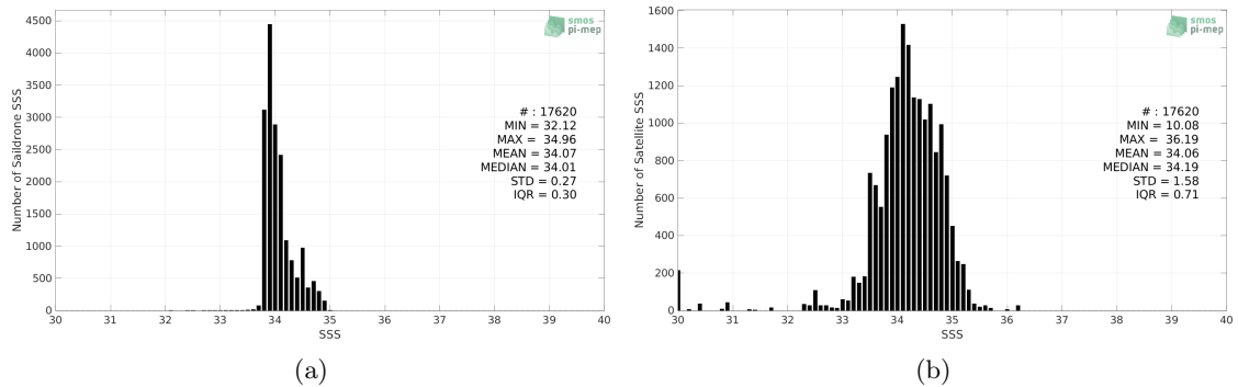
Figure 2: Histograms of SSS from Sairdron (a) and SMAP SSS L3 v5.0 - 8-Day running (JPL) (b) considering all match-up pairs per bins of 0.1 over the Roaring Forties and Furious Fifties Pi-MEP region and for the full satellite product period.
