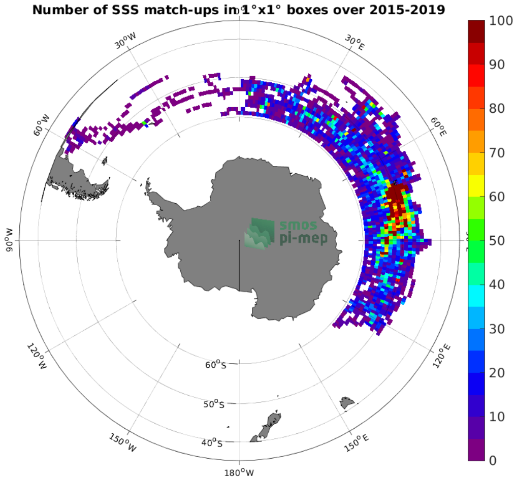
Figure 4: Number of SSS match-ups between Marine mammals SSS and the SMAP SSS L3 v5.0 - 8-Day running (JPL) SSS product for the Roaring Forties and Furious Fifties Pi-MEP region over 1^\circ \times 1^\circ boxes and for the full satellite product period.
