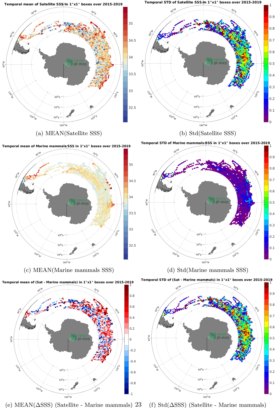
Figure 6: Temporal mean (left) and Std (right) of SSS from SMAP SSS L3 v5.0 - 8-Day running (JPL) (top), Marine mammals (middle), and of \Delta SSS (Satellite - Marine mammals). Only match-up pairs are used to generate these maps.
