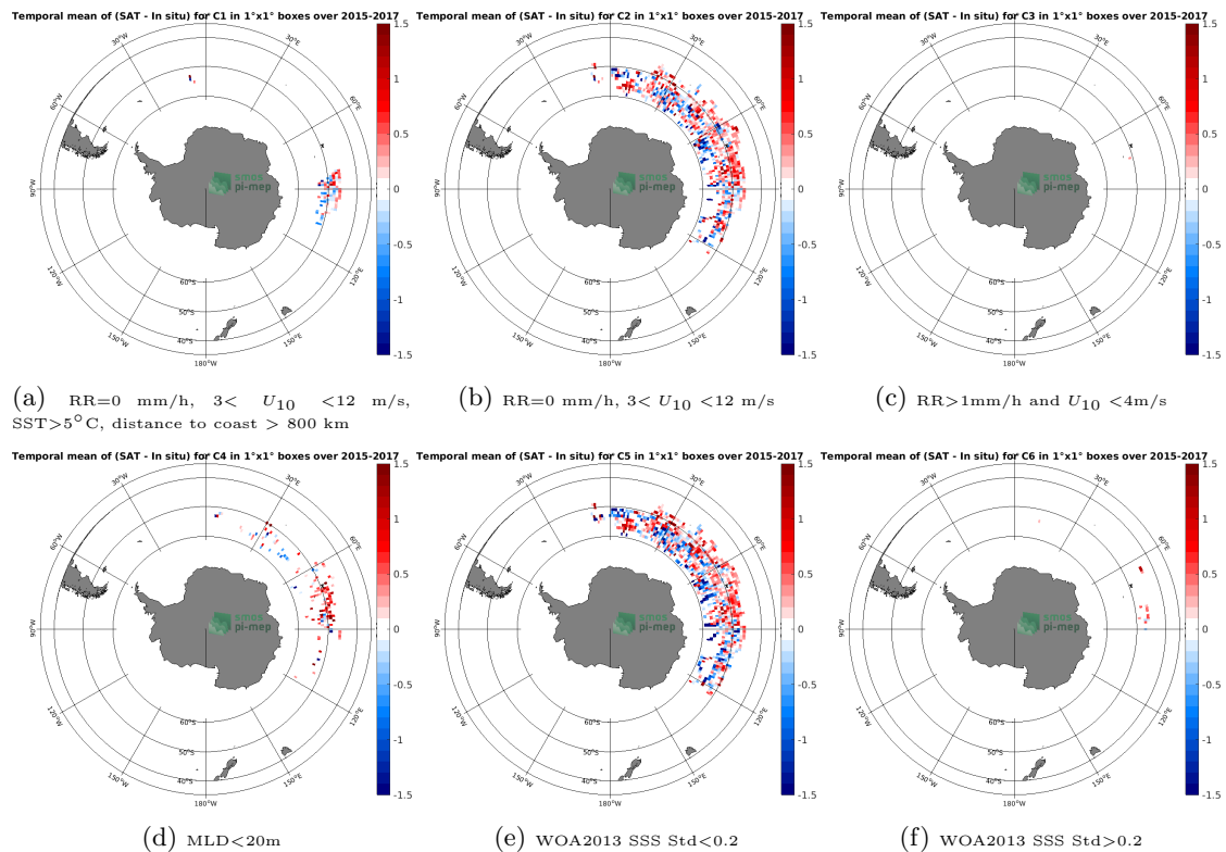
Figure 12: Temporal mean gridded over spatial boxes of size 1^{\circ}\times 1^{\circ} of \Delta\text{SSS} (SMAP SSS L3 v5.0 - 8-Day running (JPL) - Sea mammals) for 6 different subdatasets corresponding to:RR=0 mm/h, 3 < U_{10} < 12 m/s, SST >5^{\circ}\text{C} , distance to coast > 800 km (a), RR=0 mm/h, 3 < U_{10} < 12 m/s (b), RR >1 mm/h and U_{10} < 4 m/s (c),MLD <20 m (d),WOA2013 SSS Std <0.2 (e),WOA2013 SSS Std >0.2 (f).
