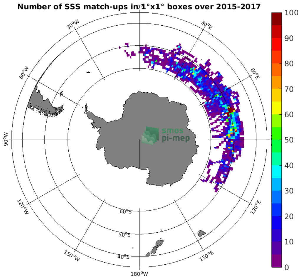
Figure 4: Number of SSS match-ups between Sea mammals SSS and the SMAP SSS L3 v5.0 - 8-Day running (JPL) SSS product for the Roaring Forties and Furious Fifties Pi-MEP region over 1^\circ \times 1^\circ boxes and for the full satellite product period.
