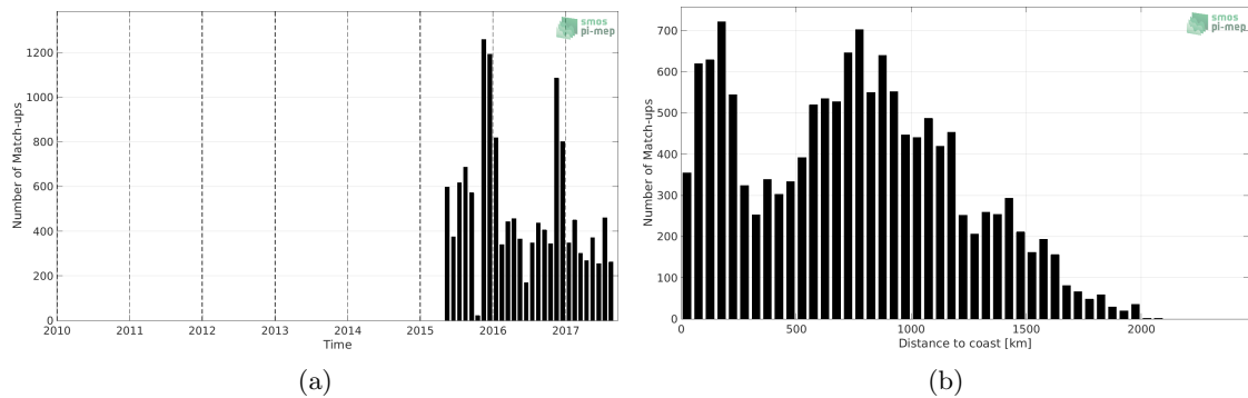
Figure 1: Number of match-ups between Sea mammals and SMAP SSS L3 v5.0 - 8-Day running (JPL) SSS as a function of time (a) and as function of the distance to coast (b) over the Roaring Forties and Furious Fifties Pi-MEP region and for the full satellite product period.
