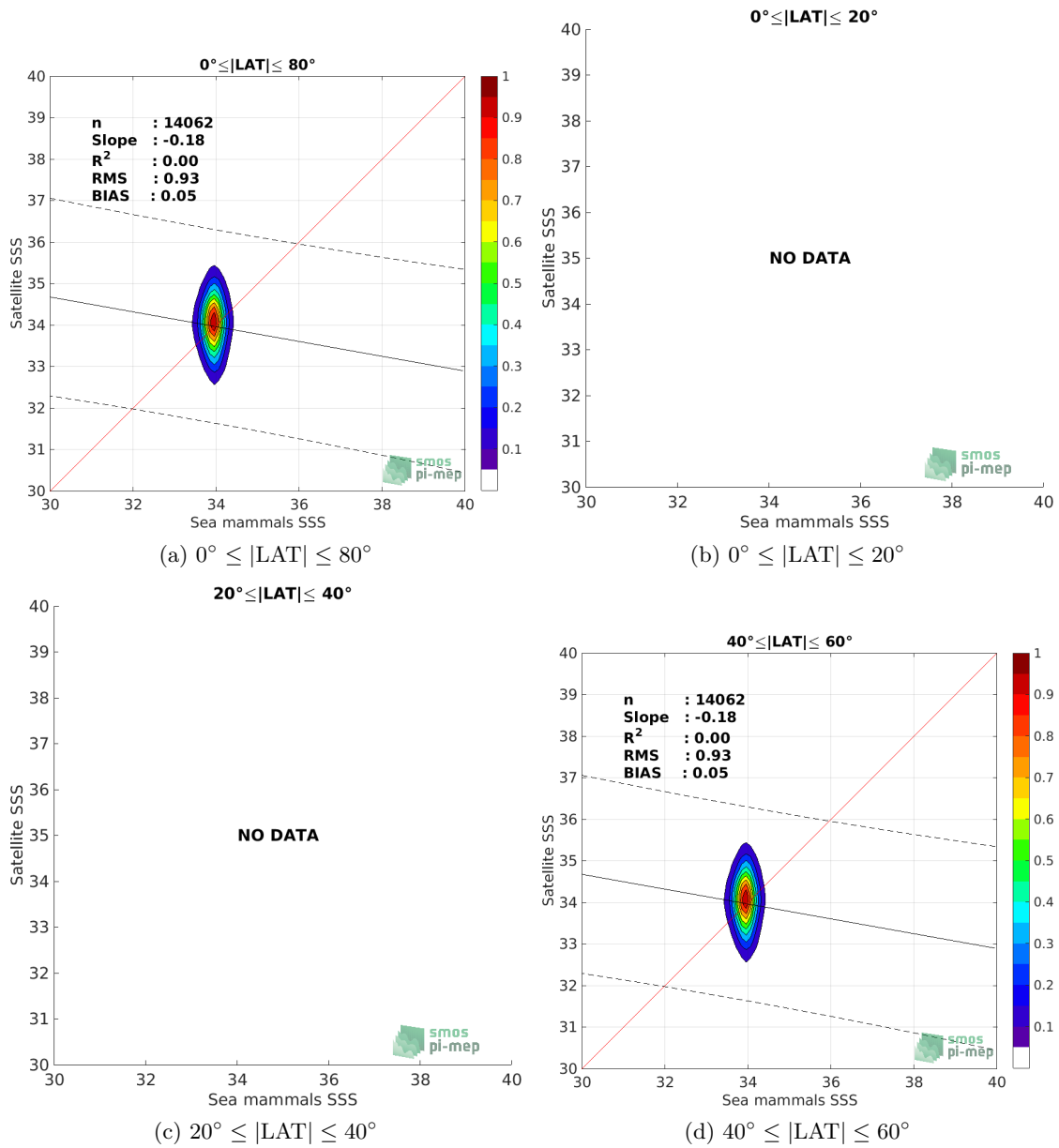
Figure 9: Contour maps of the concentration of SMAP SSS L3 v5.0 - 8-Day running (JPL) SSS (y-axis) versus Sea mammals SSS (x-axis) at match-up pairs for different latitude bands. For each plot, the red line shows x=y . The black thin and dashed lines indicate a linear fit through the data cloud and the \pm 95\% confidence levels, respectively. The number match-up pairs n , the slope and R^2 coefficient of the linear fit, the root mean square (RMS) and the mean bias between satellite and in situ data are indicated for each latitude band in each plots.
