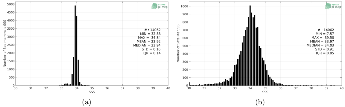
Figure 2: Histograms of SSS from Sea mammals (a) and SMAP SSS L3 v5.0 - 8-Day running (JPL) (b) considering all match-up pairs per bins of 0.1 over the Roaring Forties and Furious Fifties Pi-MEP region and for the full satellite product period.
