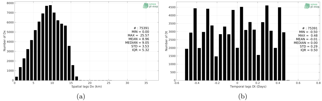
Figure 4: Histograms of the spatial (a) and temporal (b) lags between the time of the Surface drifters measurements and the date of the corresponding SMAP SSS L3 v5.0 - 8-Day running (JPL) SSS product.
