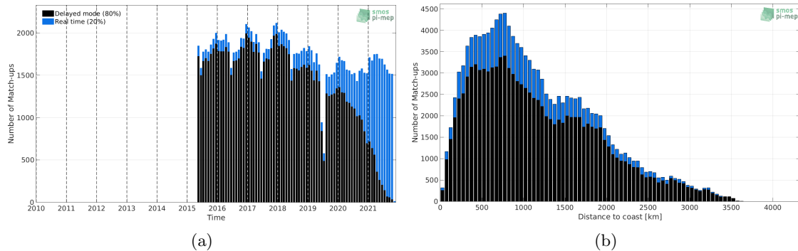
Figure 1: Number of match-ups between Argo and SMAP SSS L3 v5.0 - 8-Day running (JPL) SSS as a function of time (a) and as function of the distance to coast (b) over the Roaring Forties and Furious Fifties Pi-MEP region and for the full satellite product period.
