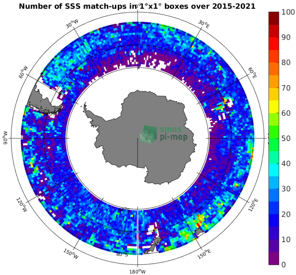
Figure 4: Number of SSS match-ups between Argo SSS and the SMAP SSS L3 v5.0 - 8-Day running (JPL) SSS product for the Roaring Forties and Furious Fifties Pi-MEP region over 1^\circ \times 1^\circ boxes and for the full satellite product period.
