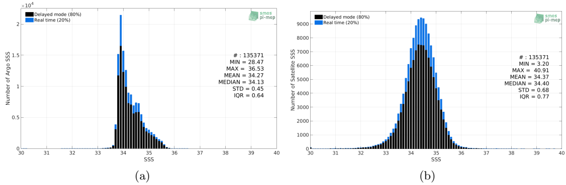
Figure 2: Histograms of SSS from Argo (a) and SMAP SSS L3 v5.0 - 8-Day running (JPL) (b) considering all match-up pairs per bins of 0.1 over the Roaring Forties and Furious Fifties Pi-MEP region and for the full satellite product period.
