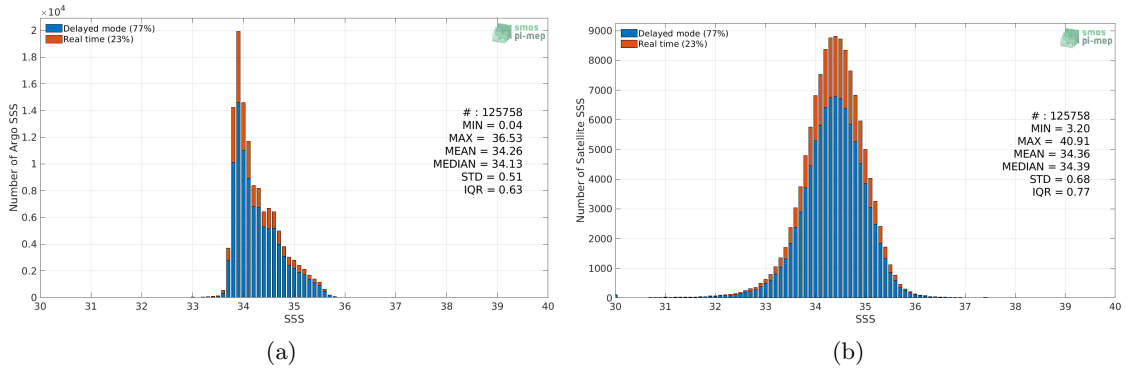
Figure 2: Histograms of SSS from Argos (a) and SMAP SSS L3 v5.0 - 8-Day running (JPL) (b) considering all match-up pairs per bins of 0.1 over the Roaring Forties and Furious Fifties Pi-MEP region and for the full satellite product period.
