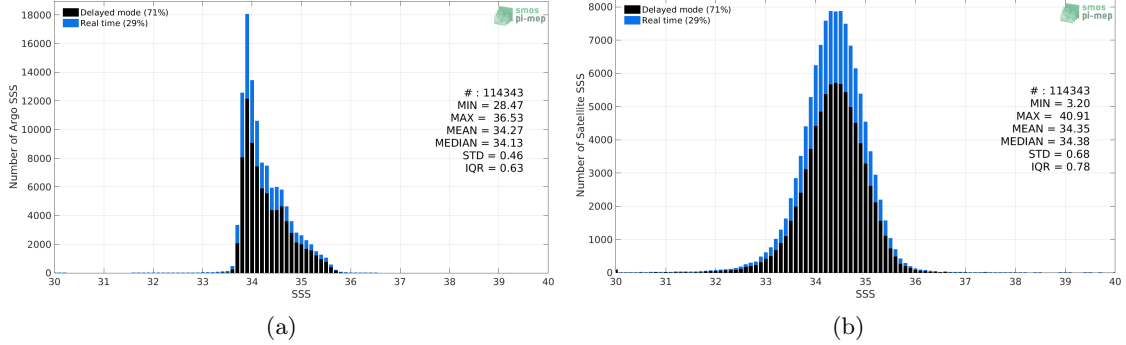
Figure 2: Histograms of SSS from Argo (a) and SMAP SSS L3 v5.0 - 8-Day running (JPL) (b) considering all match-up pairs per bins of 0.1 over the Roaring Forties and Furious Fifties Pi-MEP region and for the full satellite product period.
