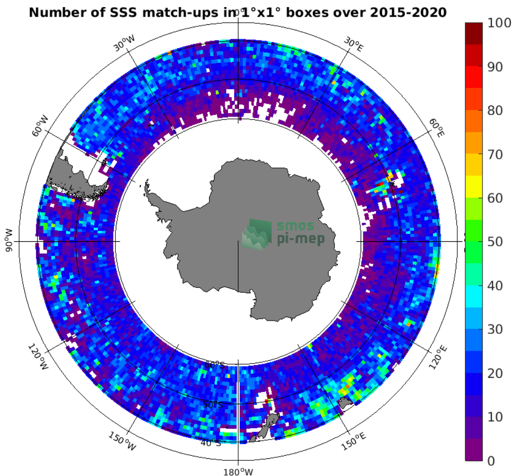
Figure 4: Number of SSS match-ups between Argo SSS and the SMAP SSS L3 v5.0 - 8-Day running (JPL) SSS product for the Roaring Forties and Furious Fifties Pi-MEP region over 1°x1° boxes and for the full satellite product period.
