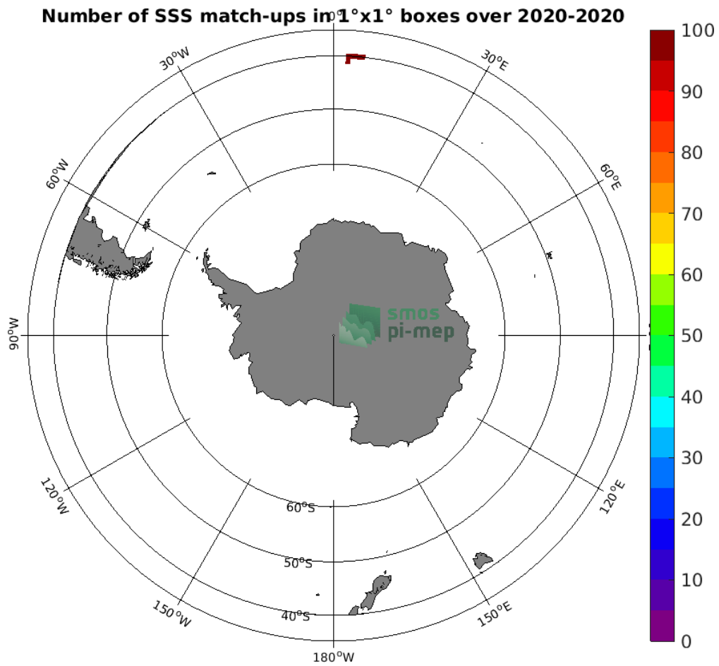
Figure 4: Number of SSS match-ups between TSG (SAMOS) SSS and the SMAP SSS L3 v5.0 - Monthly (JPL) SSS product for the Roaring Forties and Furious Fifties Pi-MEP region over 1°x1° boxes and for the full satellite product period.
