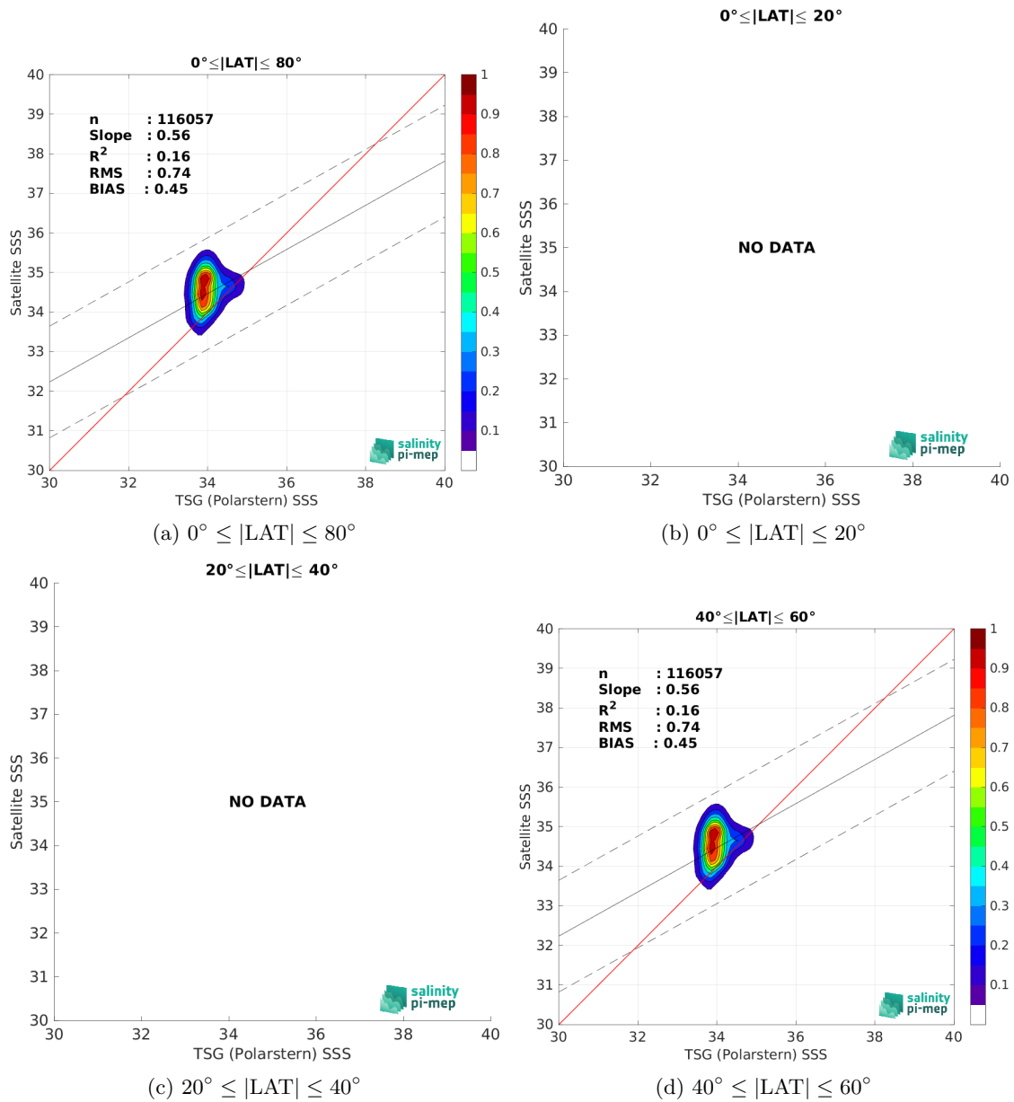
Figure 10: Contour maps of the concentration of SMAP SSS L3 v5.0 - Monthly (JPL) SSS (y-axis) versus TSG (Polarstern) SSS (x-axis) at match-up pairs for different latitude bands. For each plot, the red line shows x=y . The black thin and dashed lines indicate a linear fit through the data cloud and the \pm 95\% confidence levels, respectively. The number match-up pairs n , the slope and R^2 coefficient of the linear fit, the root mean square (RMS) and the mean bias between satellite and in situ data are indicated for each latitude band in each plots.
