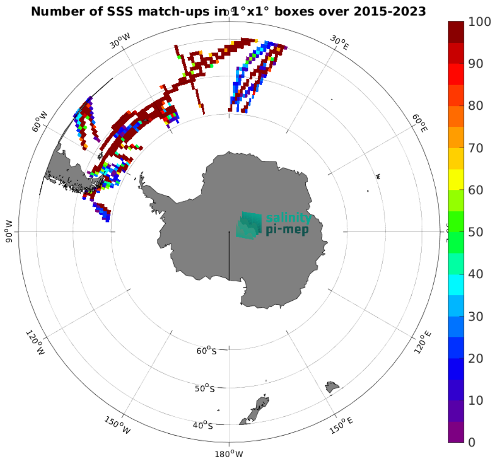
Figure 5: Number of SSS match-ups between TSG (Polarstern) SSS and the SMAP SSS L3 v5.0 - Monthly (JPL) SSS product for the Roaring Forties and Furious Fifties Pi-MEP region over 1^\circ \times 1^\circ boxes and for the full satellite product period.
