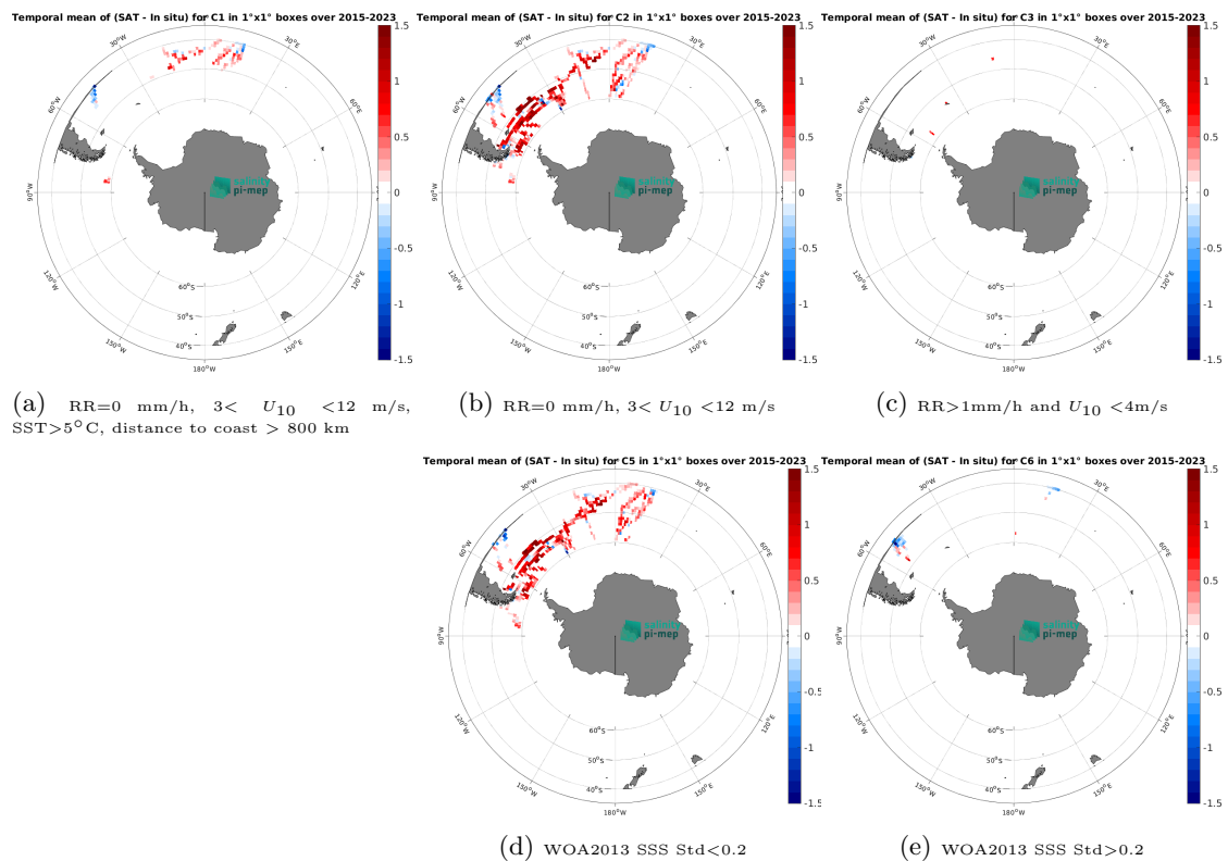
Figure 14: Temporal mean gridded over spatial boxes of size 1^\circ \times 1^\circ of \Delta SSS (SMAP SSS L3 v5.0 - Monthly (JPL) - TSG (Polarstern)) for 5 different subdatasets corresponding to:RR=0 mm/h, 3 < U_{10} < 12 m/s, SST>5°C, distance to coast > 800 km (a), RR=0 mm/h, 3 < U_{10} < 12 m/s (b), RR>1mm/h and U_{10} < 4 m/s (c), WOA2013 SSS Std<0.2 (d), WOA2013 SSS Std>0.2 (e).
