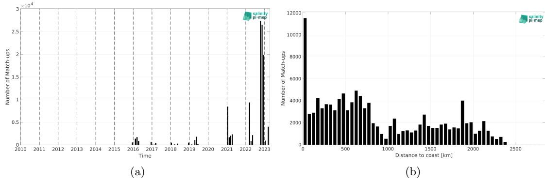
Figure 2: Number of match-ups between TSG (Polarstern) and SMAP SSS L3 v5.0 - Monthly (JPL) SSS as a function of time (a) and as function of the distance to coast (b) over the Roaring Forties and Furious Fifties Pi-MEP region and for the full satellite product period.
