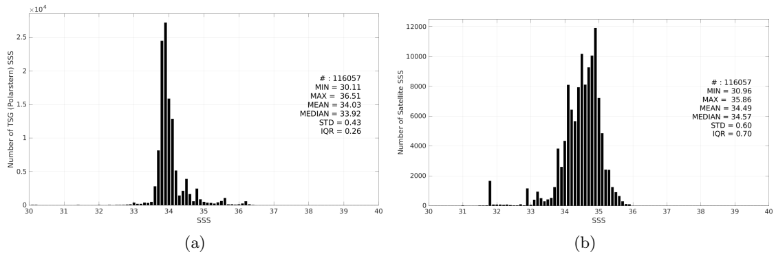
Figure 3: Histograms of SSS from TSG (Polarstern) (a) and SMAP SSS L3 v5.0 - Monthly (JPL) (b) considering all match-up pairs per bins of 0.1 over the Roaring Forties and Furious Fifties Pi-MEP region and for the full satellite product period.
